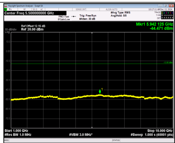
5-5-10MHz-10MHz-16QAM-16QAM-20450-20549-50RB#0- 50RB#0-1000~10000MHz-PASS
