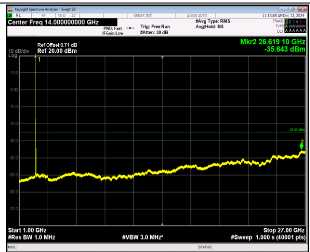
7-7-10MHz-20MHz-16QAM-16QAM-20805-20949-1RB#0-0 RB#0-1000~27000MHz-PASS
