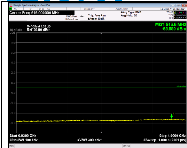
7-7-10MHz-20MHz-16QAM-16QAM-21006-21150-1RB#0 -0RB#0-30~1000MHz-PASS
