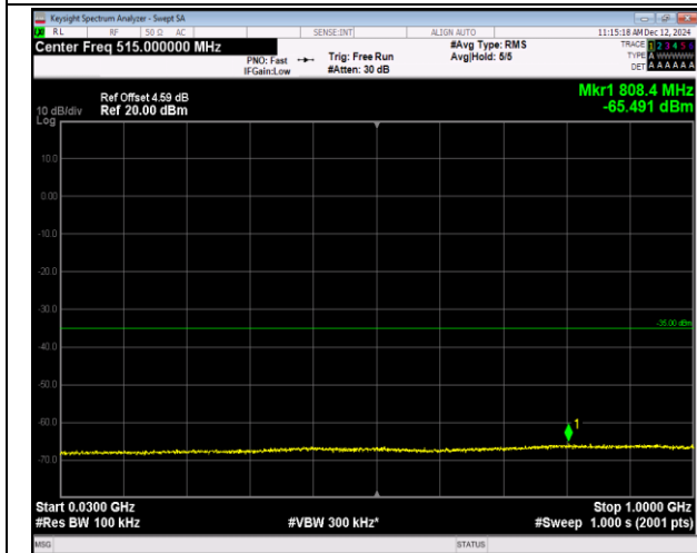
7-7-10MHz-20MHz-16QAM-16QAM-20805-20949-1RB#0 -1RB#99-30~1000MHz-PASS
