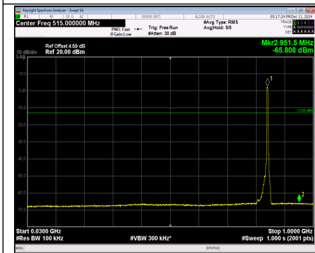
5-5-5MHz-3MHz-QPSK-QPSK-20595-20634-25RB#0-15 RB#0-30~1000MHz-PASS
