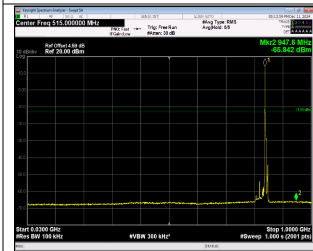
5-5-5MHz-3MHz-QPSK-QPSK-20595-20634-1RB#0-0RB#0-30~1000MHz-PASS
