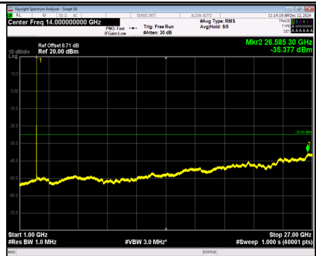
7-7-10MHz-20MHz-16QAM-16QAM-20805-20949-1RB#49- 0RB#0-1000~27000MHz-PASS
