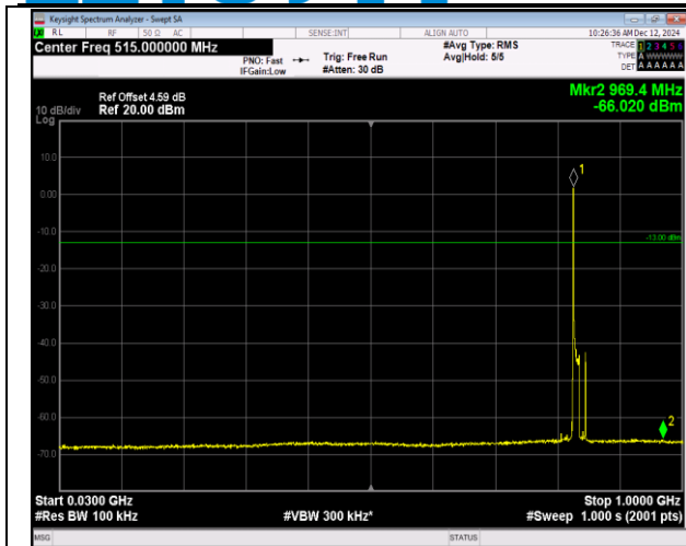
5-5-10MHz-10MHz-16QAM-16QAM-20501-20600-1RB#0 -1RB#49-30~1000MHz-PASS
