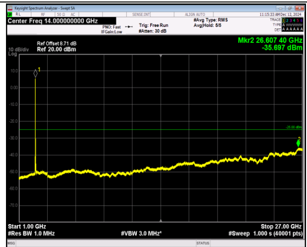
7-7-10MHz-20MHz-16QAM-16QAM-20805-20949-1RB#0-1 RB#99-1000~27000MHz-PASS
