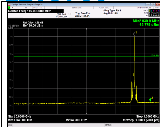
5-5-10MHz-10MHz-16QAM-16QAM-20450-20549-1RB#4 9-0RB#0-30~1000MHz-PASS
