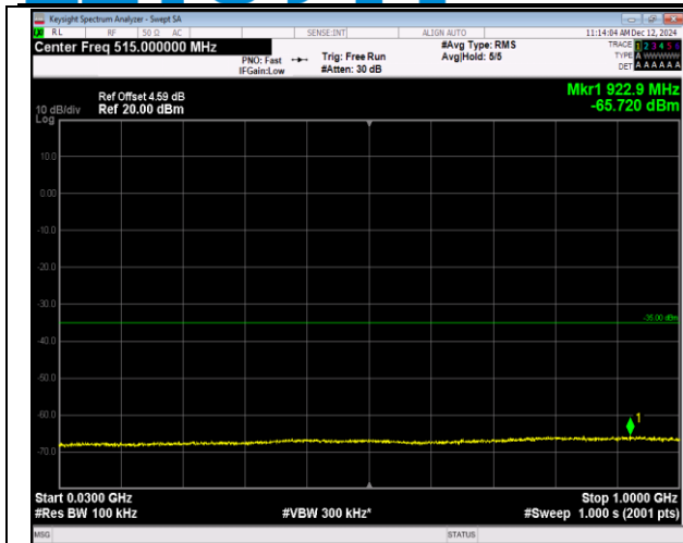
7-7-10MHz-20MHz-16QAM-16QAM-20805-20949-1RB#4 9-0RB#0-30~1000MHz-PASS
