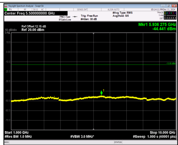
5-5-5MHz-3MHz-QPSK-QPSK-20595-20634-1RB#0-0RB#0-1000~10000MHz-PASS
