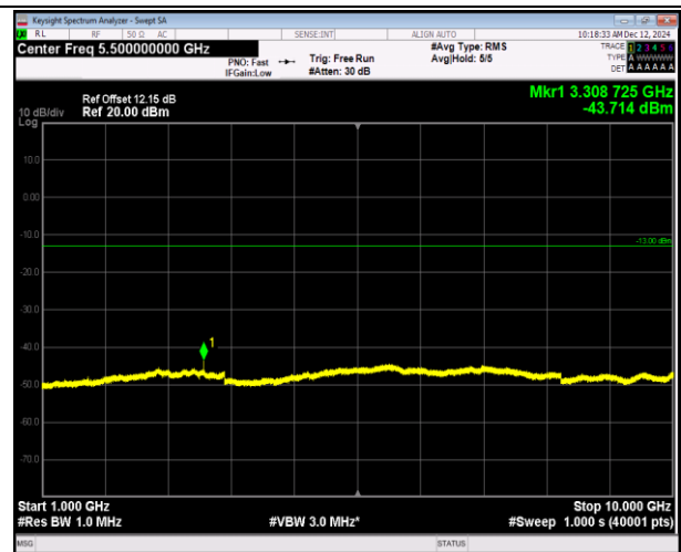
5-5-10MHz-10MHz-QPSK-QPSK-20476-20575-1RB#0-0RB #0-1000~10000MHz-PASS
