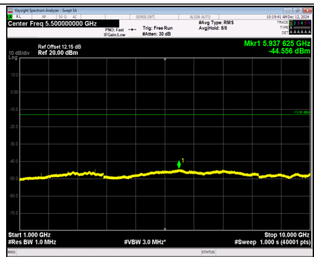
5-5-10MHz-10MHz-QPSK-QPSK-20476-20575-1RB#49-0R B#0-1000~10000MHz-PASS
