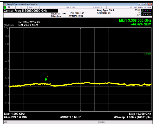
5-5-10MHz-10MHz-16QAM-16QAM-20476-20575-1RB#0-0 RB#0-1000~10000MHz-PASS
