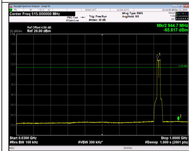
5-5-10MHz-10MHz-16QAM-16QAM-20450-20549-50RB#- 0-50RB#0-30~1000MHz-PASS
