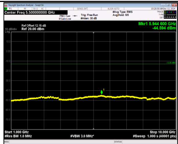
5-5-10MHz-10MHz-QPSK-QPSK-20476-20575-1RB#0-1RB #49-1000~10000MHz-PASS
