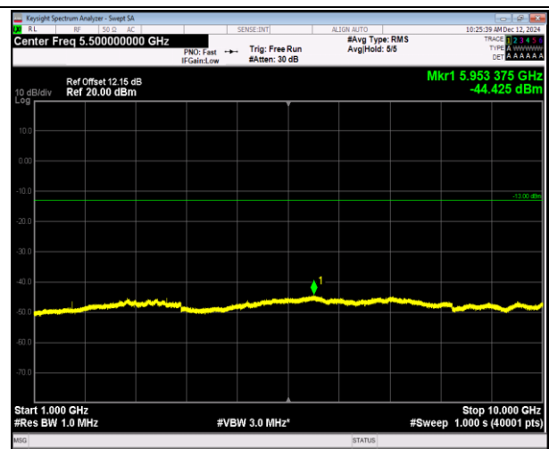
5-5-10MHz-10MHz-16QAM-16QAM-20501-20600-1RB#49- 0RB#0-1000~10000MHz-PASS
