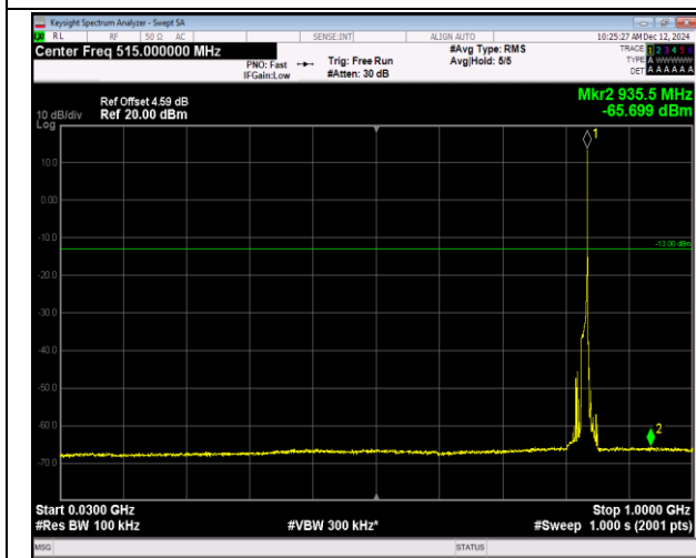
5-5-10MHz-10MHz-16QAM-16QAM-20501-20600-1RB#4 9-0RB#0-30~1000MHz-PASS
