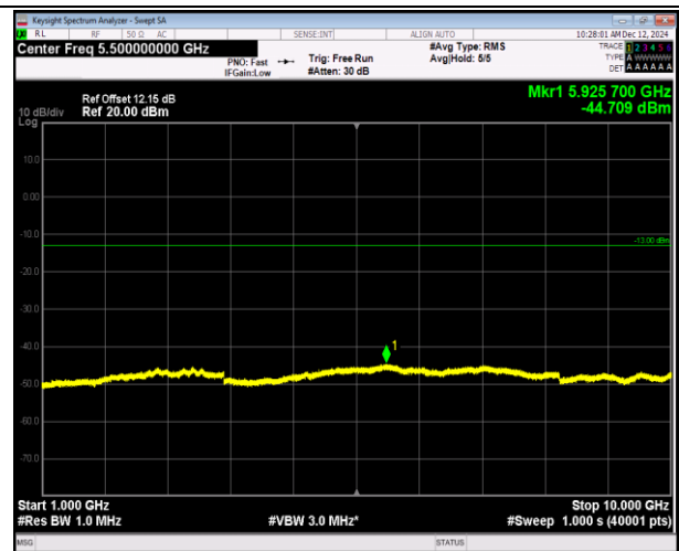
5-5-10MHz-10MHz-16QAM-16QAM-20501-20600-50RB#0- 50RB#0-1000~10000MHz-PASS
