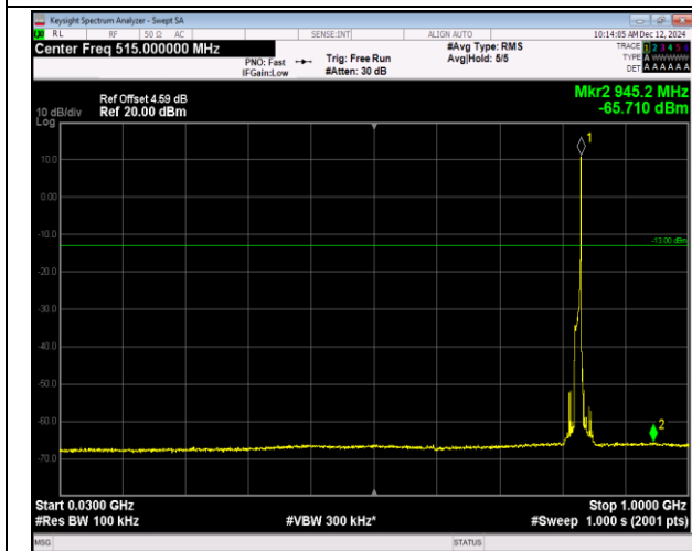
5-5-10MHz-10MHz-QPSK-QPSK-20450-20549-1RB#49-0 RB#0-30~1000MHz-PASS
