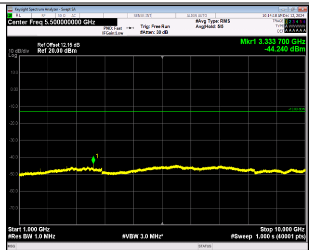
5-5-10MHz-10MHz-QPSK-QPSK-20450-20549-1RB#49-0R B#0-1000~10000MHz-PASS
