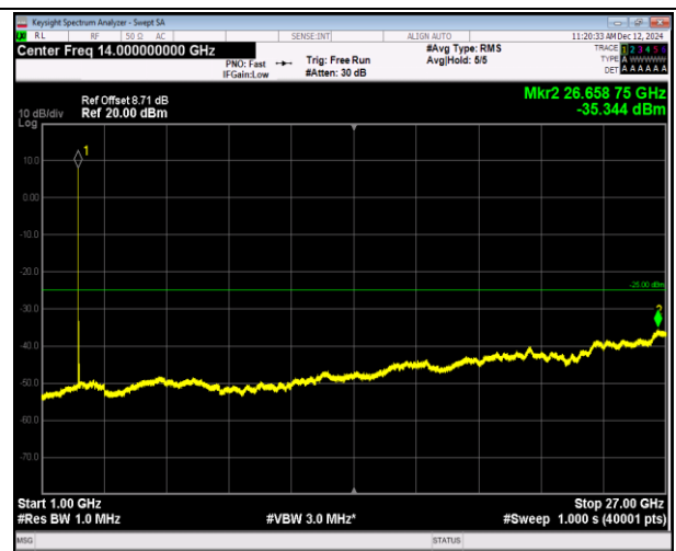
7-7-10MHz-20MHz-16QAM-16QAM-21006-21150-1RB#0-1 RB#99-1000~27000MHz-PASS
