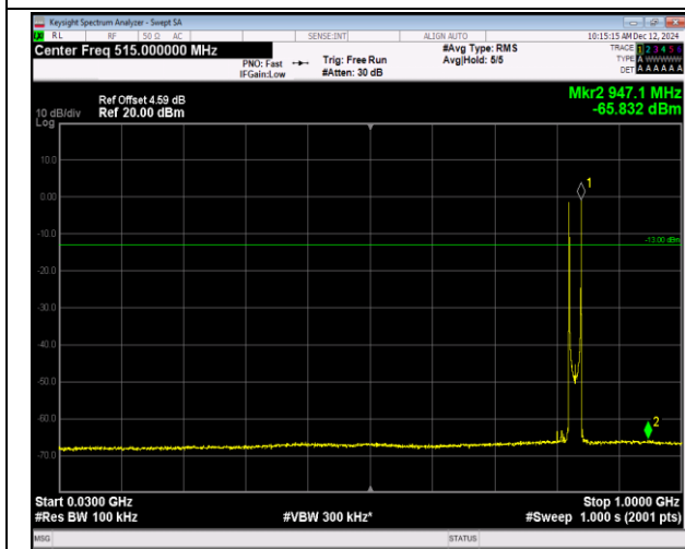
5-5-10MHz-10MHz-QPSK-QPSK-20450-20549-1RB#0-1 RB#49-30~1000MHz-PASS
