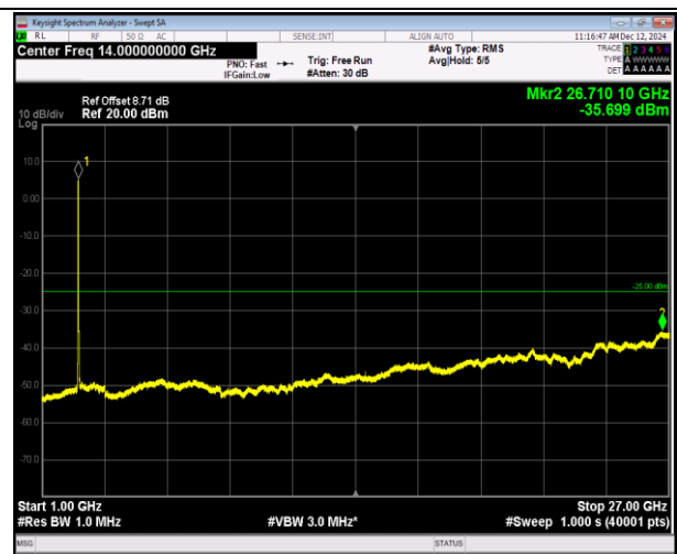
7-7-10MHz-20MHz-16QAM-16QAM-20805-20949-50RB#0- 100RB#0-1000~27000MHz-PASS
