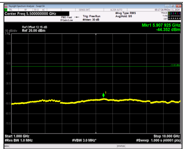
5-5-5MHz-3MHz-QPSK-QPSK-20595-20634-25RB#0-15RB #0-1000~10000MHz-PASS
