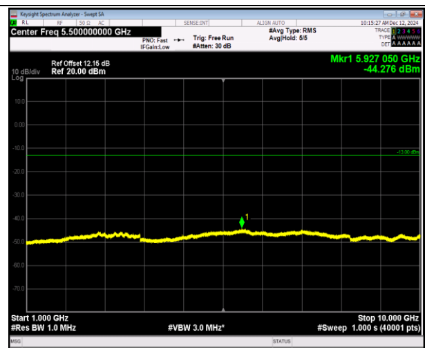
5-5-10MHz-10MHz-QPSK-QPSK-20450-20549-1RB#0-1RB #49-1000~10000MHz-PASS
