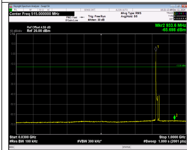
5-5-10MHz-10MHz-16QAM-16QAM-20476-20575-1RB#0 -1RB#49-30~1000MHz-PASS
