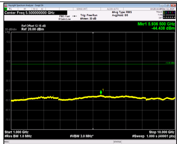
5-5-10MHz-10MHz-16QAM-16QAM-20476-20575-1RB#49- 0RB#0-1000~10000MHz-PASS
