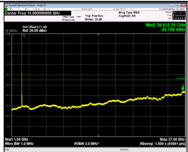
7-7-10MHz-20MHz-16QAM-16QAM-21006-21150-1RB#0-0 RB#0-1000~27000MHz-PASS
