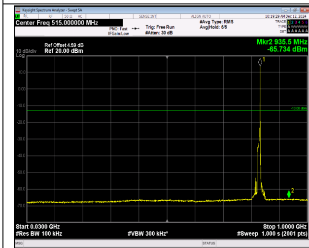
5-5-10MHz-10MHz-QPSK-QPSK-20476-20575-1RB#49-0 RB#0-30~1000MHz-PASS
