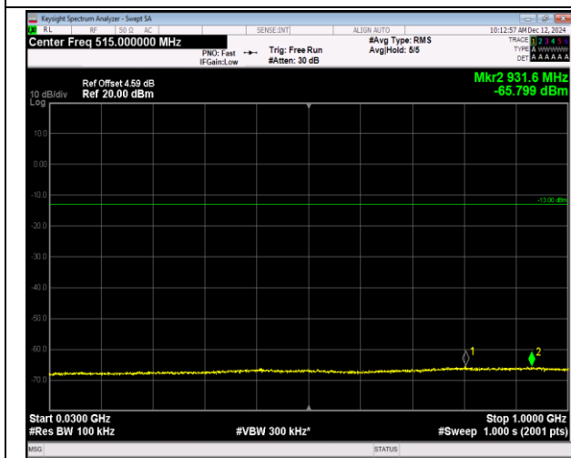
5-5-10MHz-10MHz-16QAM-16QAM-20450-20549-1RB#0 -ORB#0-30~1000MHz-PASS
