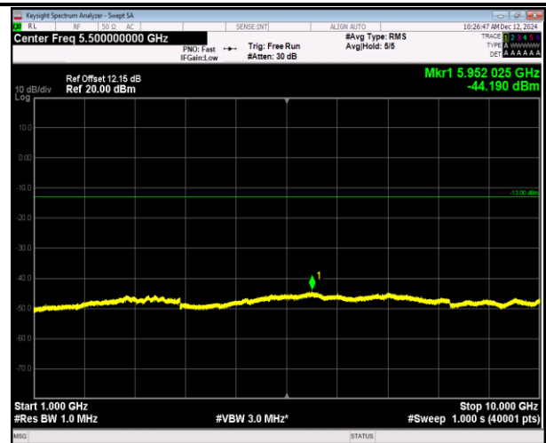
5-5-10MHz-10MHz-16QAM-16QAM-20501-20600-1RB#0-1 RB#49-1000~10000MHz-PASS
