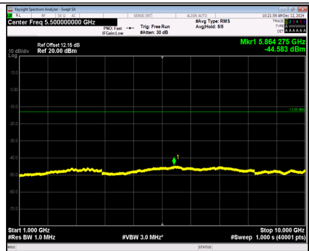
5-5-10MHz-10MHz-QPSK-QPSK-20476-20575-50RB#0-50 RB#0-1000~10000MHz-PASS
