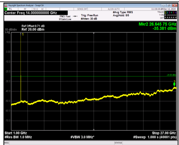
7-7-10MHz-20MHz-16QAM-16QAM-21006-21150-1RB#49- 0RB#0-1000~27000MHz-PASS
