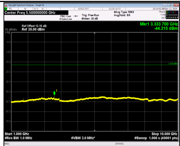
5-5-10MHz-10MHz-16QAM-16QAM-20450-20549-1RB#49- 0RB#0-1000~10000MHz-PASS
