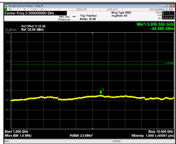
5-5-10MHz-10MHz-16QAM-16QAM-20476-20575-1RB#0-1 RB#49-1000~10000MHz-PASS
