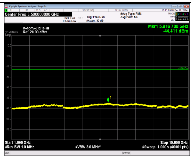
5-5-10MHz-10MHz-16QAM-16QAM-20450-20549-1RB#0-0 RB#0-1000~10000MHz-PASS
