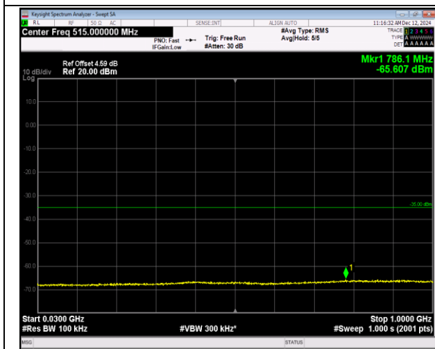
7-7-10MHz-20MHz-16QAM-16QAM-20805-20949-50RB#- 0-100RB#0-30~1000MHz-PASS
