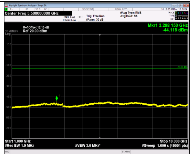
5-5-10MHz-10MHz-QPSK-QPSK-20450-20549-1RB#0-0RB #0-1000~10000MHz-PASS
