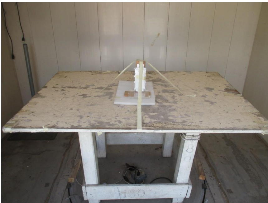
Figure 1 EUT Configuration for Radiated Emission Test
