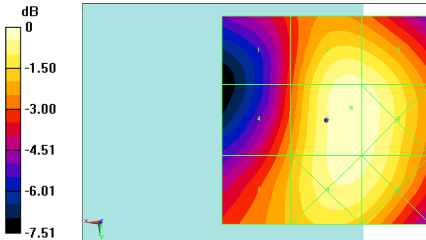
Fig B.2 HAC RF E-Field GSM 1900 Middle
