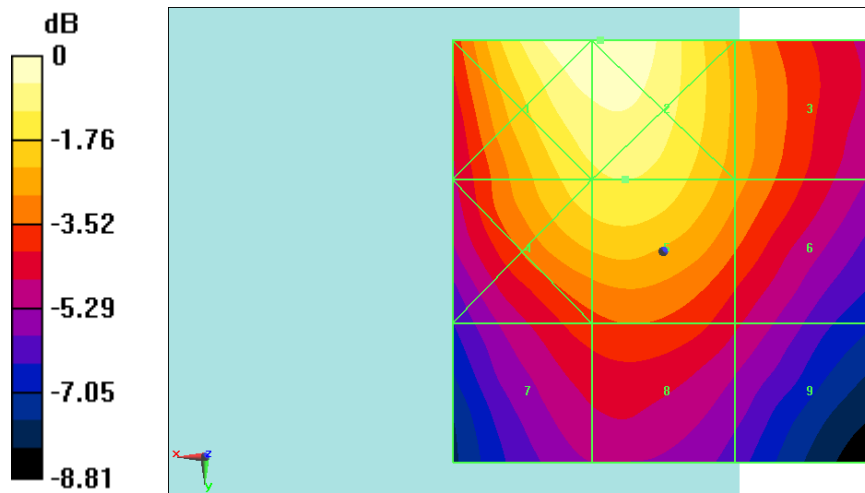
Fig B.3 HAC RF E-Field LTE Band41 QPSK CH40620
