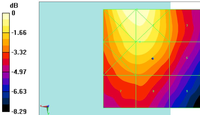
Fig B.4 HAC RF E-Field LTE Band41 QPSK CH40620
