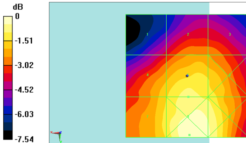
Fig B.5 HAC RF E-Field WiFi2.4G 11b
