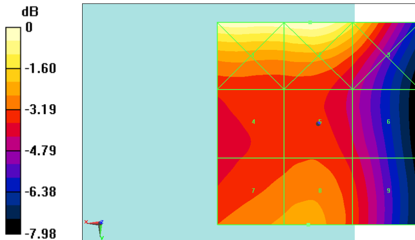
Fig B.1 HAC RF E-Field GSM 850 Low
