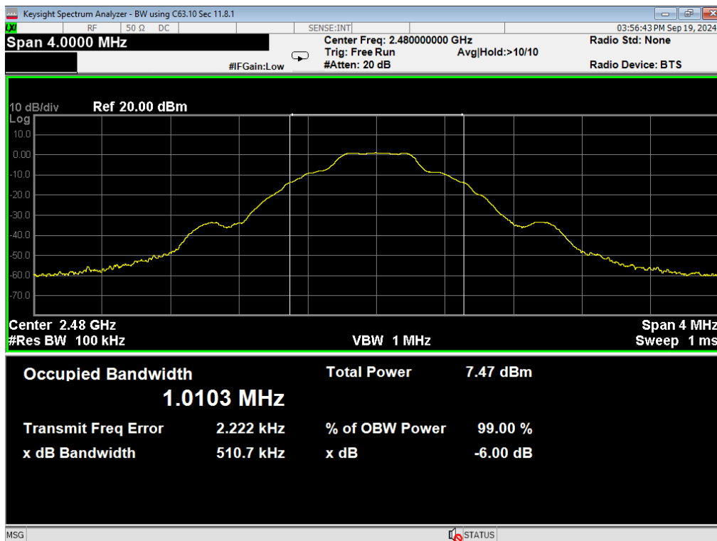
09, 6dB Bandwidth, ANT GFSK, High
