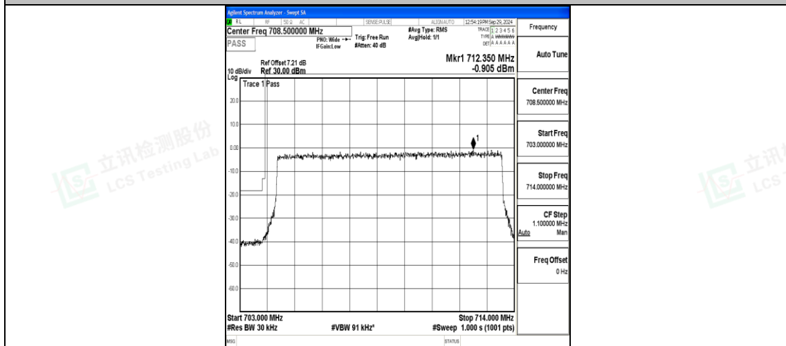
Band17_10MHz_16QAM_23780_50RB#0
