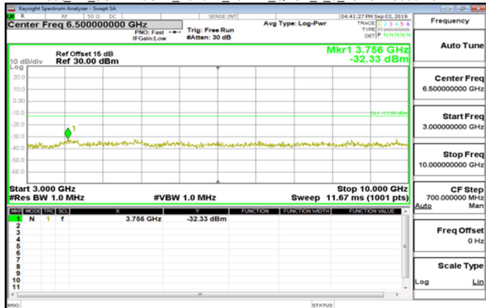
Cat M1_3GHz~10GHz_Band12_10MHz_QPSK_1_0_LowCH23060-704
