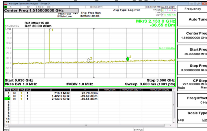
Cat M1_30MHz~3GHz_Band12_10MHz_QPSK_1_0_HighCH23130-711
