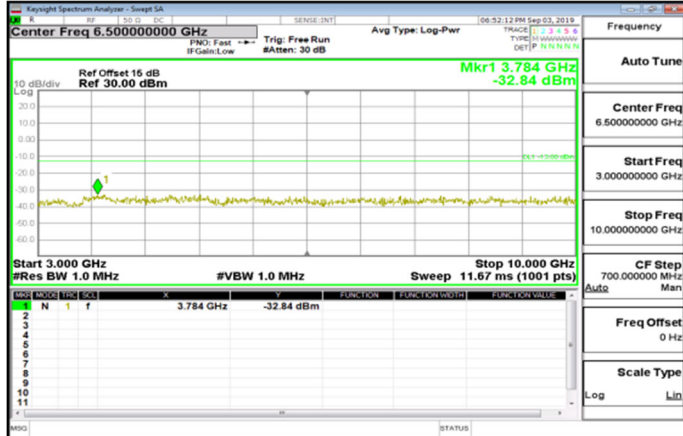
Cat_M1_3GHz~10GHz_Band13_5MHz_QPSK_1_0_LowCH23205-779.5
