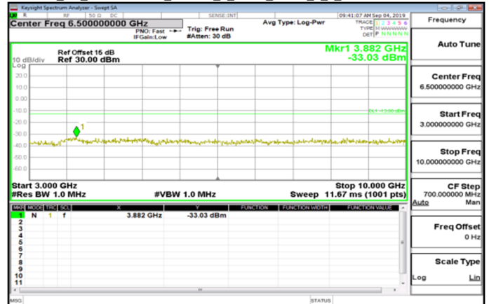
Cat_M1_3GHz~10GHz_Band26_1_4MHz_QPSK_1_0_LowCH26797-824.7
