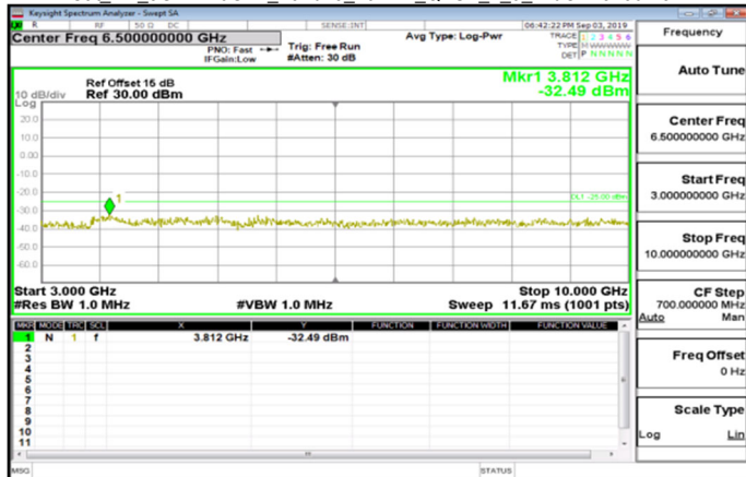
Cat_M1_3GHz~10GHz_Band13_10MHz_QPSK_1_0_MidCH23230-782
