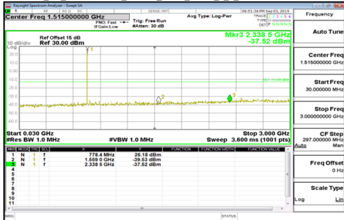
Cat_M1_30MHz~3GHz_Band13_5MHz_QPSK_1_0_LowCH23205-779.5
