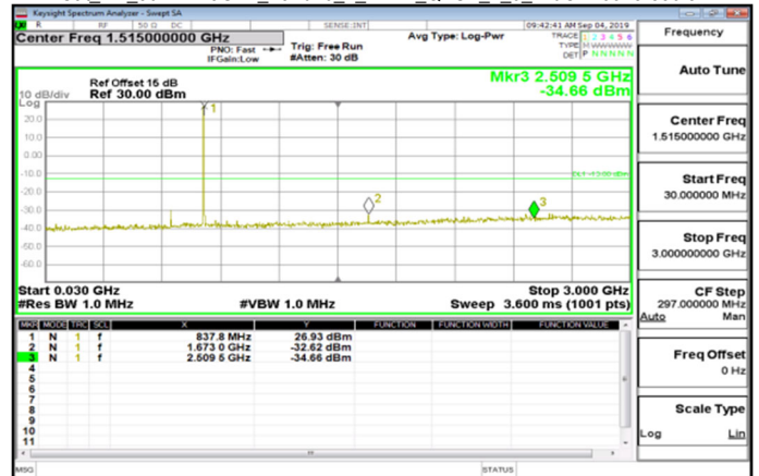
Cat_M1_30MHz~3GHz_Band26_1_4MHz_QPSK_1_0_MidCH26915-836.5
