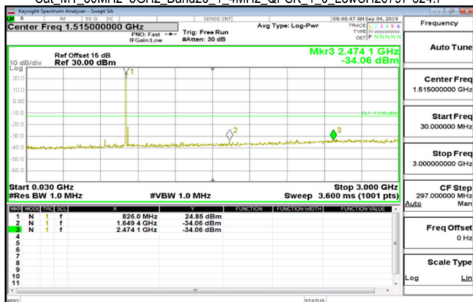
Cat_M1_30MHz~3GHz_Band26_1_4MHz_QPSK_1_0_LowCH26797-824.7
