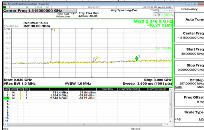
Cat_M1_30MHz~3GHz_Band13_5MHz_QPSK_1_0_MidCH23230-782
