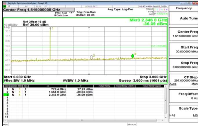
Cat_M1_30MHz~3GHz_Band13_10MHz_QPSK_1_0_MidCH23230-782
