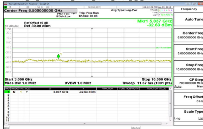
Cat M1_3GHz~10GHz_Band12_10MHz_QPSK_1_0_MidCH23095-707.5
