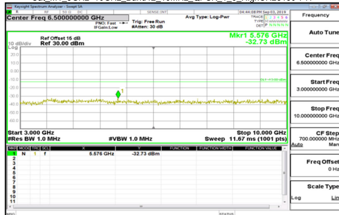
Cat M1_3GHz~10GHz_Band12_10MHz_QPSK_1_0_HighCH23130-711
