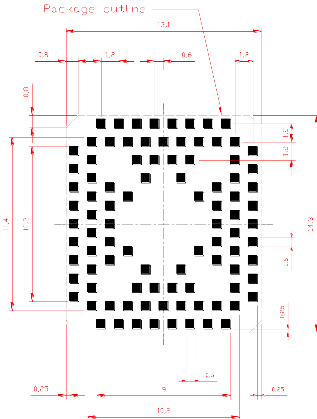
COPPER PATTERN (top view)
