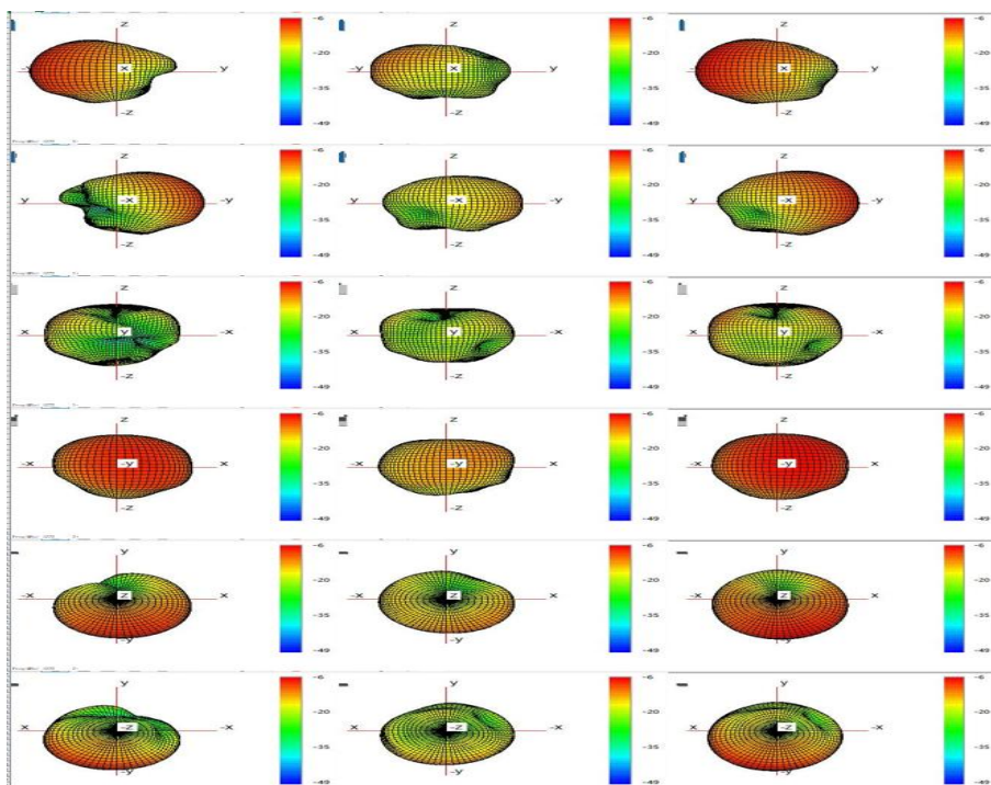
GPS L5 passive direction diagram/field pattern diagram
