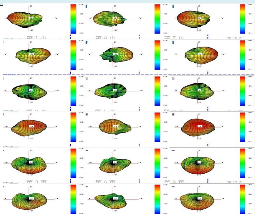
BT passive direction diagram/field pattern diagram
