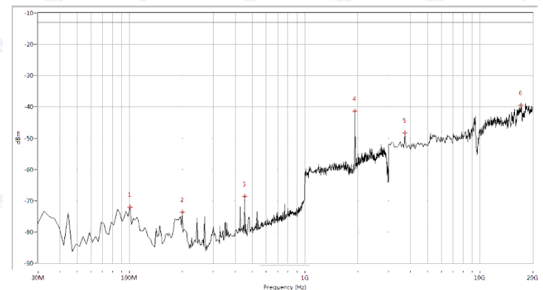
(Plot E6: WCDMA 850MHz Channel = 4233, Test Antenna Vertical)
