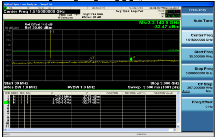
30MHz~3GHz_Band17_5MHz_QPSK_1_0_HighCH23825-713.5
