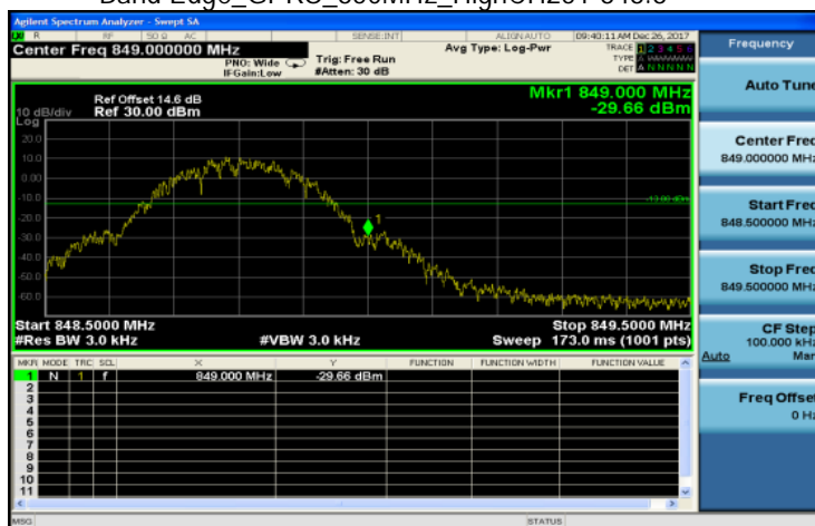
Band Edge_GPRS_850MHz_HighCH251-848.8
