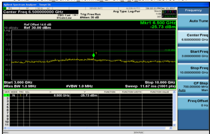
3GHz~10GHz_Band17_10MHz_QPSK_1_0_LowCH23780-709
