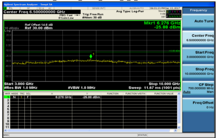
3GHz~10GHz_Band17_5MHz_QPSK_1_0_MidCH23790-710
