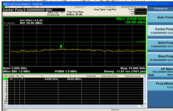
3GHz~10GHz_Band12_10MHz_QPSK_1_0_LowCH23060-704
