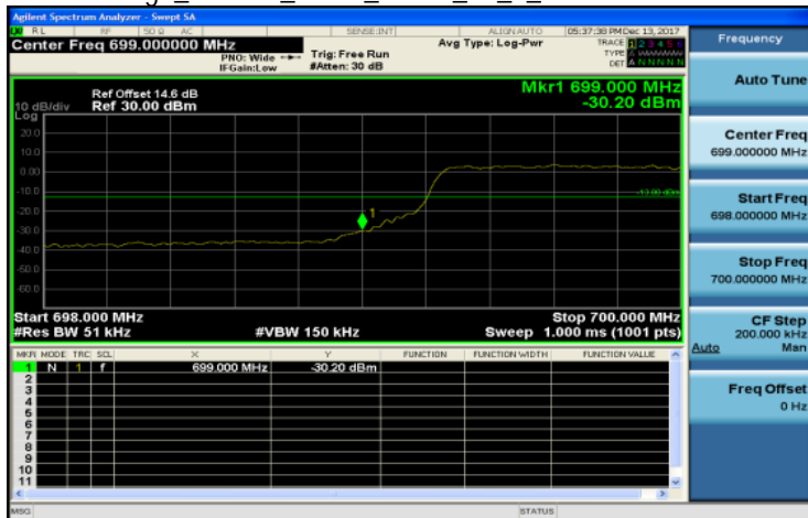
Band Edge_Band12_5MHz_QPSK_25_0_LowCH23035-701.5
