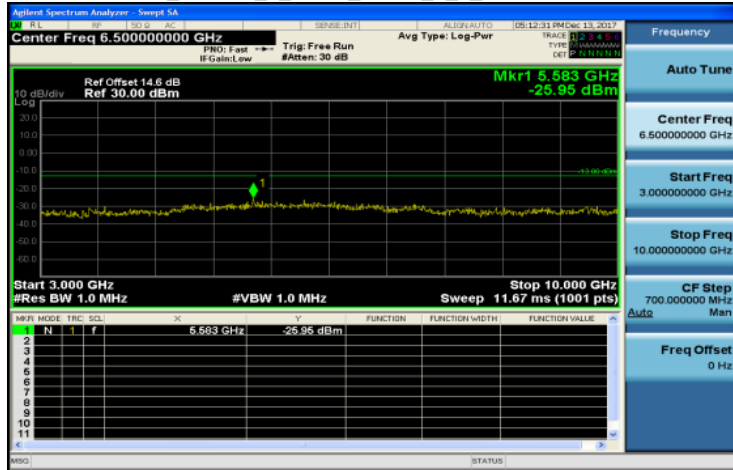
3GHz~10GHz_Band12_1_4MHz_QPSK_1_0_LowCH23017-699.7
