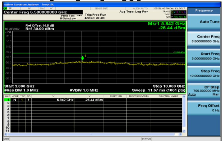
3GHz~10GHz_Band12_10MHz_QPSK_1_0_MidCH23095-707.5
