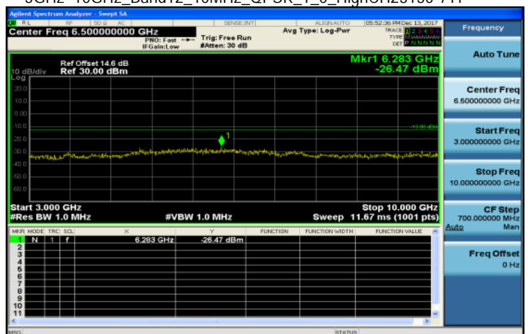
3GHz~10GHz_Band12_10MHz_QPSK_1_0_HighCH23130-711
