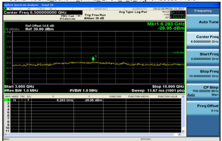
3GHz~10GHz_Band17_5MHz_QPSK_1_0_HighCH23825-713.5
