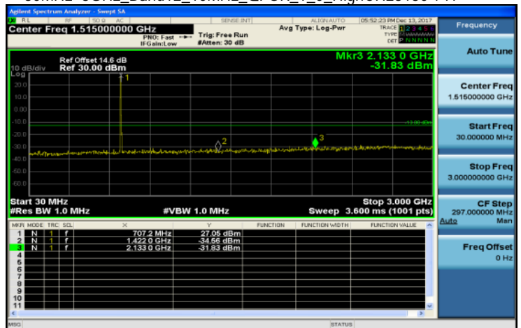
30MHz~3GHz_Band12_10MHz_QPSK_1_0_HighCH23130-711
