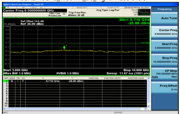
3GHz~10GHz_WCDMA_B5_HighCH4233-846.6
