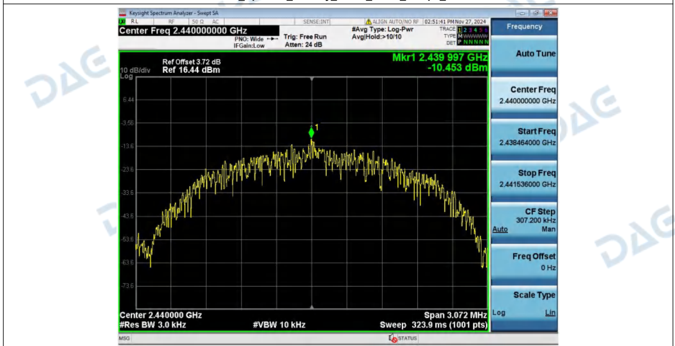
Power_Spectral_Density_NVNT_ANT1_2Mbps_2440
