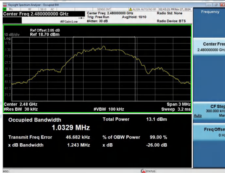
99%_Occupied_Bandwidth_NVNT_ANT1_1Mbps_2480
