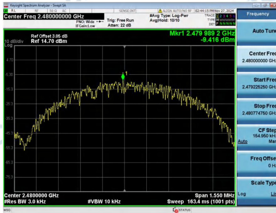
Power_Spectral_Density_NVNT_ANT1_1Mbps_2480
