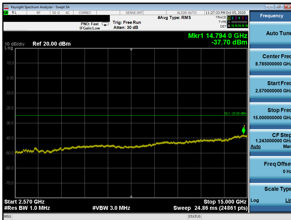
Plot 7-14. Conducted Spurious Plot (LTE Band 7 - 20MHz QPSK - RB Size 1, RB Offset 0 - Low Channel)
