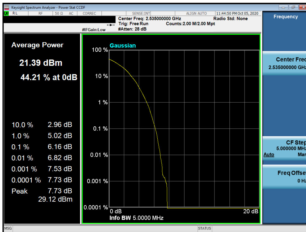
Plot 7-39. PAR Plot (LTE Band 7 - 5MHz 16-QAM - Full RB Configuration)
