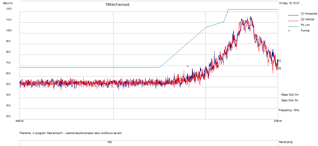
Figure 116: Low U-NII-3 band edge for 802.11a NoHT 6Mbps at Channel 149
