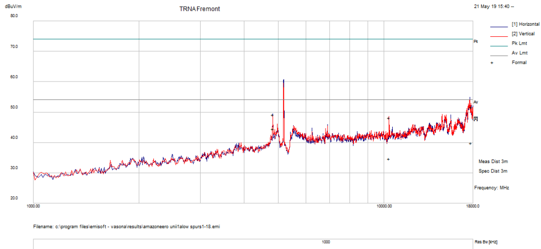
Figure 125: 1-18GHz 802.11a Mode Channel 36
