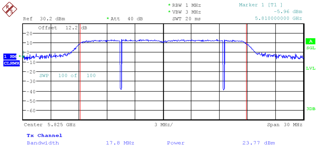
Figure 11: Output Power, Channel 165 802.11 HT20, Chain 0
