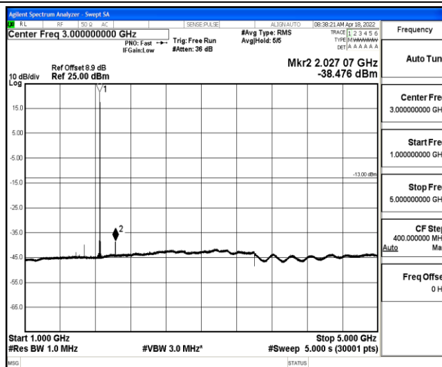
Band2-10MHz-QPSK-18650-1-0-Low-1000-5000--38.48-PASS
