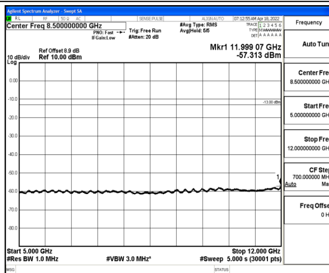
Band2-1.4MHz-QPSK-18900-1-0-Low-5000-12000--57.31-PASS
