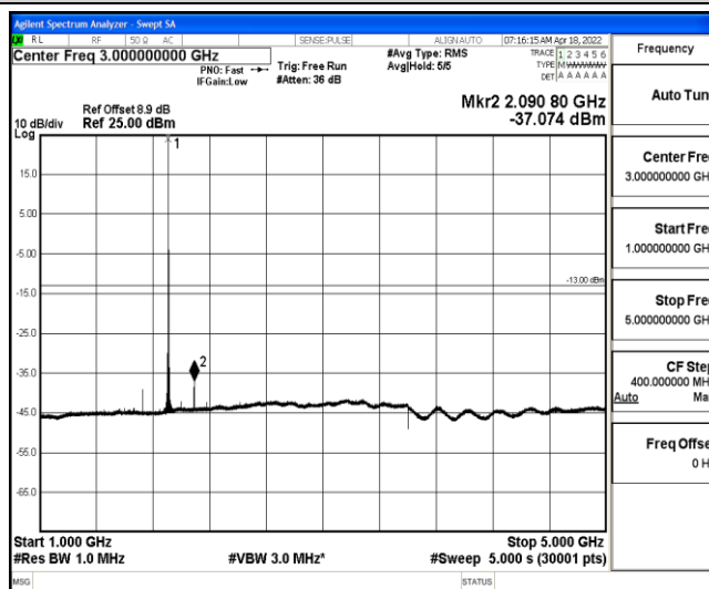
Band2-1.4MHz-QPSK-19193-1-0-High-1000-5000--37.07-PASS
