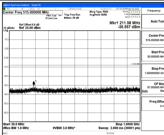
Band2-1.4MHz-QPSK-19193-1-0-High-30-1000--35.56-PASS
