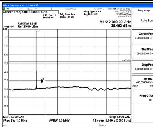
Band2-10MHz-QPSK-19150-1-0-High-1000-5000--38.49-PASS
