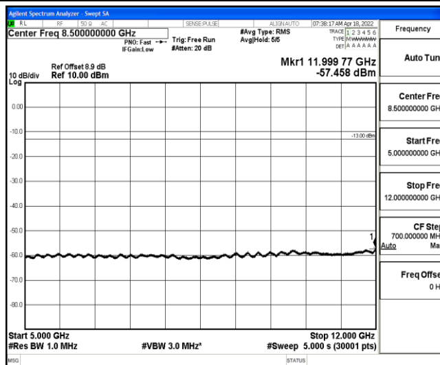
Band2-3MHz-QPSK-18615-1-0-Low-5000-12000--57.46-PASS
