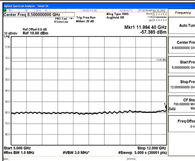
Band2-1.4MHz-16QAM-18607-1-0-Low-5000-12000--57.39-PASS
