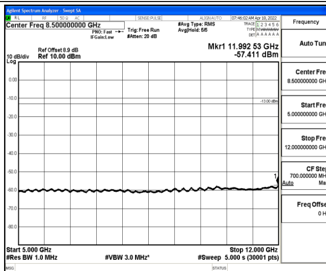
Band2-3MHz-QPSK-19185-1-0-High-5000-12000--57.41-PASS
