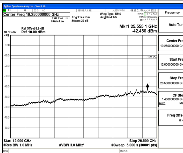
Band2-5MHz-16QAM-18625-1-0-Low-12000-26500--42.45-PASS
