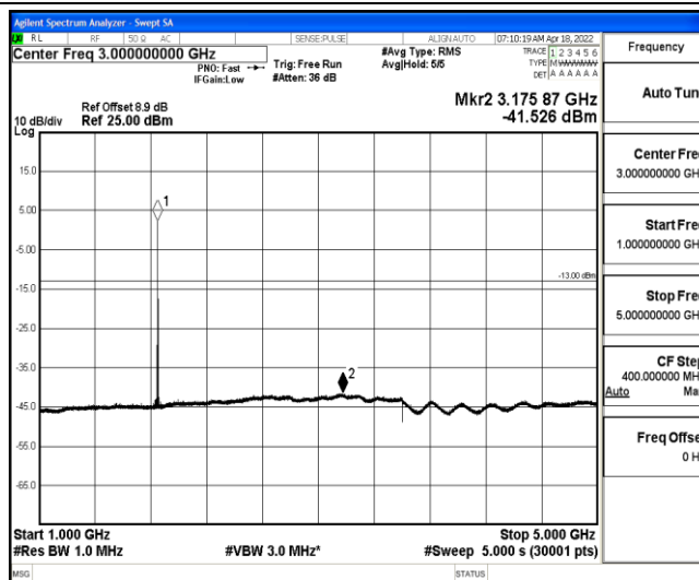
Band2-1.4MHz-16QAM-18607-1-0-Low-1000-5000--41.53-PASS
