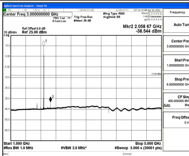
Band2-1.4MHz-16QAM-18900-1-0-Low-1000-5000--38.54-PASS
