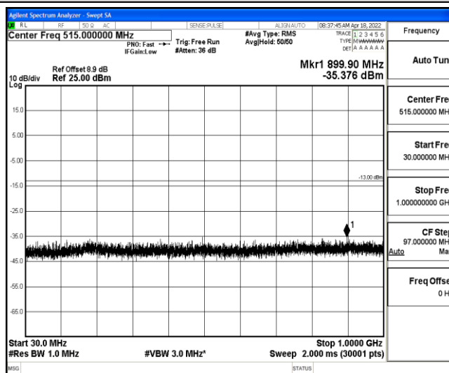
Band2-10MHz-QPSK-18650-1-0-Low-30-1000--35.38-PASS
