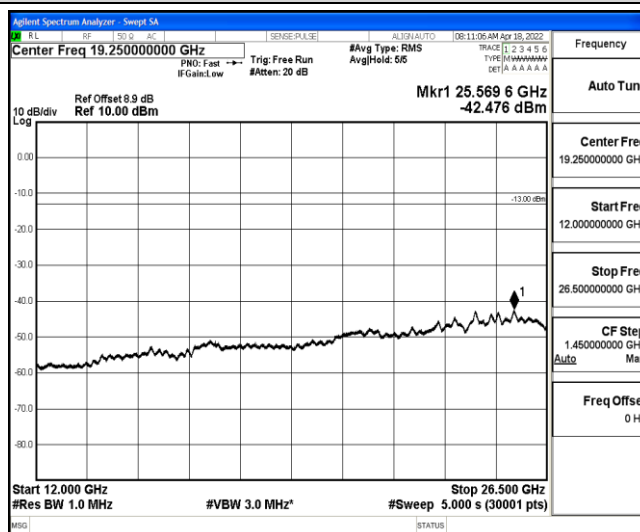
Band2-5MHz-QPSK-18625-1-0-Low-12000-26500--42.48-PASS
