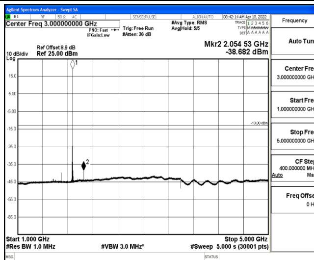
Band2-10MHz-QPSK-18900-1-0-Low-1000-5000--38.68-PASS
