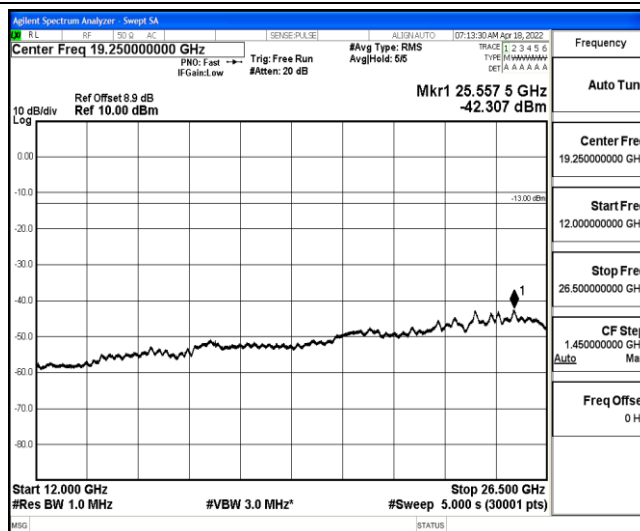
Band2-1.4MHz-QPSK-18900-1-0-Low-12000-26500--42.31-PASS
