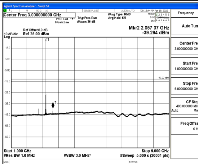
Band2-5MHz-16QAM-18900-1-0-Low-1000-5000--39.29-PASS
