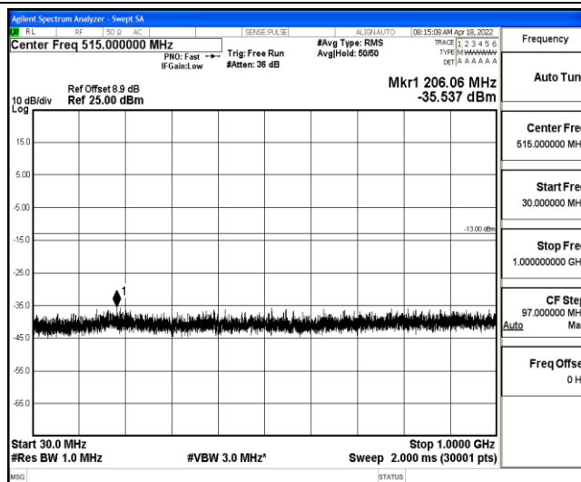
Band2-5MHz-16QAM-18900-1-0-Low-30-1000--35.54-PASS
