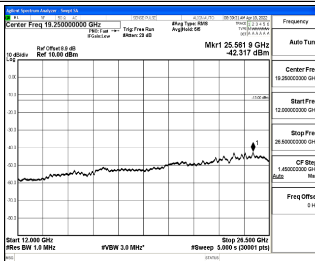
Band2-10MHz-QPSK-18650-1-0-Low-12000-26500--42.32-PASS
