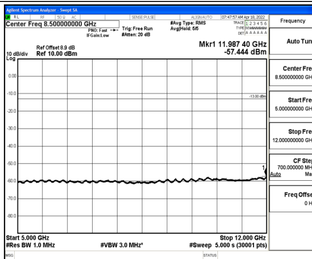
Band2-3MHz-16QAM-19185-1-0-High-5000-12000--57.44-PASS
