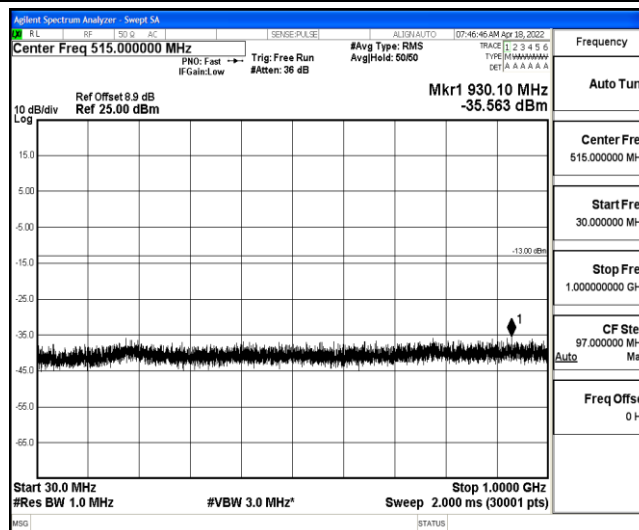
Band2-3MHz-16QAM-19185-1-0-High-30-1000--35.56-PASS
