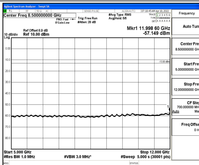
Band2-1.4MHz-16QAM-19193-1-0-High-5000-12000--57.15-PASS
