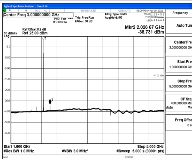
Band2-5MHz-QPSK-18625-1-0-Low-1000-5000--38.73-PASS
