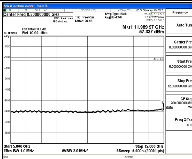
Band2-10MHz-QPSK-18650-1-0-Low-5000-12000--57.34-PASS
