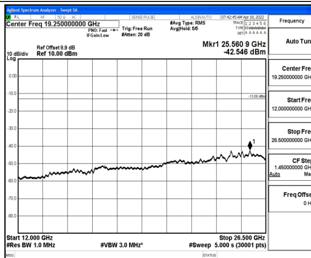
Band2-3MHz-QPSK-18900-1-0-Low-12000-26500--42.55-PASS
