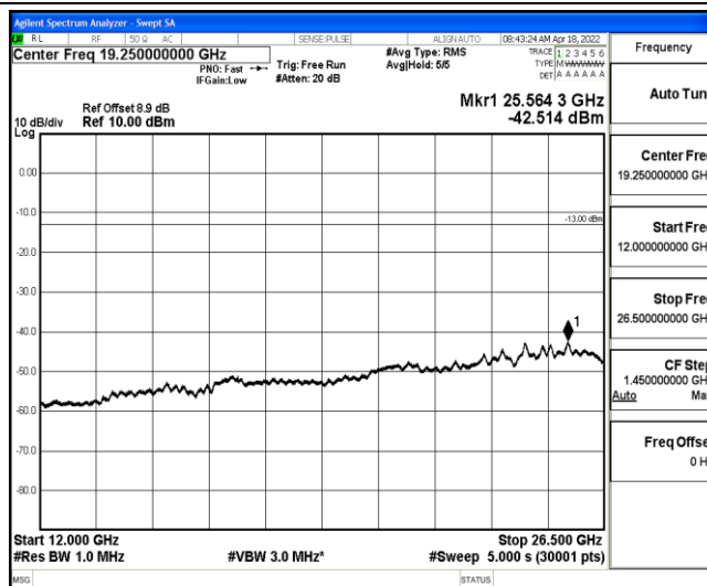
Band2-10MHz-QPSK-18900-1-0-Low-12000-26500--42.51-PASS
