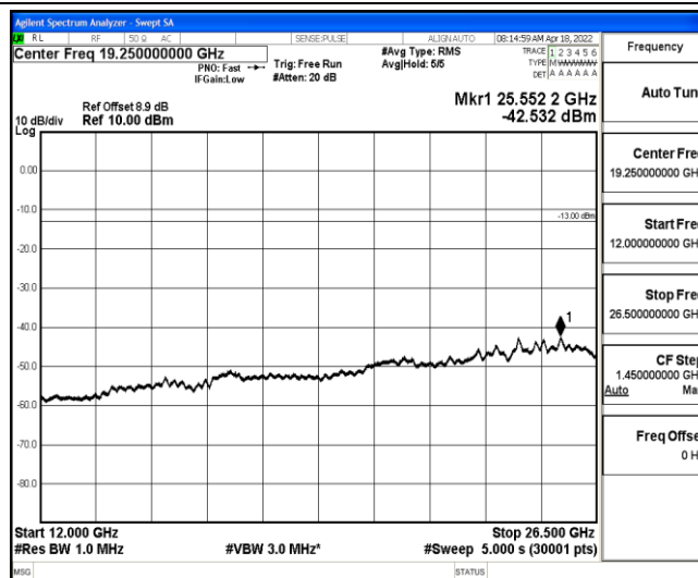
Band2-5MHz-QPSK-18900-1-0-Low-12000-26500--42.53-PASS
