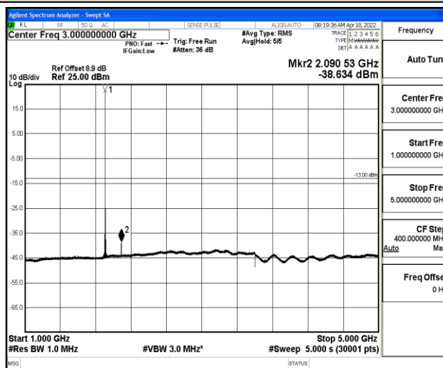
Band2-5MHz-16QAM-19175-1-0-High-1000-5000--38.63-PASS
