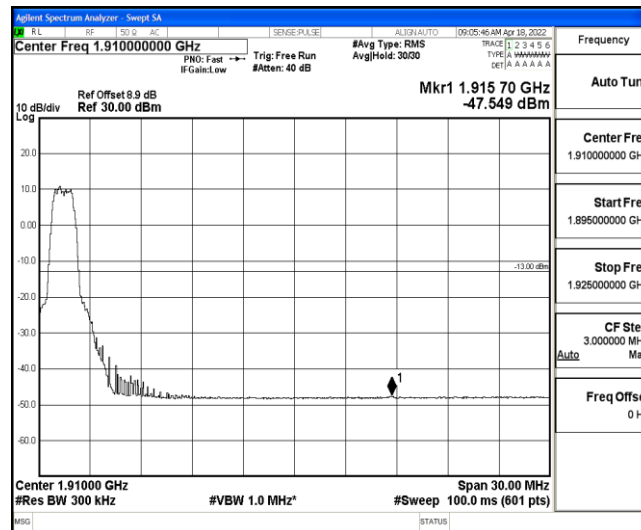
Band2-15MHz-16QAM-19125-6-0-Low--47.55-PASS
