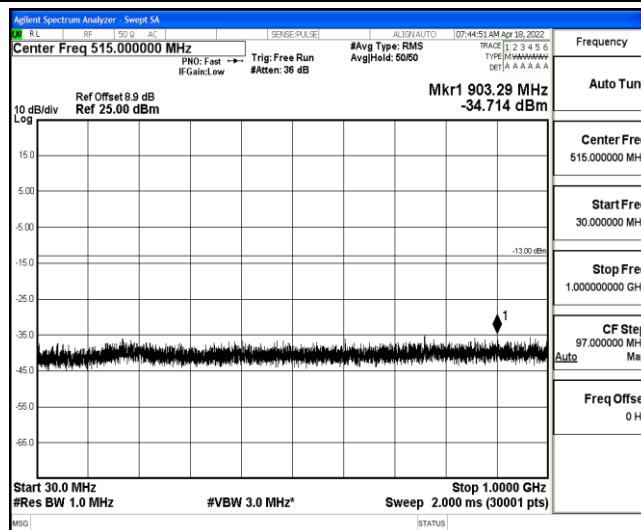
Band2-3MHz-QPSK-19185-1-0-High-30-1000--34.71-PASS
