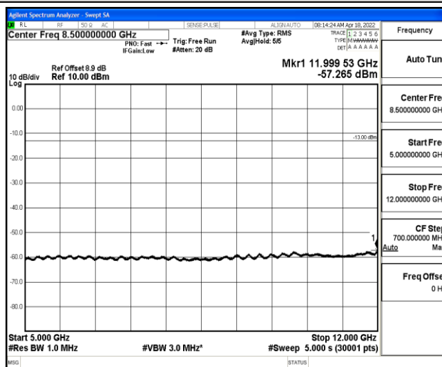
Band2-5MHz-QPSK-18900-1-0-Low-5000-12000--57.27-PASS
