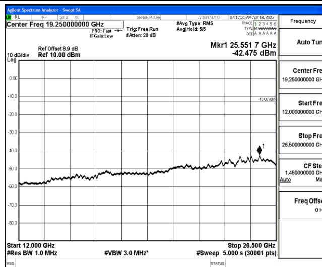
Band2-1.4MHz-QPSK-19193-1-0-High-12000-26500--42.48-PASS
