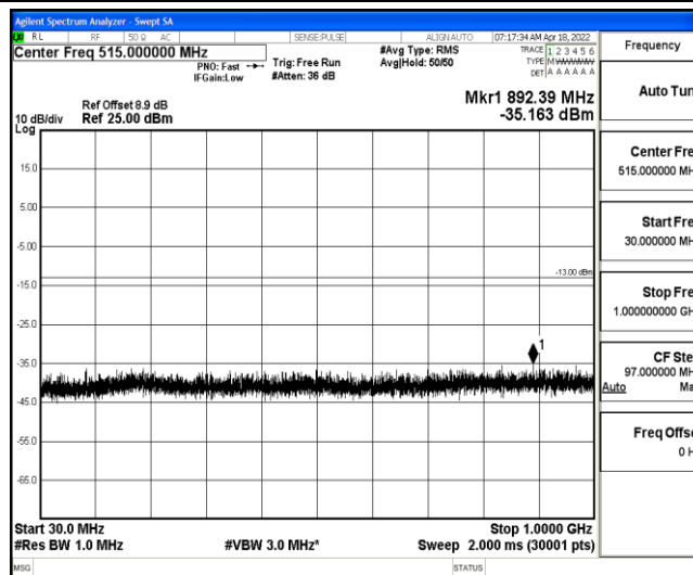
Band2-1.4MHz-16QAM-19193-1-0-High-30-1000--35.16-PASS
