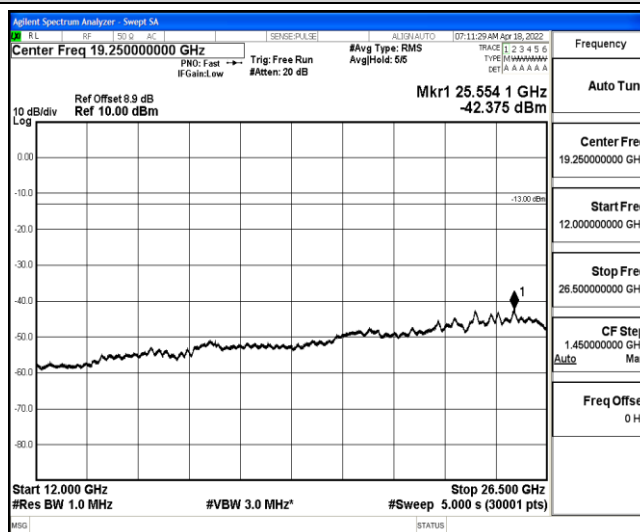
Band2-1.4MHz-16QAM-18607-1-0-Low-12000-26500--42.38-PASS
