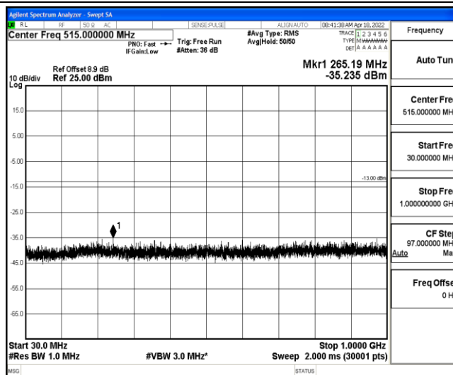
Band2-10MHz-QPSK-18900-1-0-Low-30-1000--35.24-PASS
