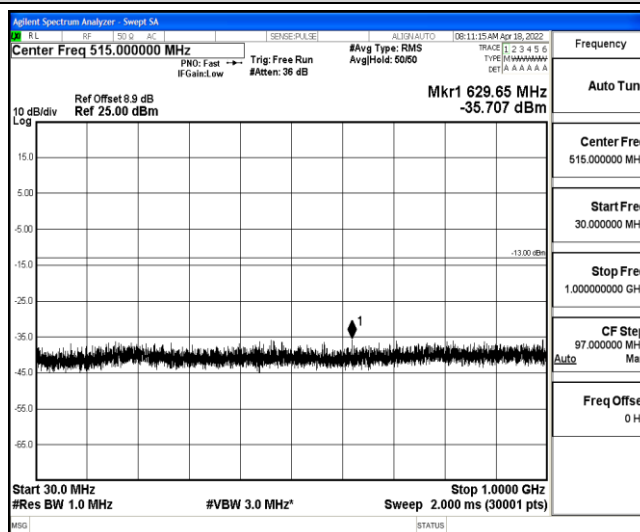
Band2-5MHz-16QAM-18625-1-0-Low-30-1000--35.71-PASS
