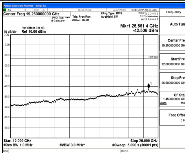
Band2-1.4MHz-16QAM-19193-1-0-High-12000-26500--42.51-PASS
