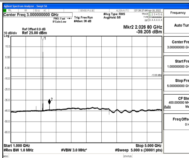
Band2-3MHz-16QAM-18615-1-0-Low-1000-5000--39.21-PASS
