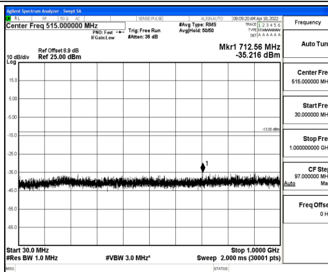
Band2-5MHz-QPSK-18625-1-0-Low-30-1000--35.22-PASS
