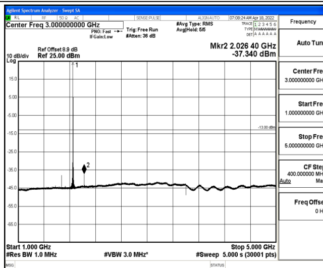
Band2-1.4MHz-QPSK-18607-1-0-Low-1000-5000--37.34-PASS
