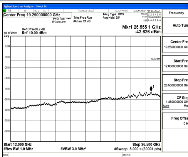
Band2-1.4MHz-QPSK-18607-1-0-Low-12000-26500--42.63-PASS
