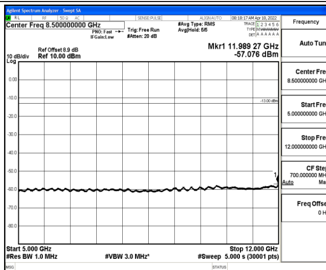
Band2-5MHz-QPSK-19175-1-0-High-5000-12000--57.08-PASS
