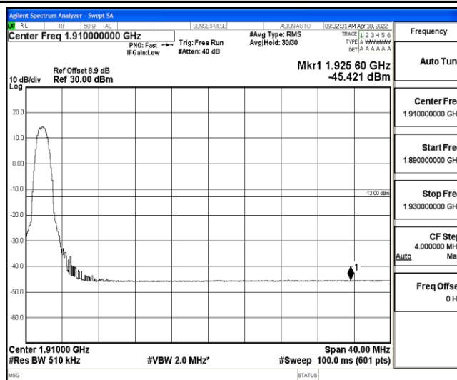
Band2-20MHz-16QAM-19100-6-0-Low--45.42-PASS
