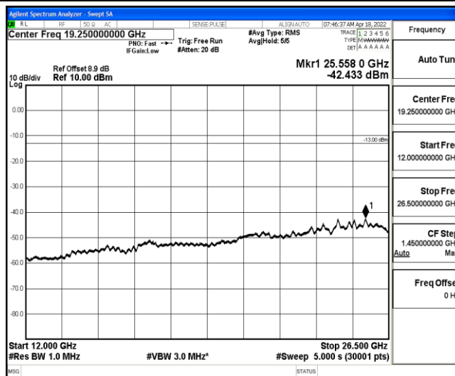
Band2-3MHz-QPSK-19185-1-0-High-12000-26500--42.43-PASS
