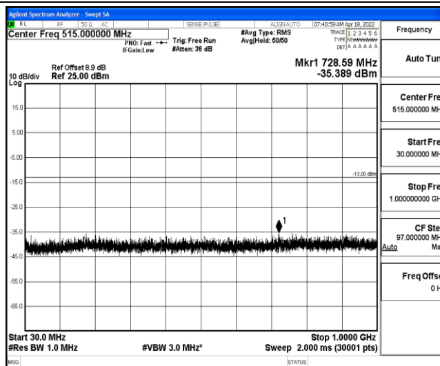
Band2-3MHz-QPSK-18900-1-0-Low-30-1000--35.39-PASS
