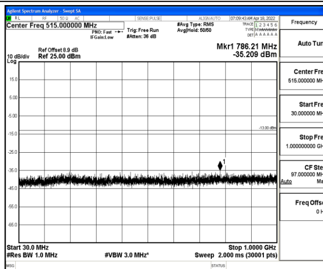
Band2-1.4MHz-16QAM-18607-1-0-Low-30-1000--35.21-PASS
