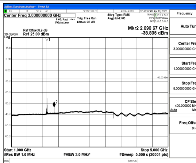
Band2-3MHz-16QAM-19185-1-0-High-1000-5000--38.81-PASS
