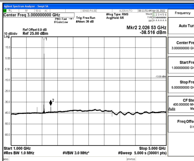
Band2-5MHz-16QAM-18625-1-0-Low-1000-5000--38.52-PASS
