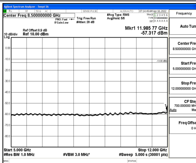
Band2-1.4MHz-16QAM-18900-1-0-Low-5000-12000--57.32-PASS
