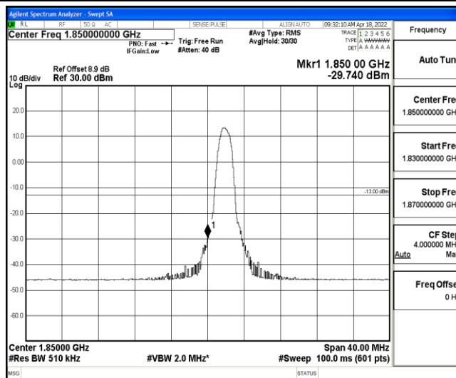
Band2-20MHz-16QAM-18700-6-0-Low--29.74-PASS
