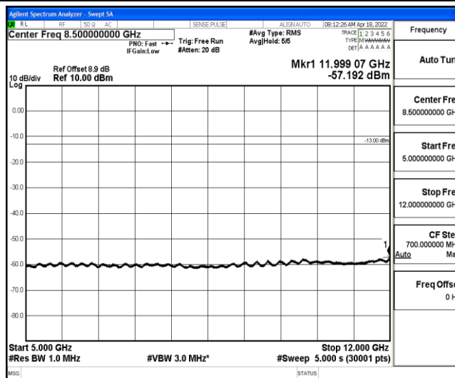
Band2-5MHz-16QAM-18625-1-0-Low-5000-12000--57.19-PASS
