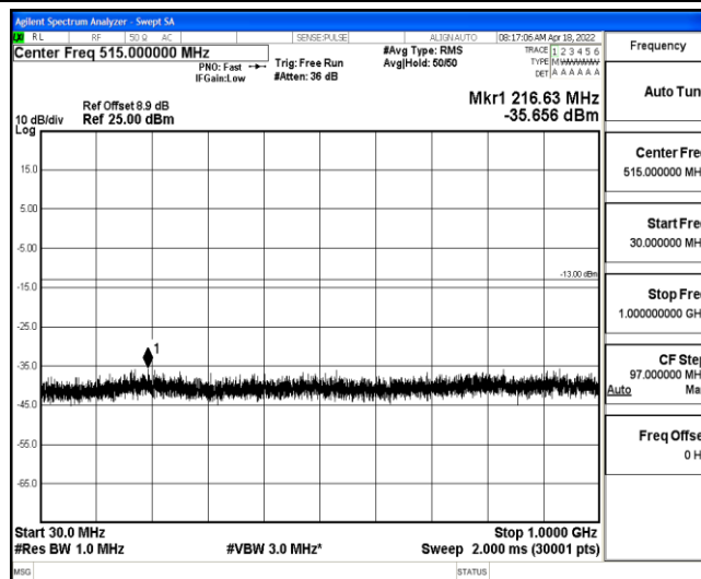
Band2-5MHz-QPSK-19175-1-0-High-30-1000--35.66-PASS
