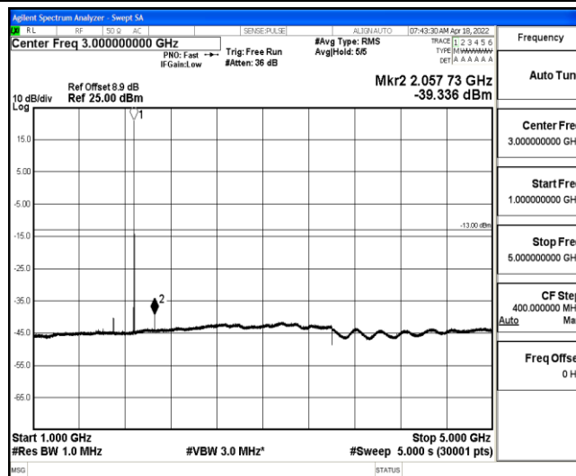
Band2-3MHz-16QAM-18900-1-0-Low-1000-5000--39.34-PASS
