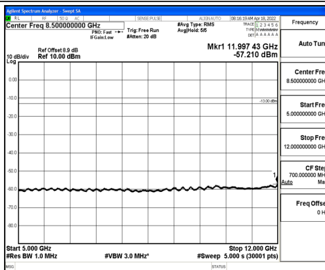
Band2-5MHz-16QAM-18900-1-0-Low-5000-12000--57.21-PASS
