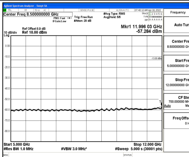
Band2-3MHz-16QAM-18615-1-0-Low-5000-12000--57.28-PASS
