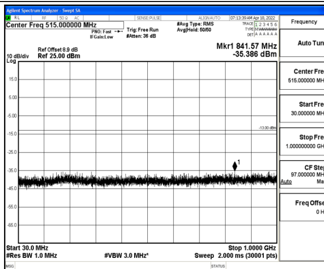
Band2-1.4MHz-16QAM-18900-1-0-Low-30-1000--35.39-PASS
