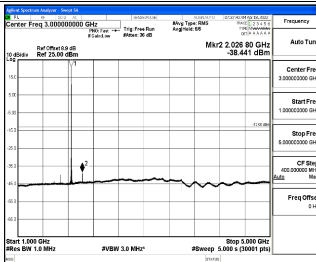
Band2-3MHz-QPSK-18615-1-0-Low-1000-5000--38.44-PASS
