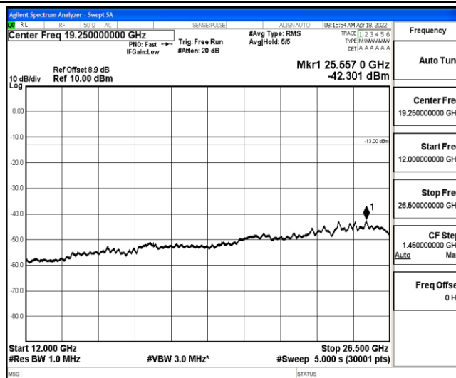
Band2-5MHz-16QAM-18900-1-0-Low-12000-26500--42.3-PASS
