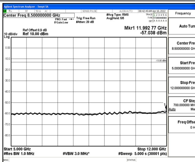
Band2-10MHz-QPSK-18900-1-0-Low-5000-12000--57.04-PASS
