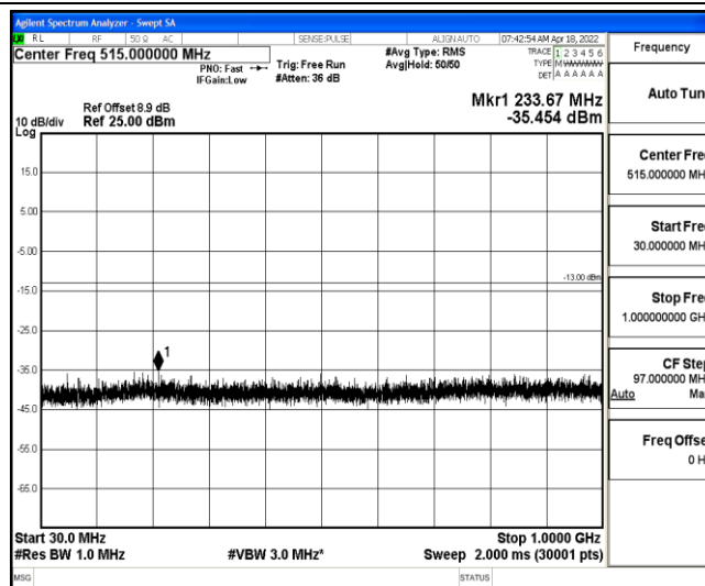
Band2-3MHz-16QAM-18900-1-0-Low-30-1000--35.45-PASS
