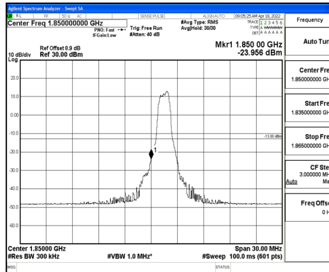
Band2-15MHz-16QAM-18675-6-0-Low--23.96-PASS
