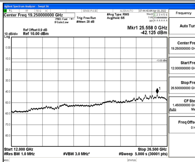
Band2-3MHz-16QAM-18900-1-0-Low-12000-26500--42.13-PASS
