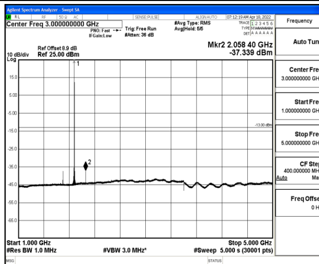
Band2-1.4MHz-QPSK-18900-1-0-Low-1000-5000--37.34-PASS
