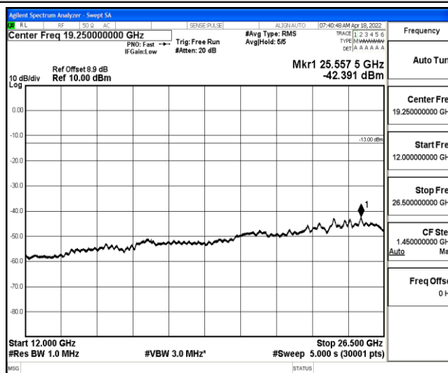
Band2-3MHz-16QAM-18615-1-0-Low-12000-26500--42.39-PASS
