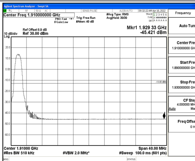
Band2-20MHz-QPSK-19100-6-0-Low--45.42-PASS
