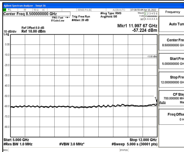
Band2-1.4MHz-QPSK-18607-1-0-Low-5000-12000--57.22-PASS
