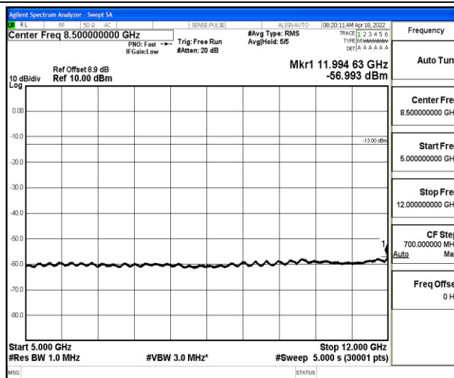
Band2-5MHz-16QAM-19175-1-0-High-5000-12000--56.99-PASS
