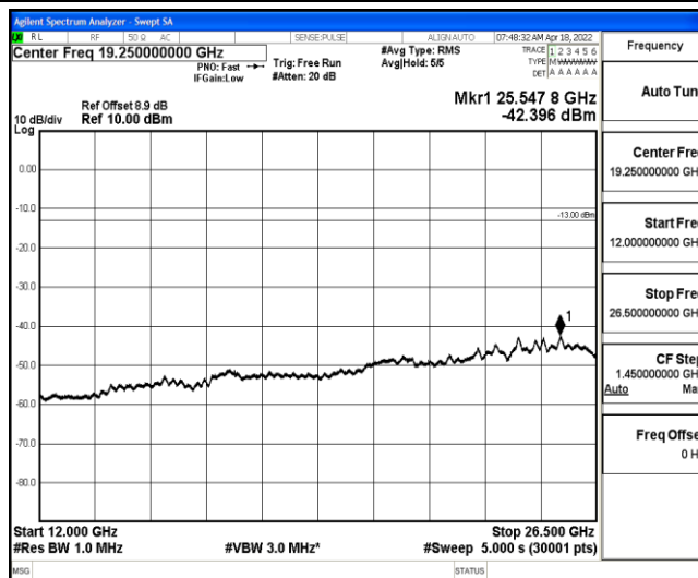
Band2-3MHz-16QAM-19185-1-0-High-12000-26500--42.4-PASS
