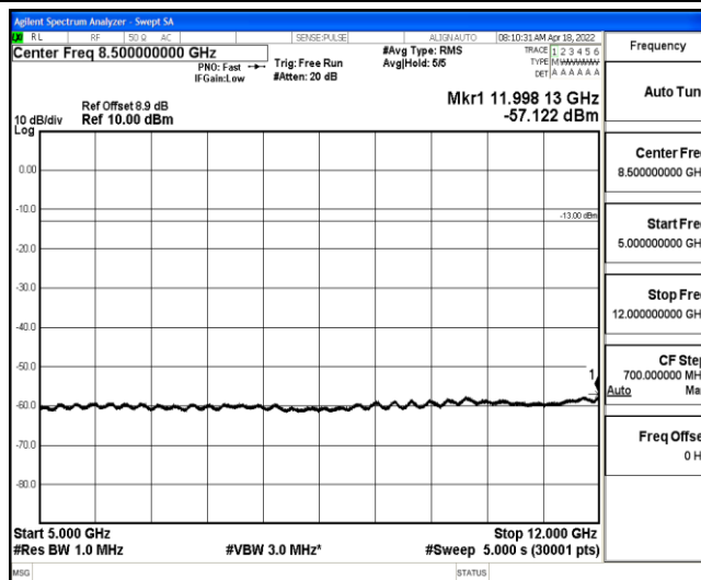
Band2-5MHz-QPSK-18625-1-0-Low-5000-12000--57.12-PASS
