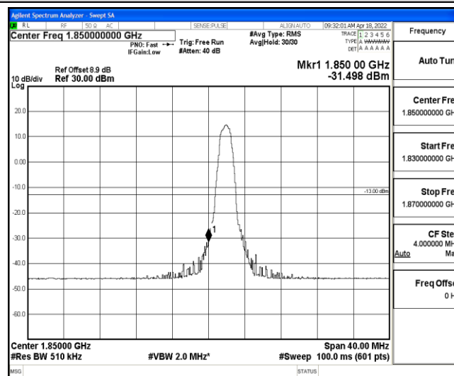
Band2-20MHz-QPSK-18700-6-0-Low--31.50-PASS
