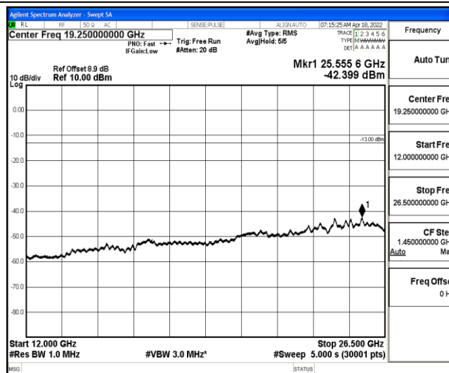
Band2-1.4MHz-16QAM-18900-1-0-Low-12000-26500--42.4-PASS
