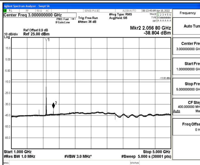
Band2-5MHz-QPSK-18900-1-0-Low-1000-5000--38.8-PASS
