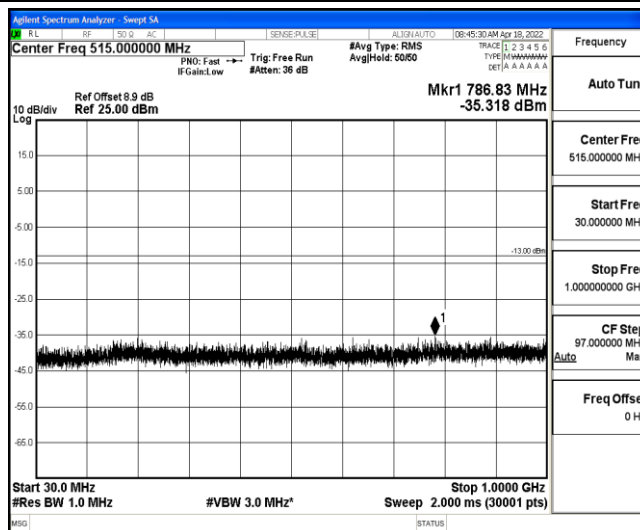
Band2-10MHz-QPSK-19150-1-0-High-30-1000--35.32-PASS
