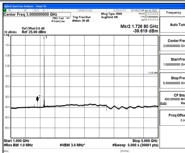
Band2-3MHz-QPSK-19185-1-0-High-1000-5000--39.62-PASS
