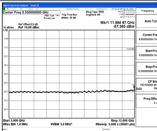
Band2-3MHz-QPSK-18900-1-0-Low-5000-12000--57.36-PASS
