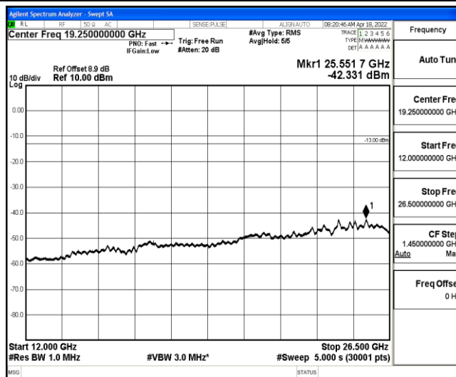
Band2-5MHz-16QAM-19175-1-0-High-12000-26500--42.33-PASS
