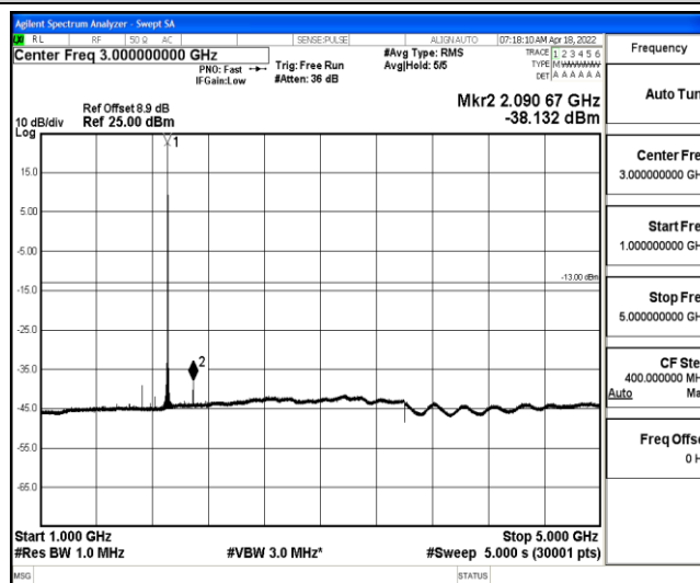
Band2-1.4MHz-16QAM-19193-1-0-High-1000-5000--38.13-PASS
