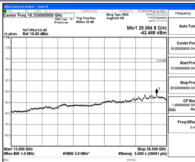
Band2-3MHz-QPSK-18615-1-0-Low-12000-26500--42.47-PASS
