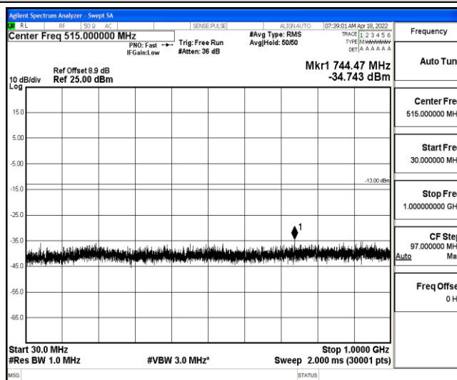
Band2-3MHz-16QAM-18615-1-0-Low-30-1000--34.74-PASS
