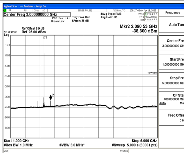
Band2-5MHz-QPSK-19175-1-0-High-1000-5000--38.3-PASS
