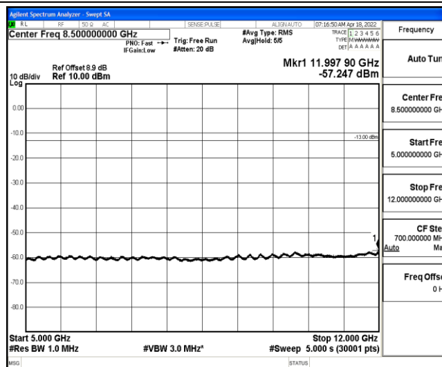
Band2-1.4MHz-QPSK-19193-1-0-High-5000-12000--57.25-PASS
