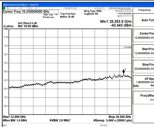
Band2-5MHz-QPSK-19175-1-0-High-12000-26500--42.44-PASS
