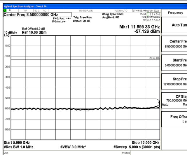
Band2-3MHz-16QAM-18900-1-0-Low-5000-12000--57.13-PASS
