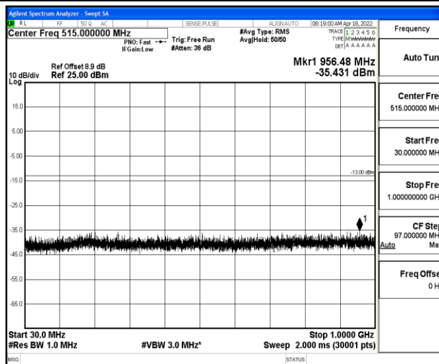
Band2-5MHz-16QAM-19175-1-0-High-30-1000--35.43-PASS
