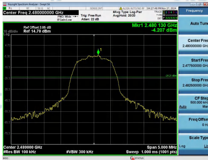
2_Spurious_Emissions_NVNT_ANT1_2-DH5_2480_00
