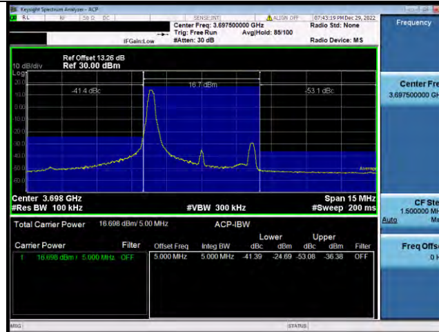
Band48-5MHz-QPSK-56715-1RB#24
