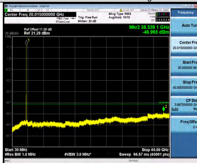
Band48-10MHz-64QAM-56690-1RB#0-Range1:30~40000MHz
