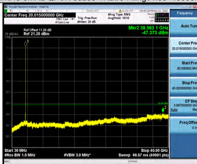
Band48-5MHz-QPSK-55990-1RB#0-Range1:30~40000MHz
