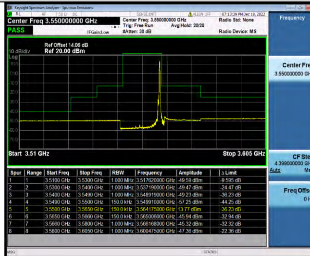
Band48-15MHz-64QAM-55315-75RB#0
