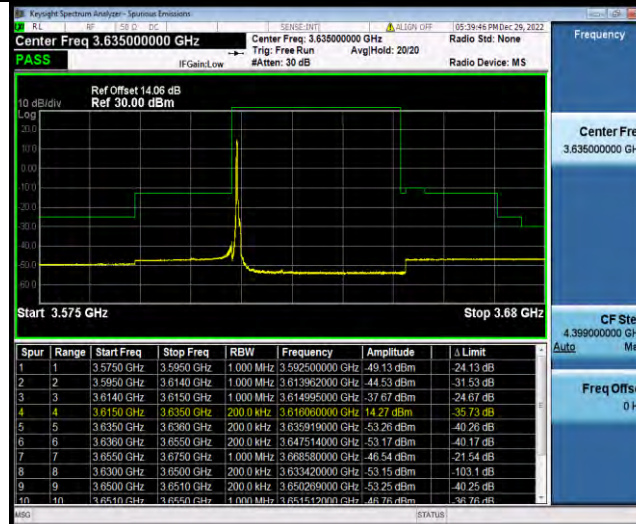
Band48-20MHz-16QAM-55990-1RB#99
