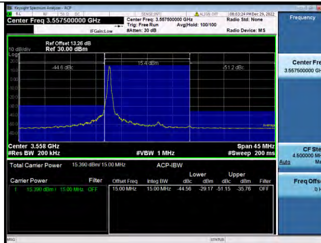
Band48-15MHz-QPSK-55315-75RB#0
