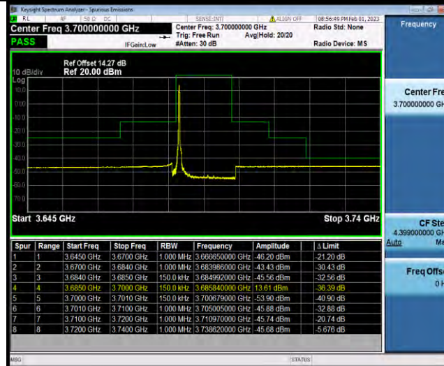
Band48-15MHz-64QAM-56665-1RB#74
