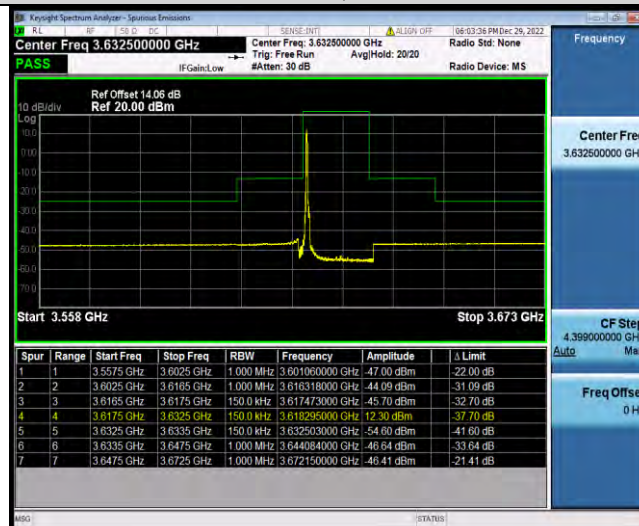
Band48-15MHz-64QAM-55990-1RB#74
