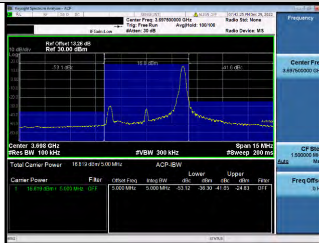
Band48-5MHz-QPSK-56715-25RB#0
