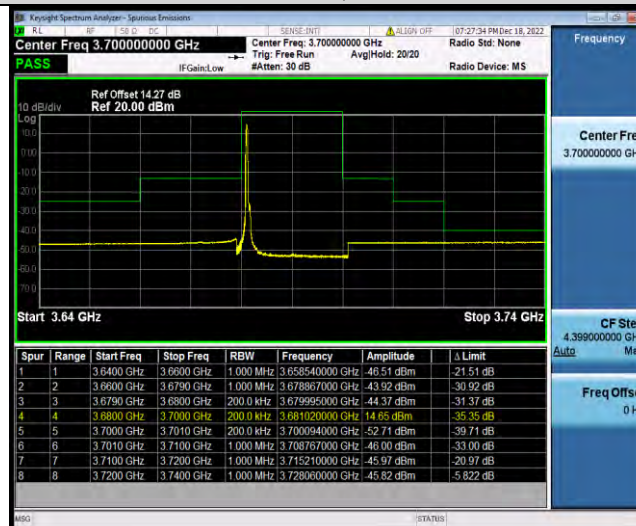
Band48-20MHz-16QAM-56640-1RB#99
