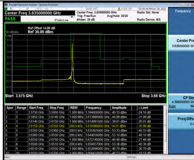
Band48-20MHz-64QAM-55990-1RB#99
