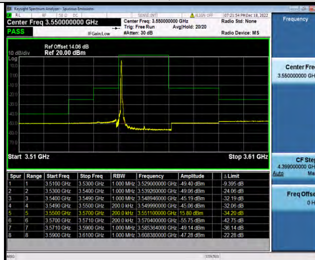
Band48-20MHz-16QAM-55340-1RB#99
