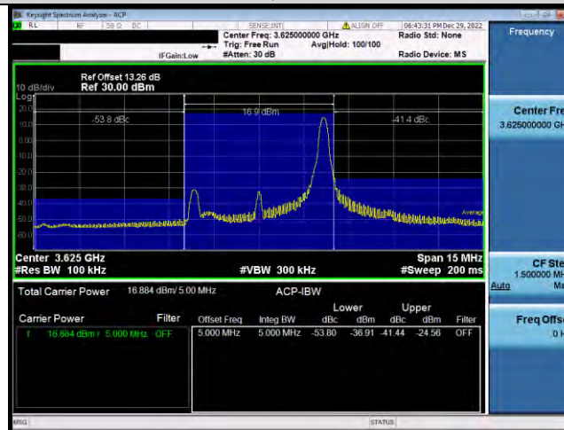
Band48-5MHz-QPSK-55990-25RB#0
