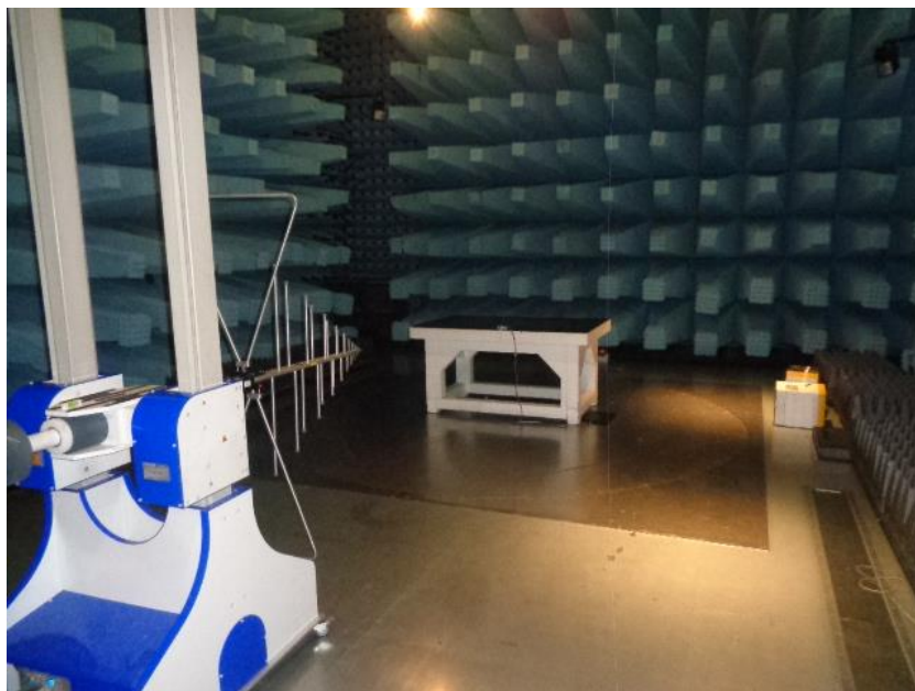
Figure 9.1-2: Radiated emissions set-up for frequencies below 1 GHz
