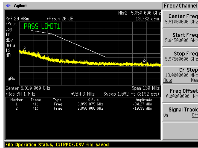
Ant-4
