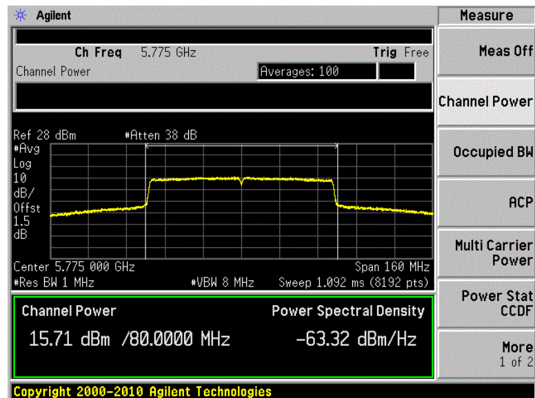
Ant-6
