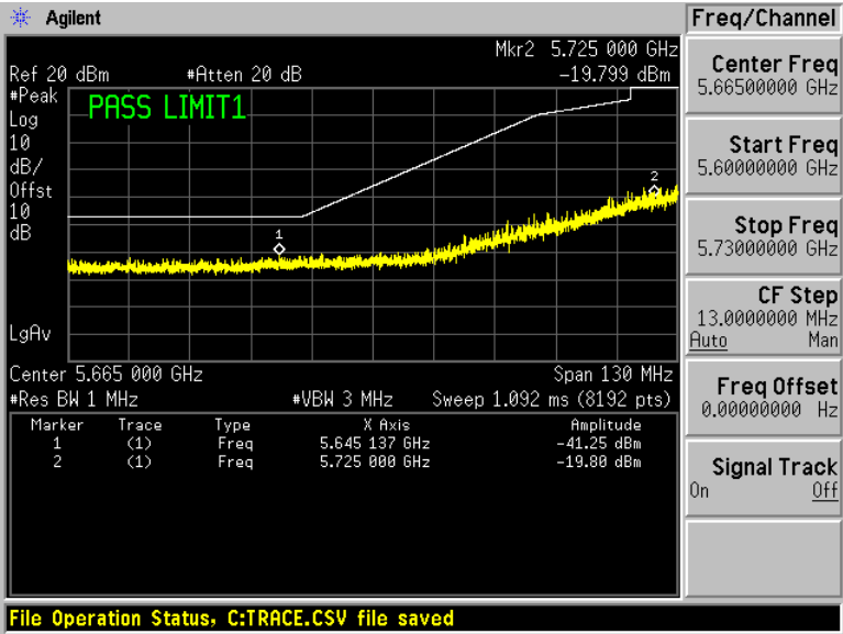
Ant-2
