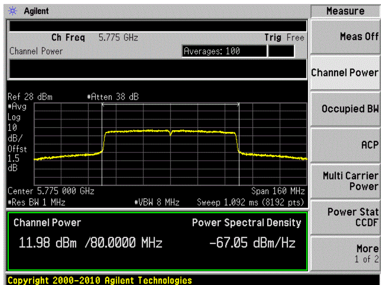
Ant-5
