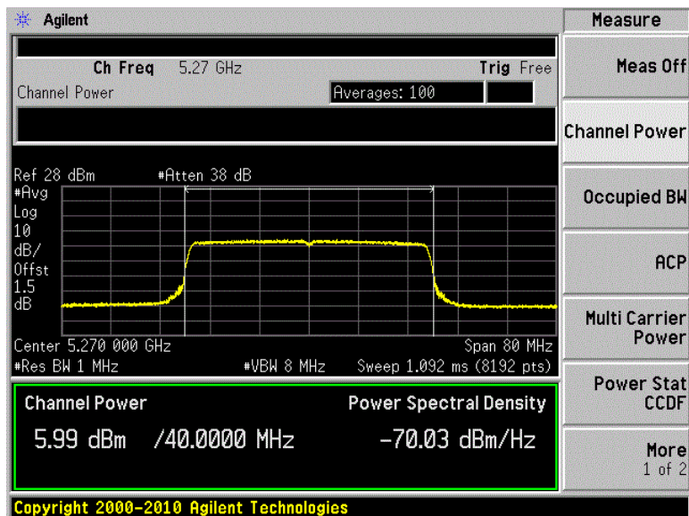
Ant-1
