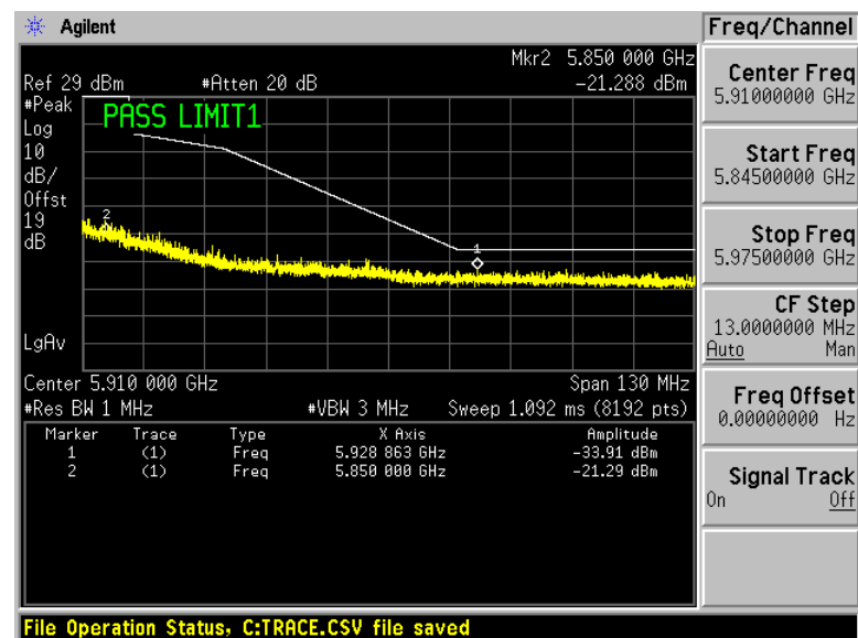
Ant-4
