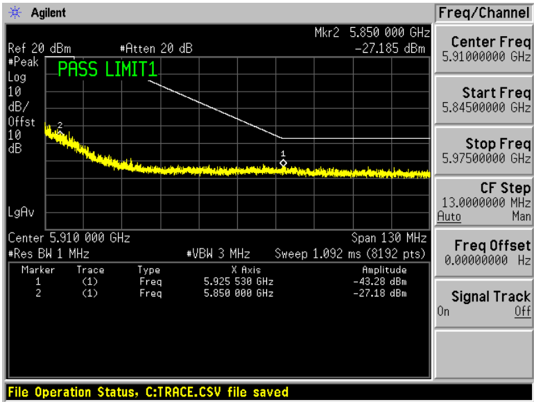
Ant-2
