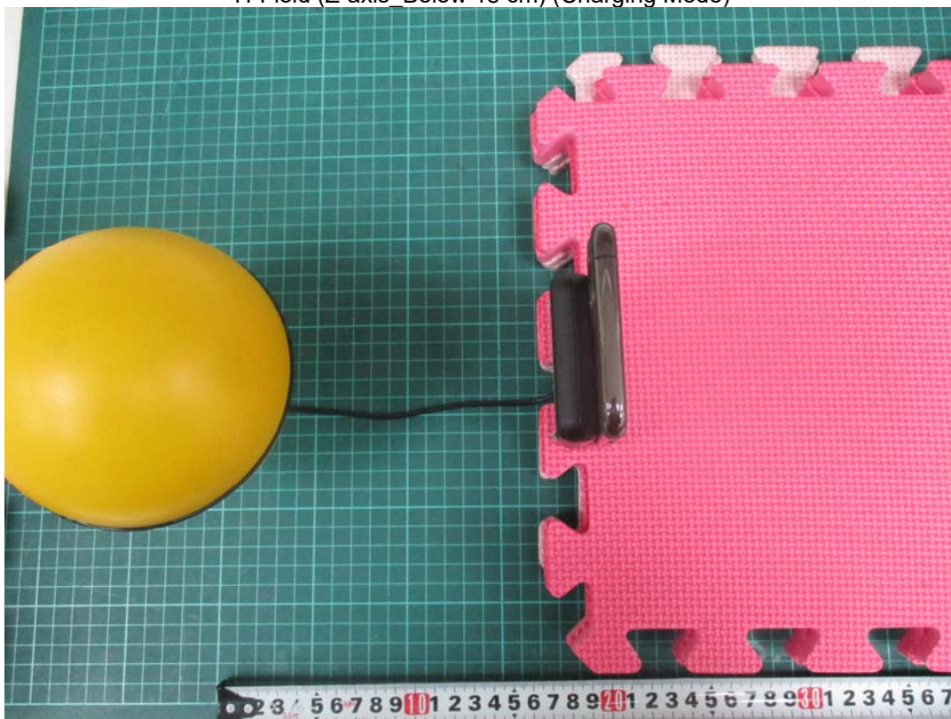
H-Field (Z-axis_Below 18 cm) (Charging Mode)
