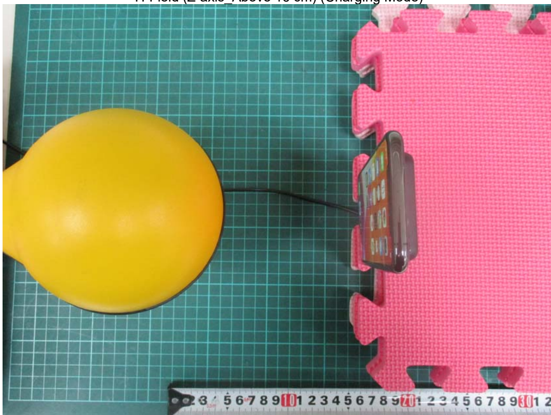
H-Field (Z-axis_Above 16 cm) (Charging Mode)
