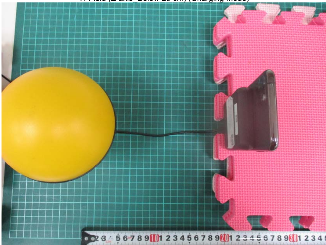
H-Field (Z-axis_Below 20 cm) (Charging Mode)
