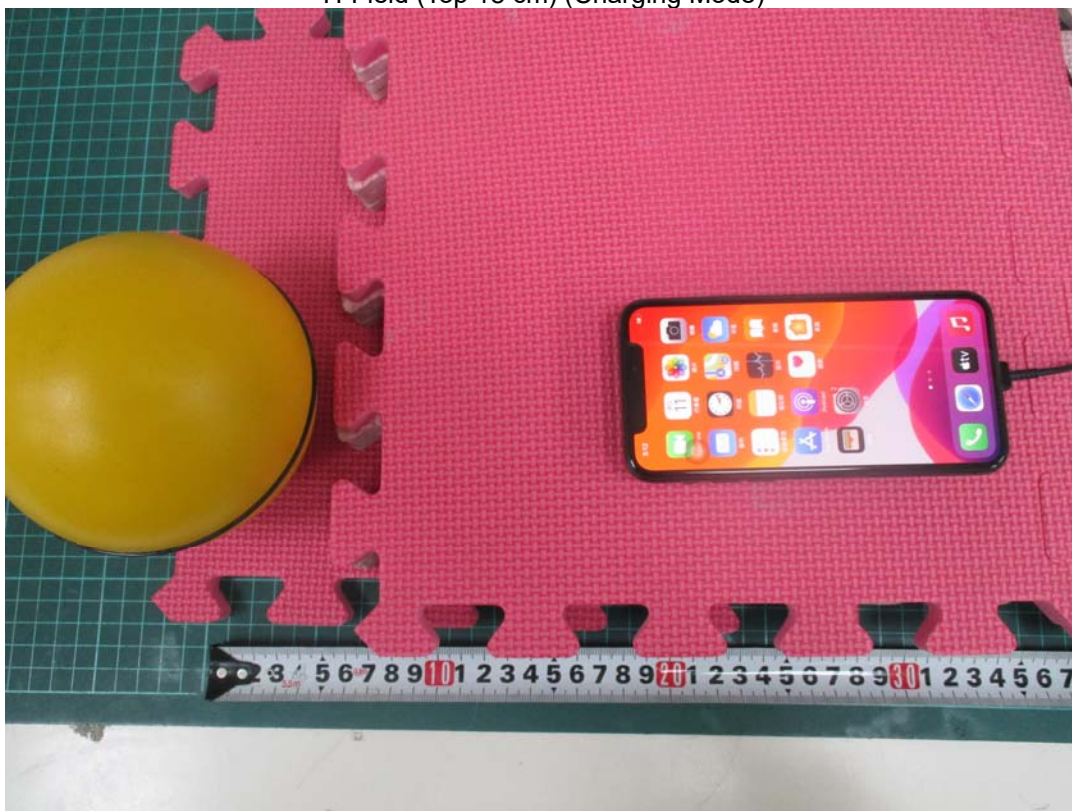
H-Field (Top 18 cm) (Charging Mode)
