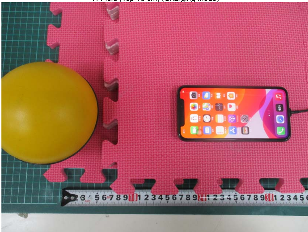
H-Field (Top 16 cm) (Charging Mode)
