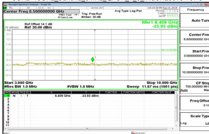
3GHz~10GHz_Band12_5MHz_QPSK_1_0_MidCH23095-707.5
