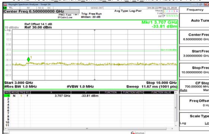
3GHz~10GHz_Band12_3MHz_QPSK_1_0_MidCH23095-707.5
