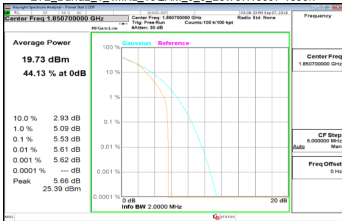
LTE_Band2_1_4MHz_64QAM_6_0_LowCH18607-1850.7
