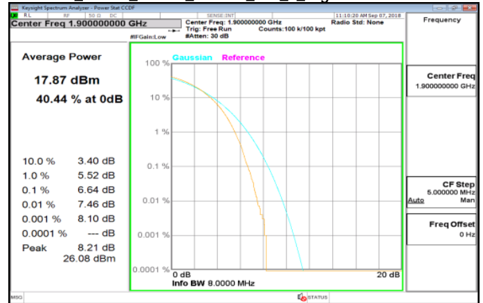
LTE_Band2_20MHz_64QAM_100_0_HighCH19100-1900
