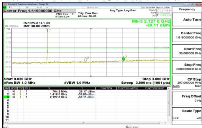
30MHz~3GHz_Band17_10MHz_QPSK_1_0_LowCH23780-709
