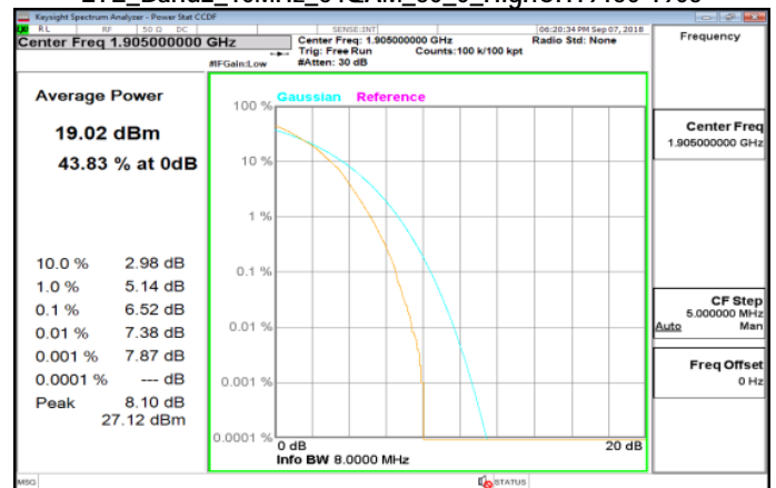
LTE_Band2_10MHz_64QAM_50_0_HighCH19150-1905
