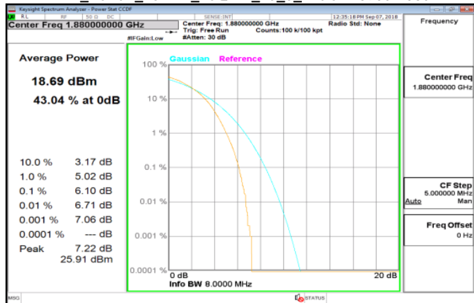
LTE_Band2_15MHz_16QAM_75_0_MidCH18900-1880
