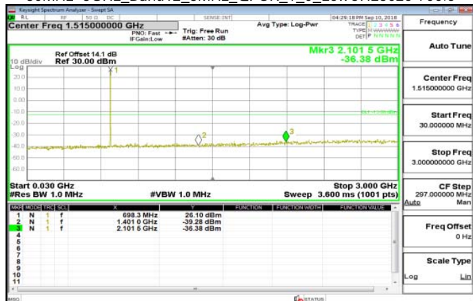
30MHz~3GHz_Band12_3MHz_QPSK_1_0_LowCH23025-700.5
