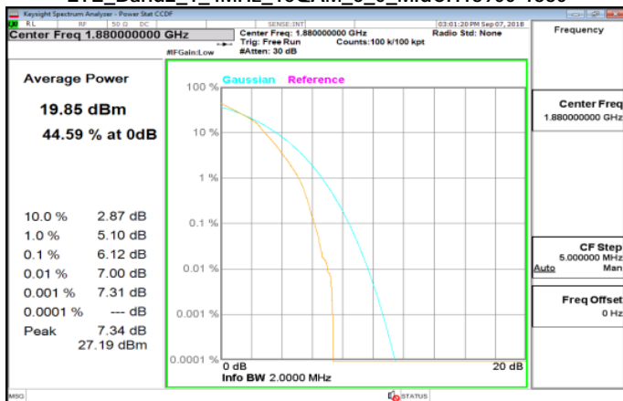
LTE_Band2_1_4MHz_16QAM_6_0_MidCH18900-1880
