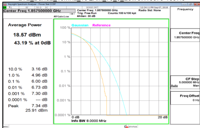
LTE_Band2_15MHz_64QAM_75_0_LowCH18675-1857.5
