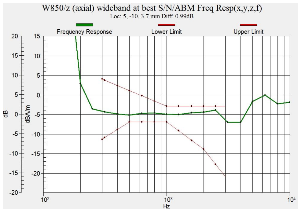
Figure B.4 Frequency Response of WCDMA Band 5
