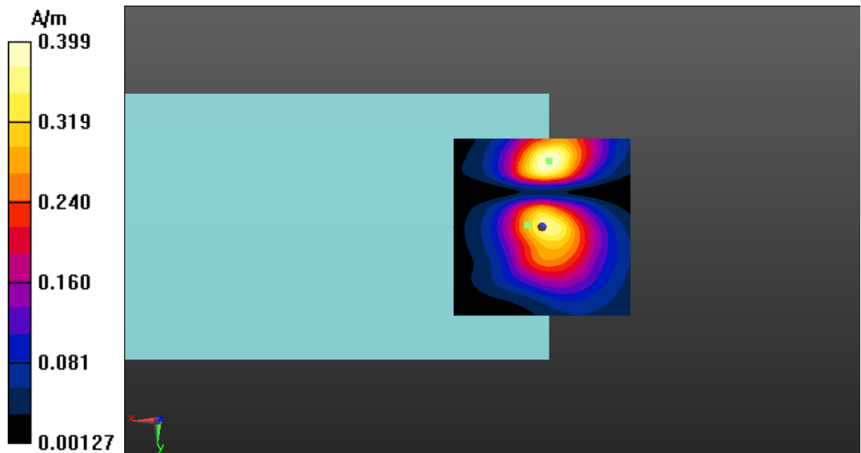
Fig A.9 T-Coil WLAN 2.4G-Y
