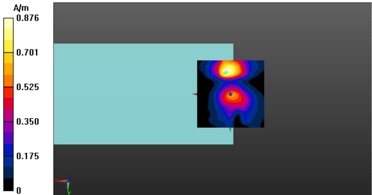
Fig A.11 T-Coil GSM 1900-Y
