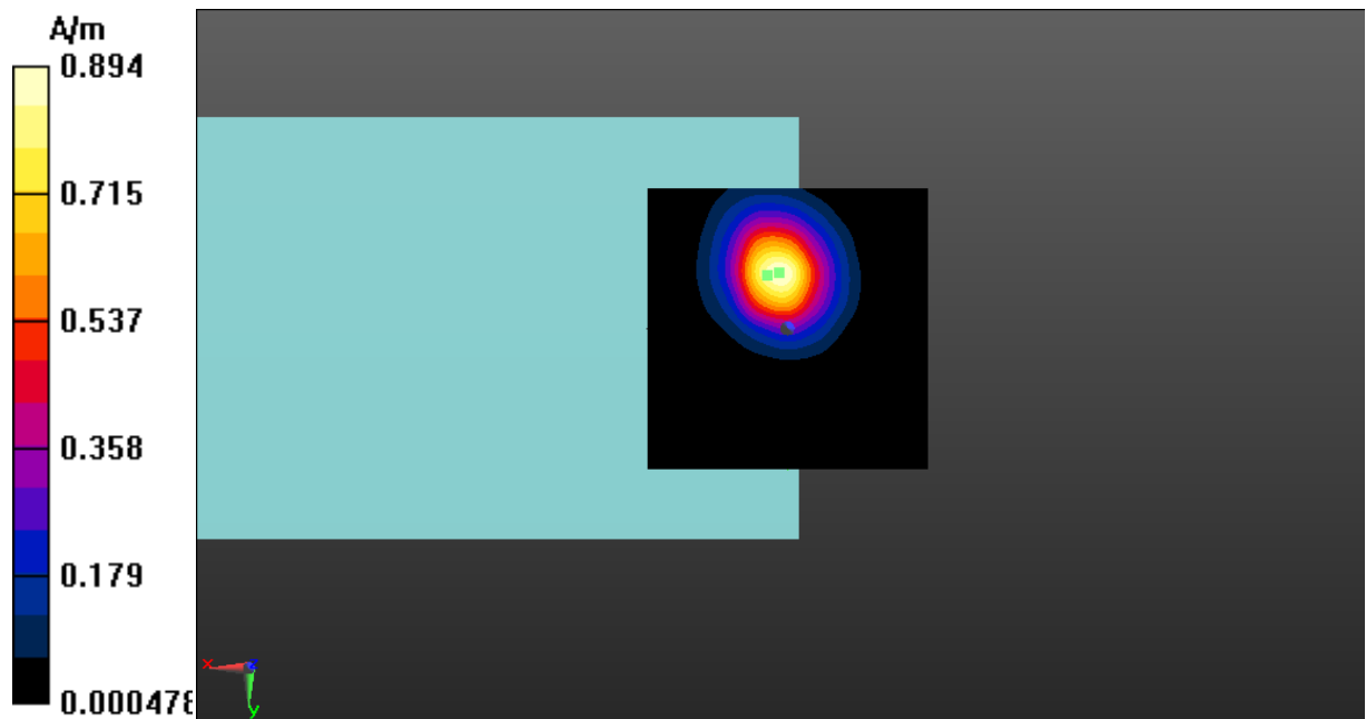
Fig A.8 T-Coil LTE-Band 41-Z
