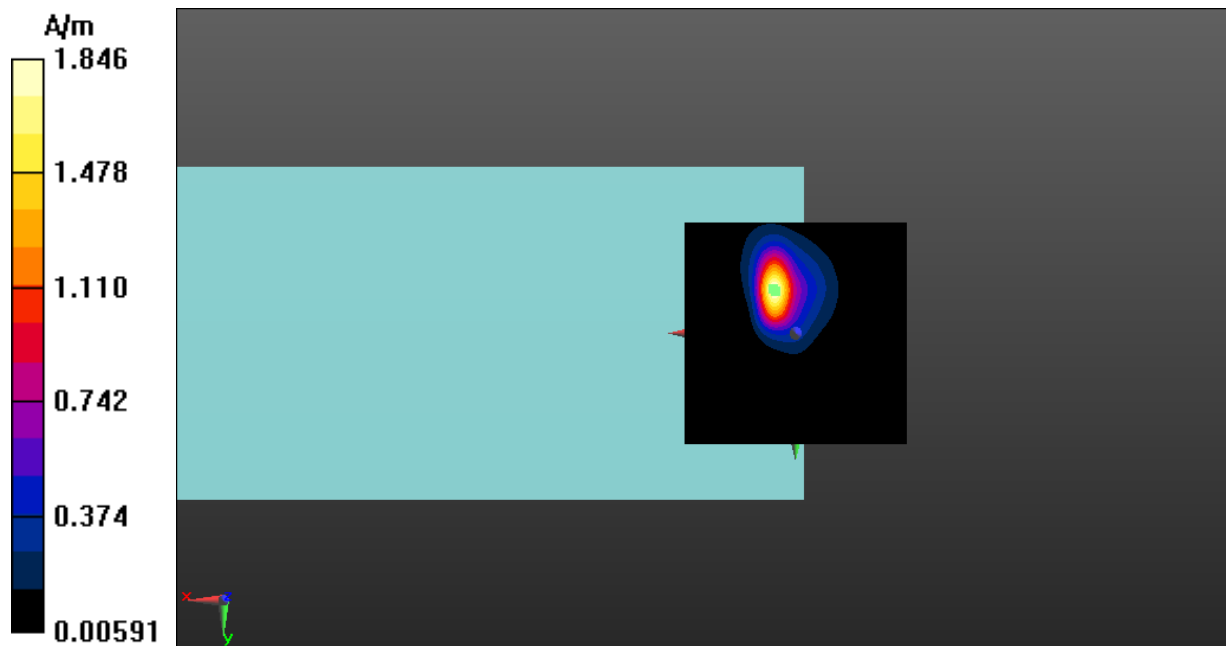
Fig A.9 T-Coil WLAN 2.4G-Z
