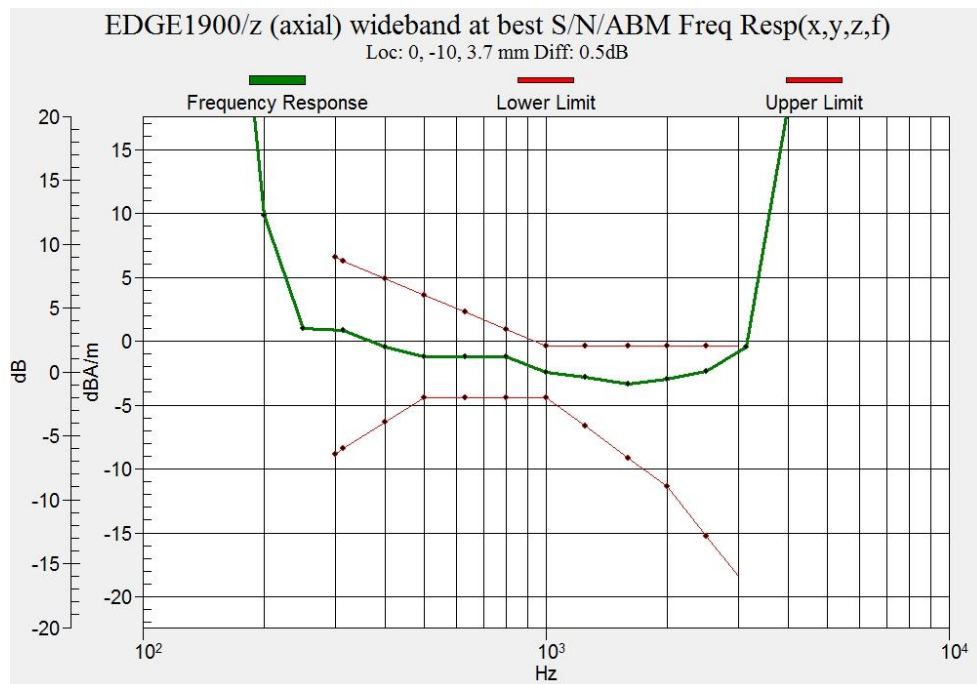
Figure B.11 Frequency Response of GSM 1900 (Google Duo)
