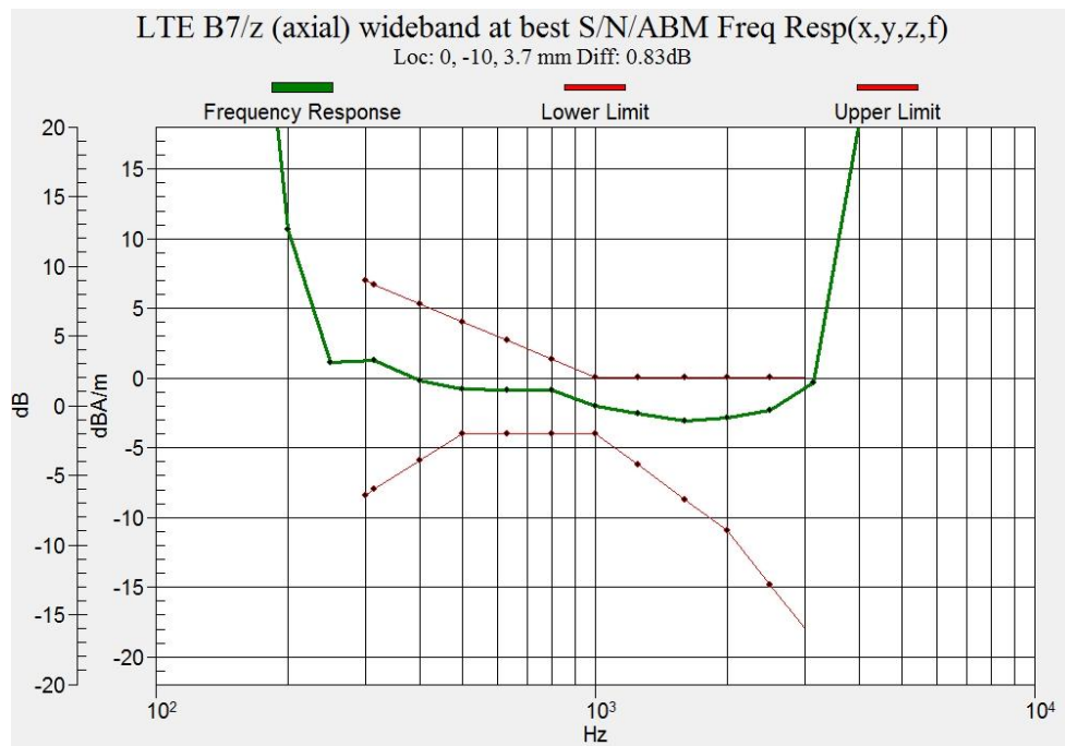
Figure B.14 Frequency Response of LTE Band 7 (Google Duo)
