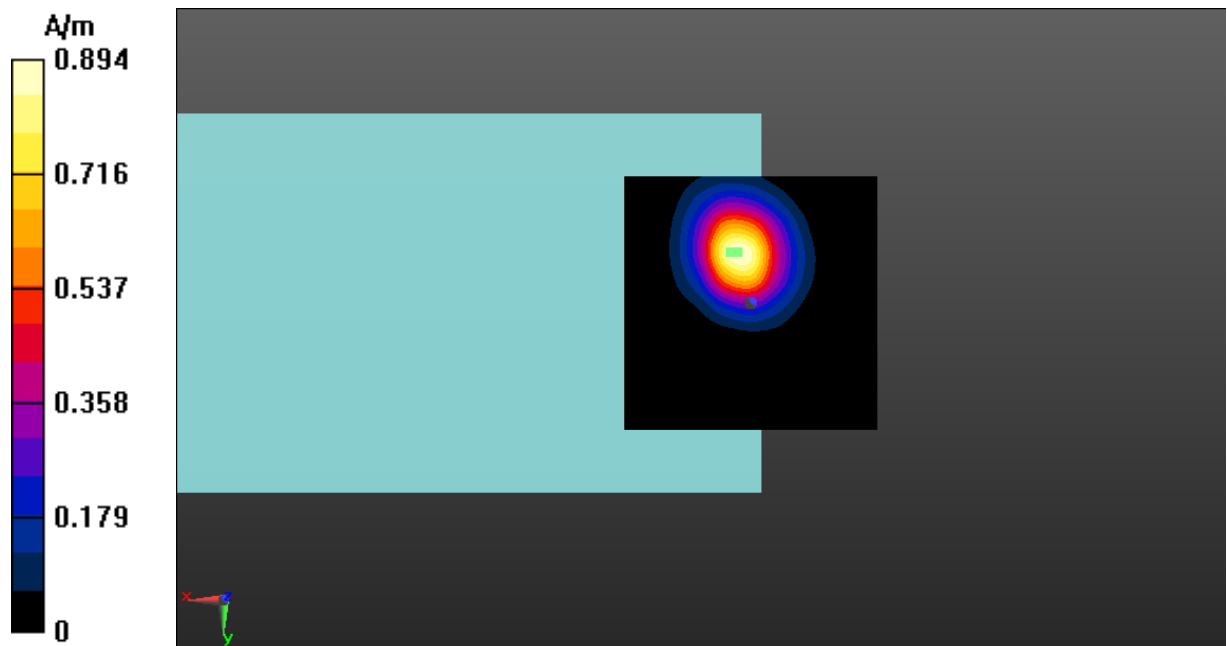
Fig A.7 T-Coil LTE-Band 38-Z
