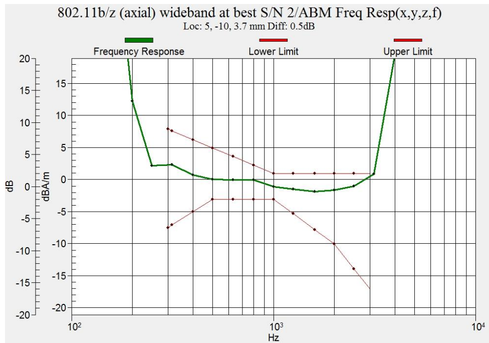
Figure B.15 Frequency Response of WLAN 2.4G (Google Duo)
