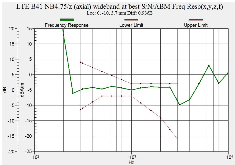
Figure B.8 Frequency Response of LTE Band 41
