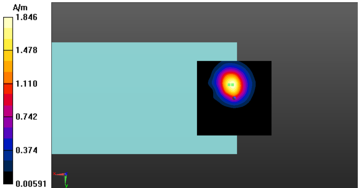
Fig A.14 T-Coil LTE-Band 7-Z
