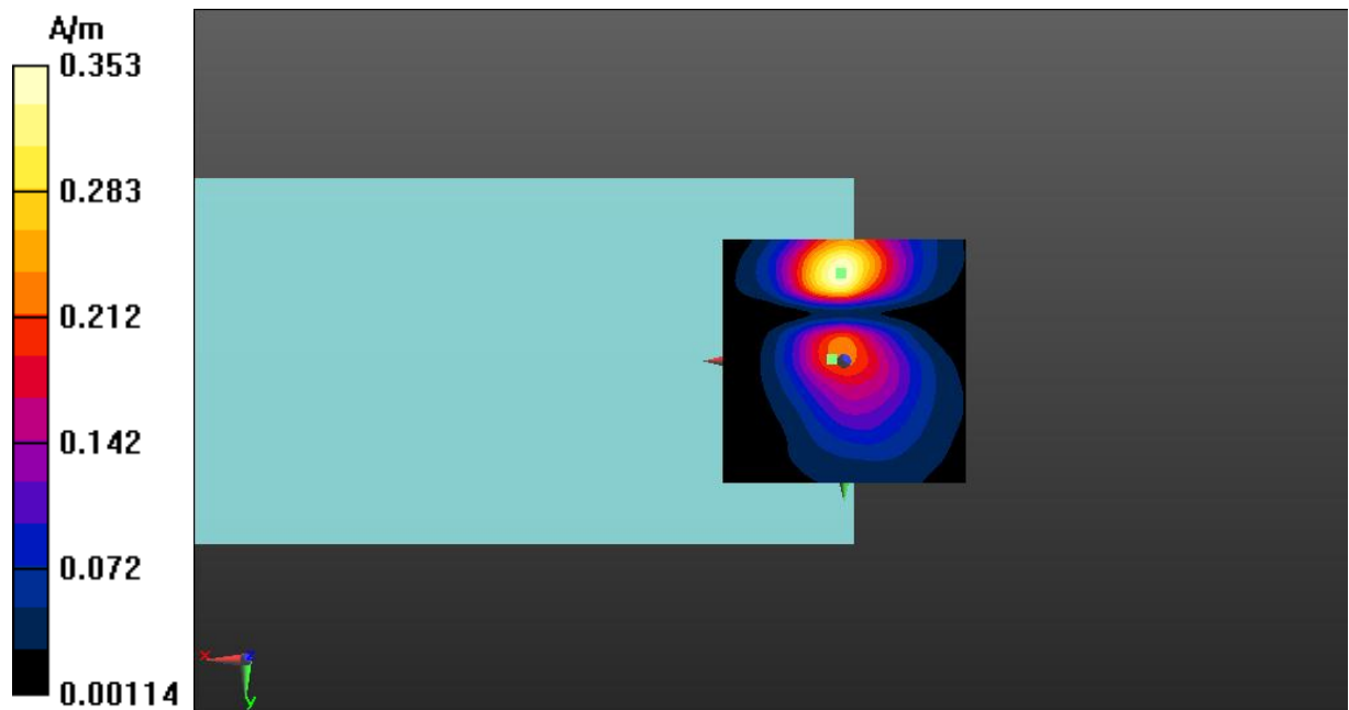
Fig A.7 T-Coil LTE-Band 38-Y
