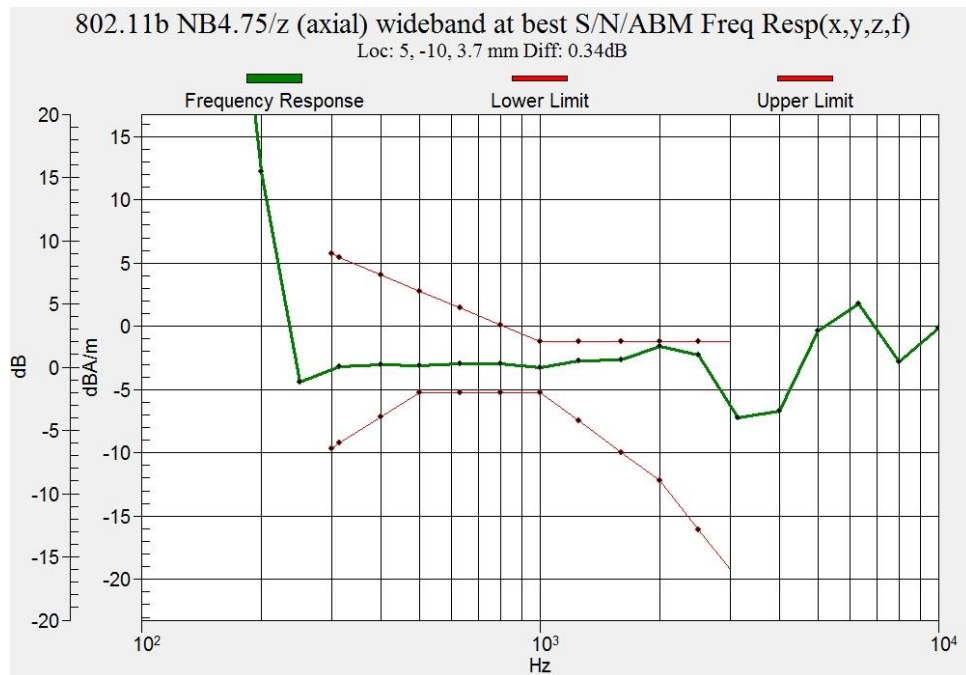
Figure B.9 Frequency Response of WLAN 2.4G
