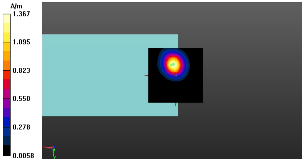
Fig A.5 T-Coil LTE-Band 5-Z
