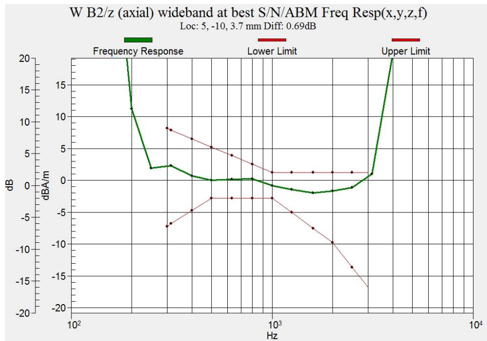
Figure B.12 Frequency Response of WCDMA Band 2 (Google Duo)
