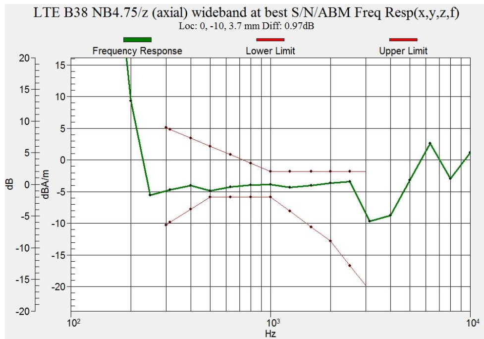
Figure B.7 Frequency Response of LTE Band 38
