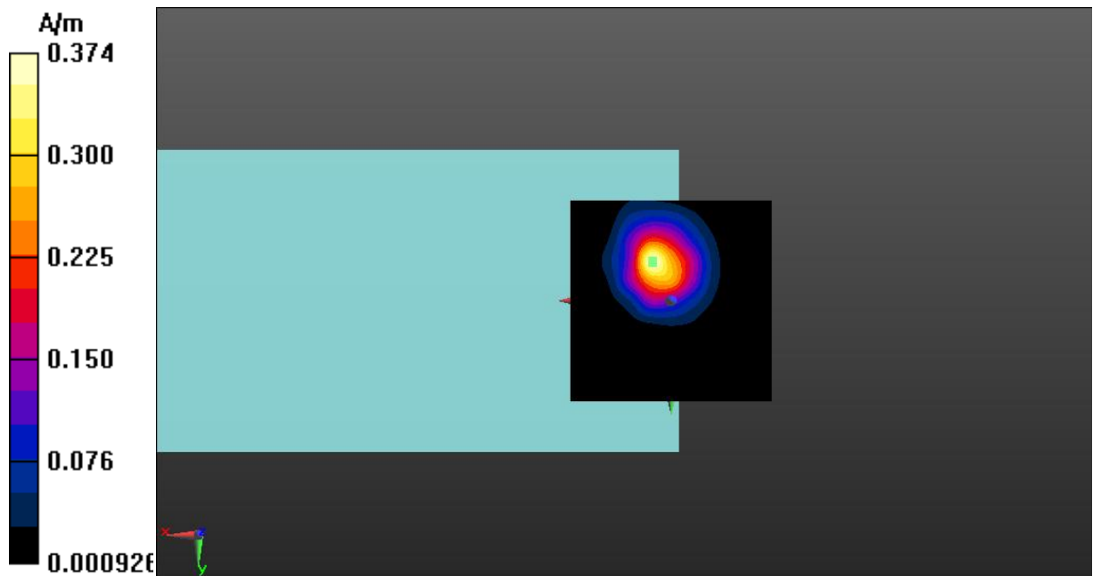
Fig A.13 T-Coil WCDMA Band 5-Z
