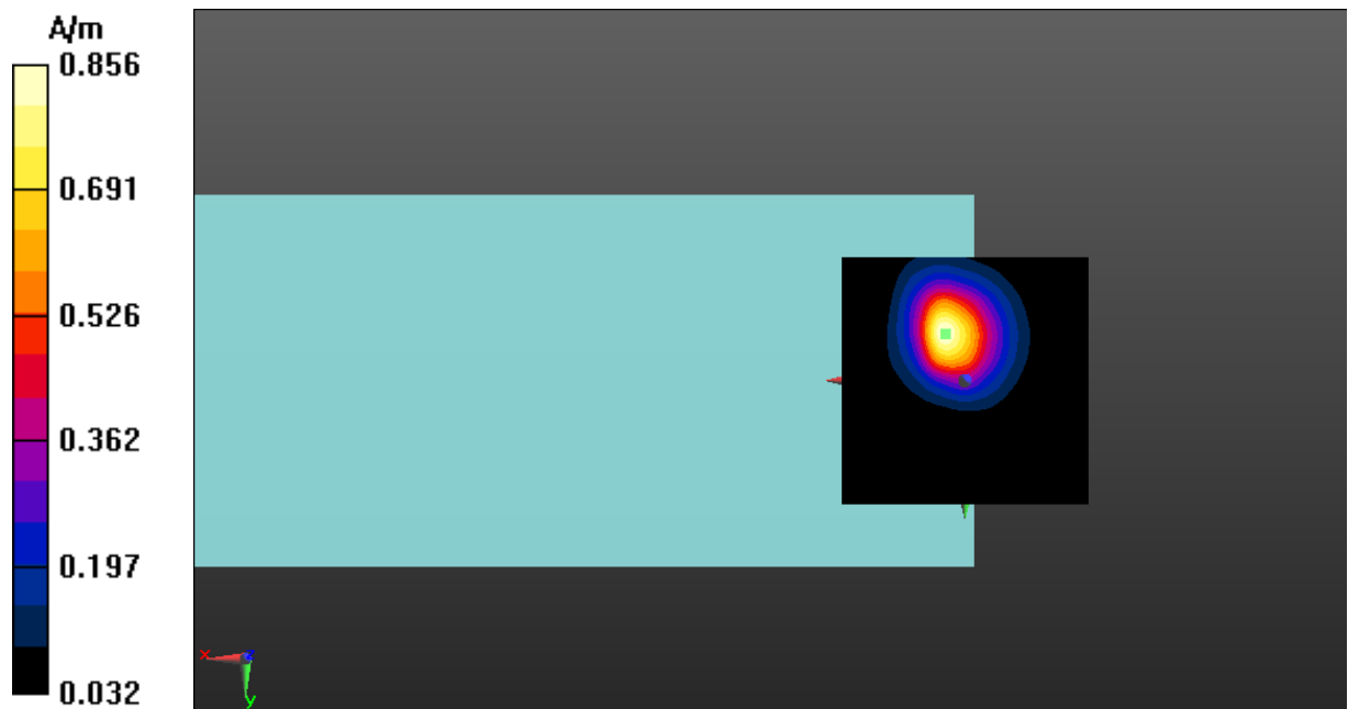
Fig A.4 T-Coil WCDMA Band 5-Z
