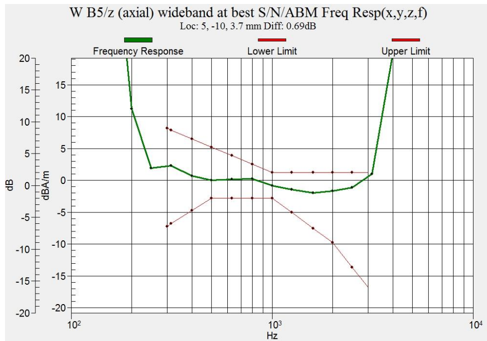
Figure B.13 Frequency Response of WCDMA Band 5 (Google Duo)
