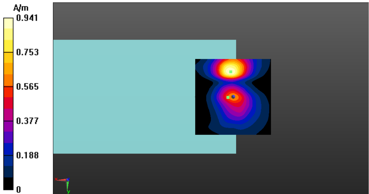
Fig A.13 T-Coil WCDMA Band 5-Y
