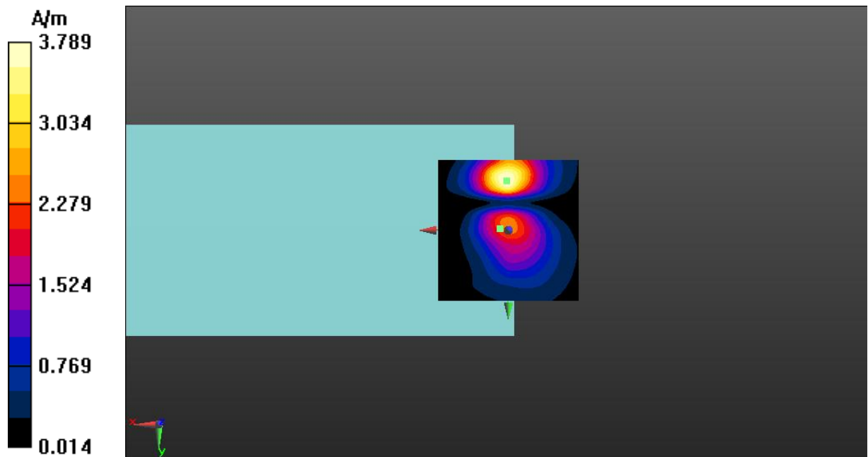
Fig A.5 T-Coil LTE-Band 5-Y
