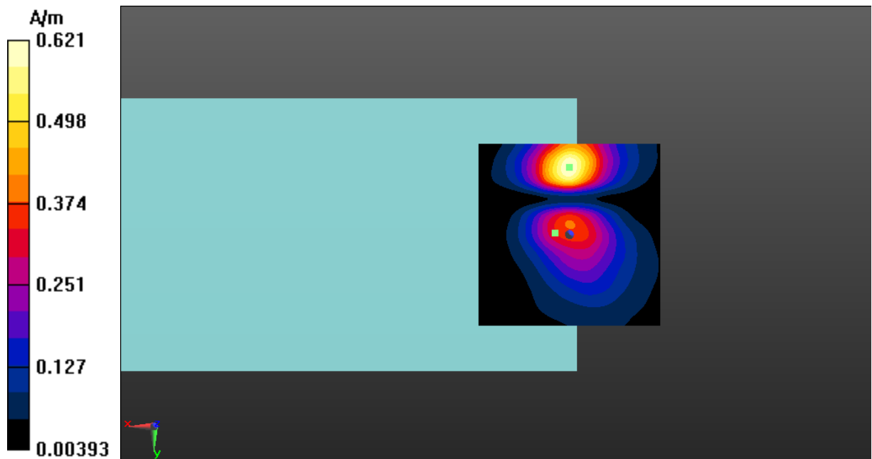
Fig A.6 T-Coil LTE-Band 7-Y
