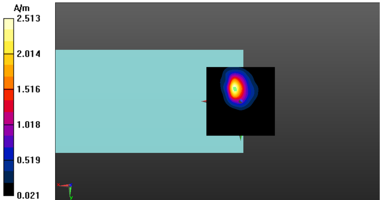
Fig A.15 T-Coil WLAN 2.4G-Z
