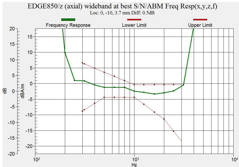
Figure B.10 Frequency Response of GSM 850 (Google Duo)
