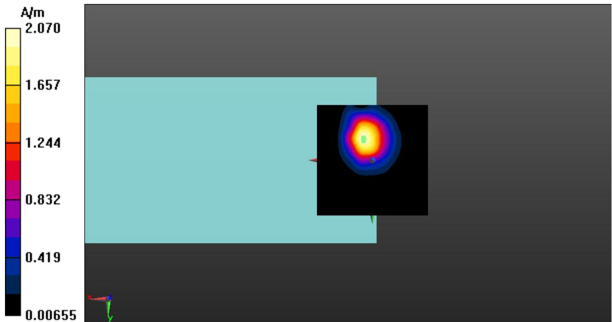
Fig A.11 T-Coil GSM 1900-Z
