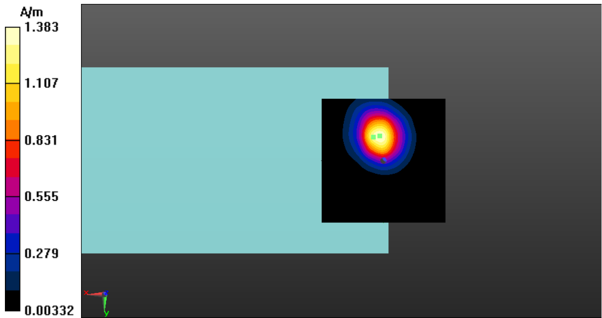
Fig A.6 T-Coil LTE-Band 7-Z
