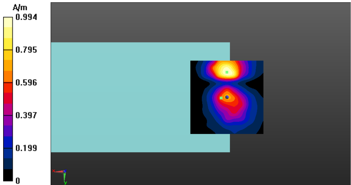
Fig A.14 T-Coil LTE-Band 7-Y
