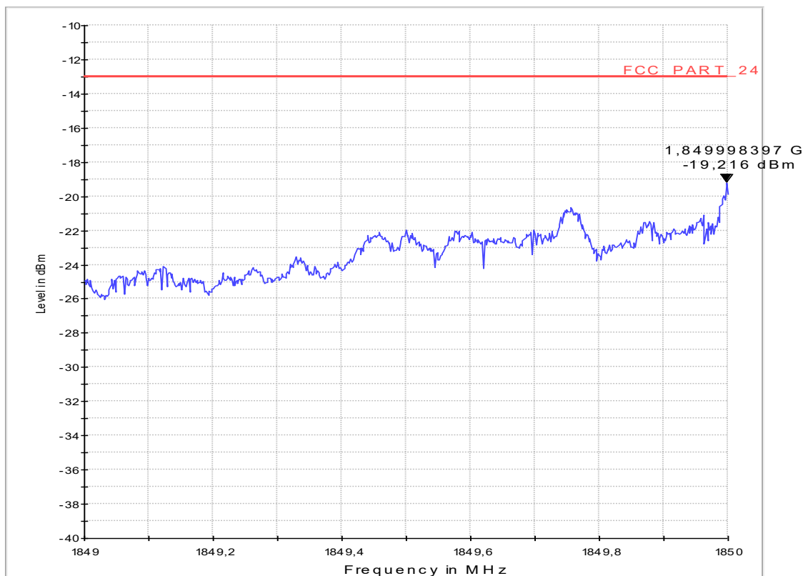
Sweep_3a_Band_Edge_Channel_9262_PK
