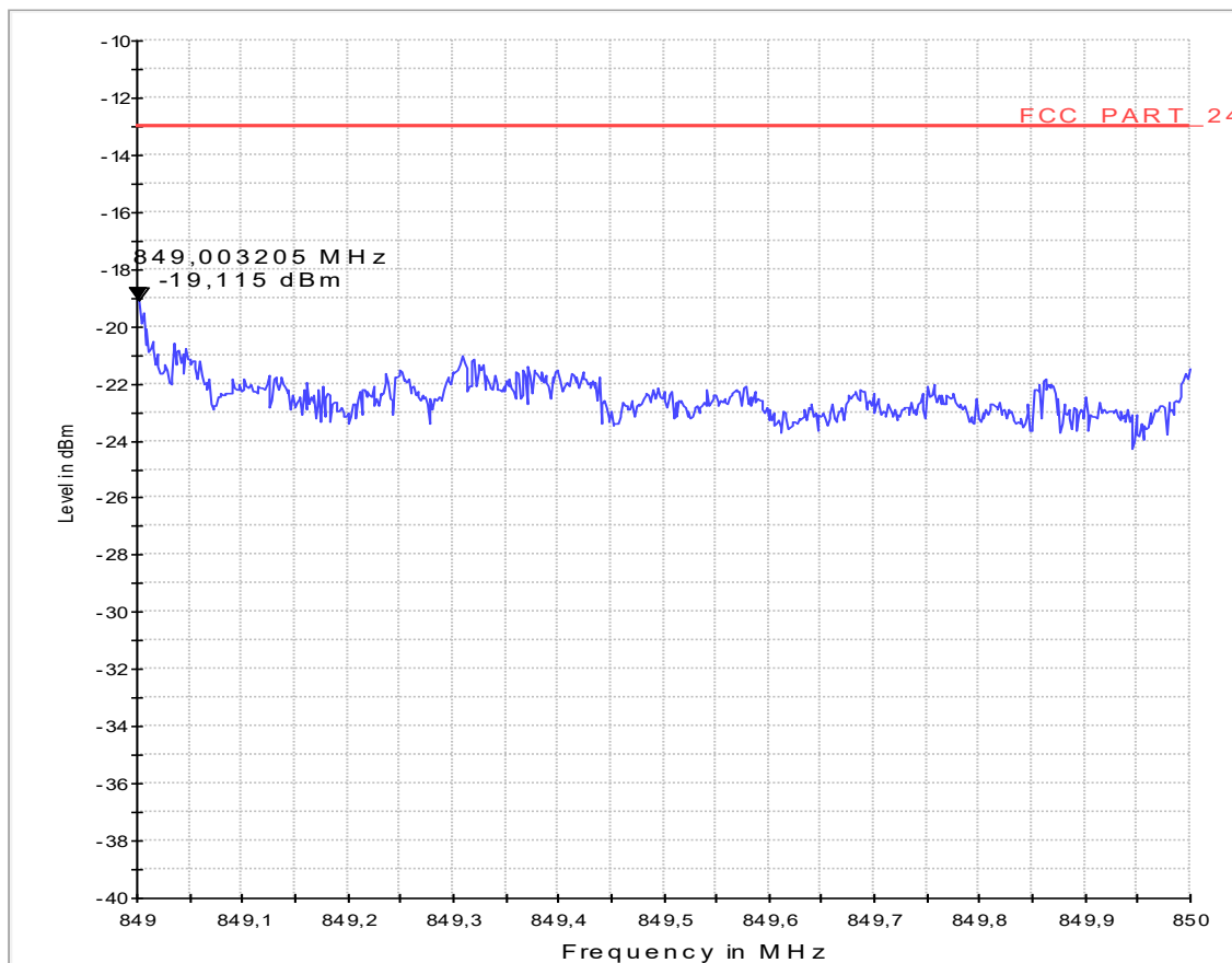
Sweep_4a_Band_Edge_Channel_4233_PK
