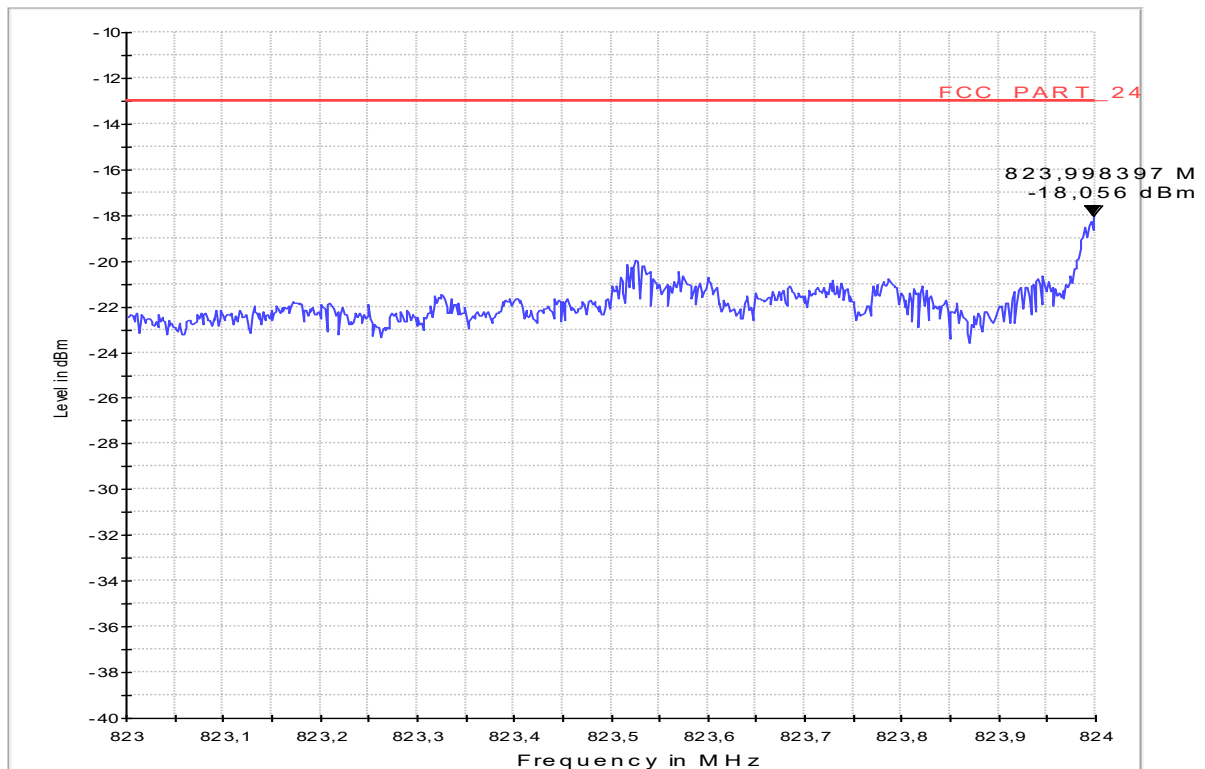
Sweep_3a_Band_Edge_Channel_4132_PK
