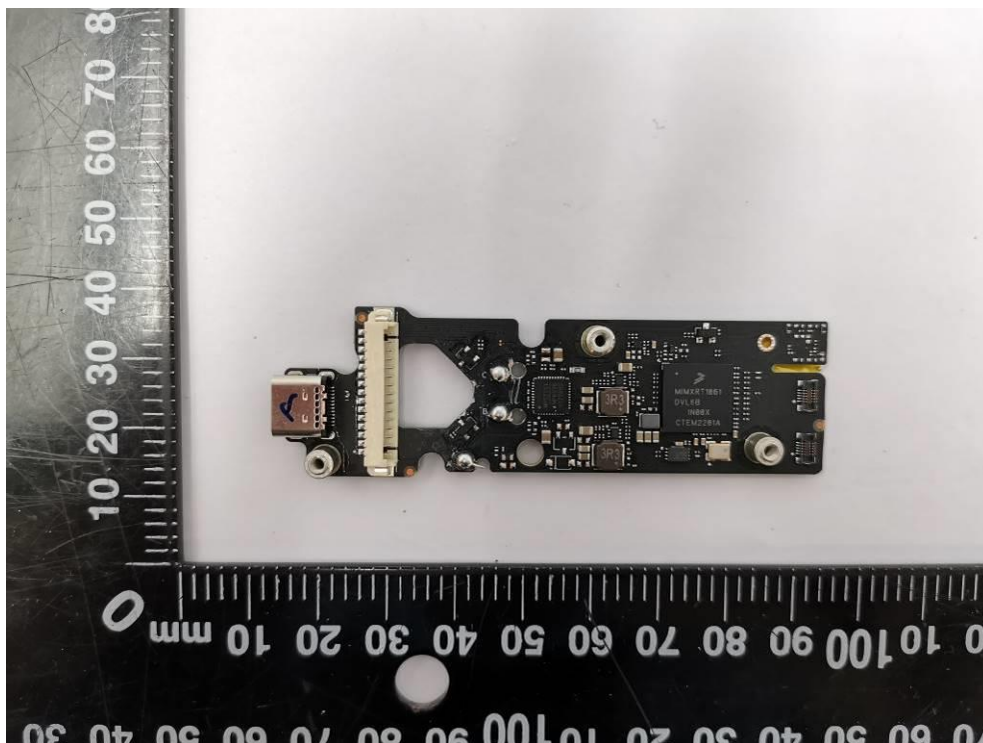
Photo- 08 PCB view-07
