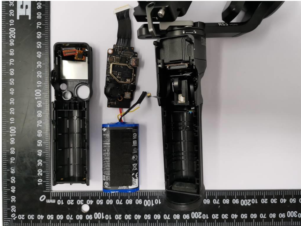
Photo- 01 Internal view
