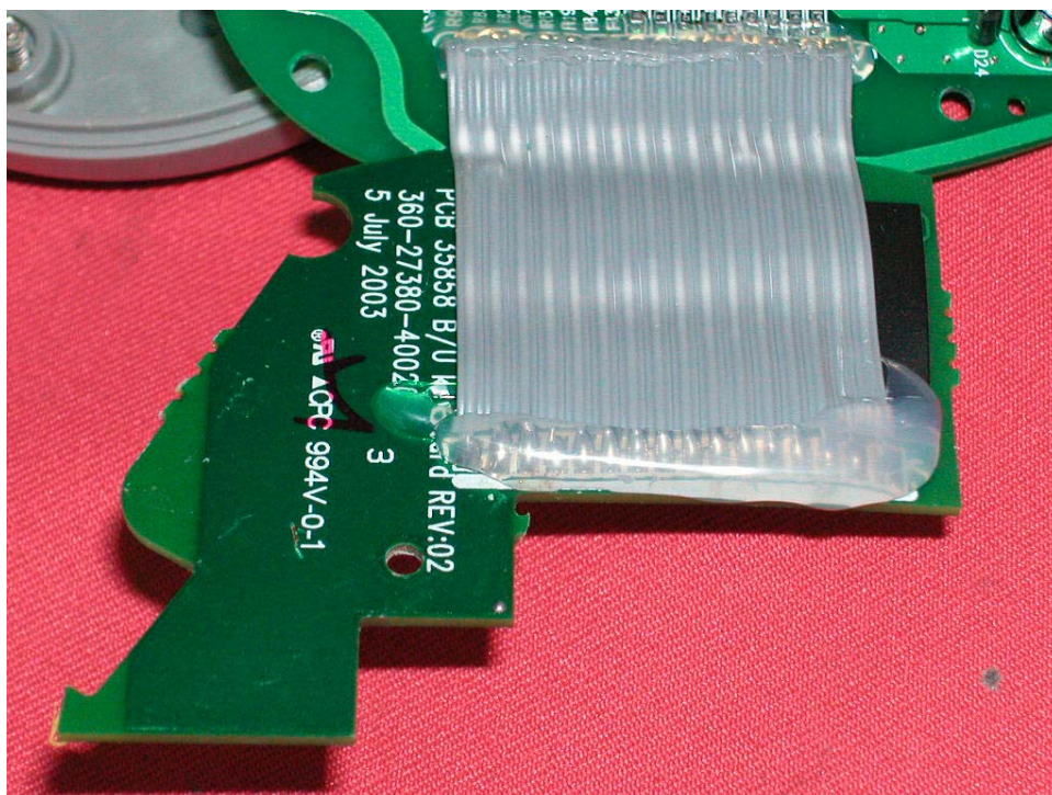
Base DAM keypad PCB rear side (View 2)
