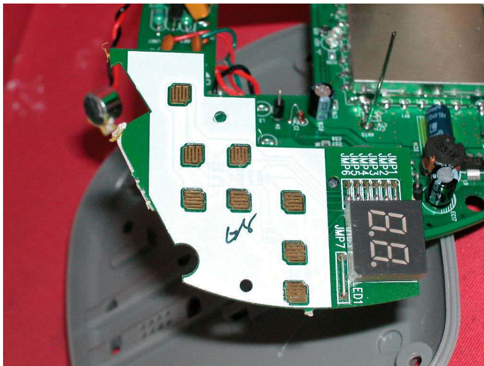
Base DAM keypad PCB front side
