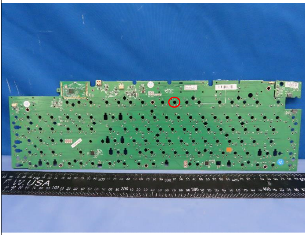
Difference 5 (PCB layout adjusted)
