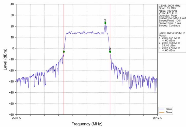
Band41 5MHz QPSK MCH 2605MHz RB 25 0 NTNV
