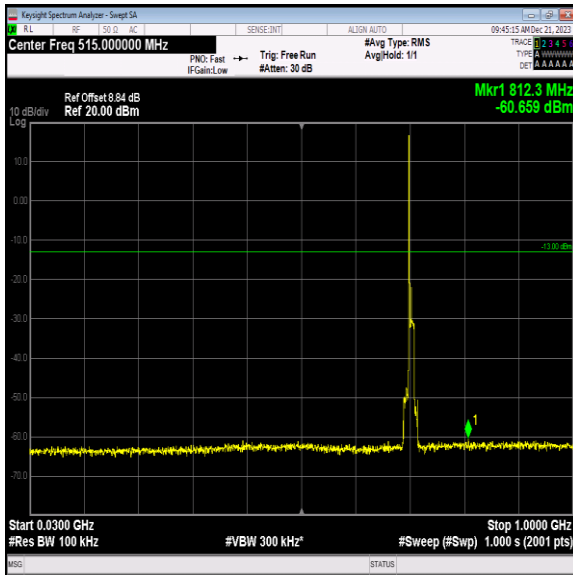
Band12_10MHz_16QAM_23130_1RB#0_30~1000_30~1000
