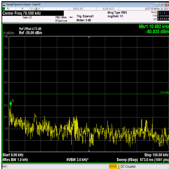
Band40_5MHz_QPSK_38775_1RB#0_0.009~0.15_0.009~0.15
