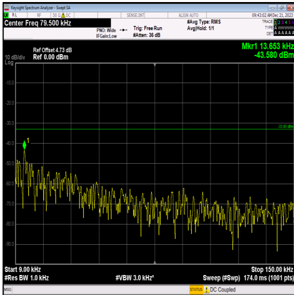
Band12_10MHz_64QAM_23095_1RB#0_0.009~0.15_0.009~0.15
