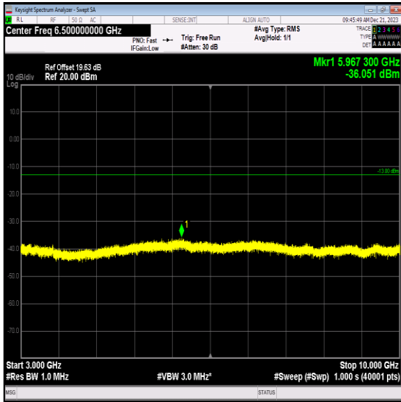
Band12_10MHz_16QAM_23130_1RB#0_3000~10000_3000~10000
