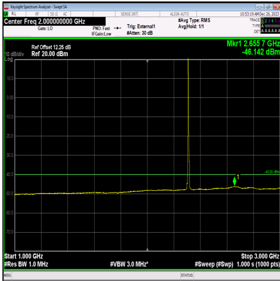
Band40_5MHz_QPSK_38750_1RB#0_1000~3000_1000~3000
