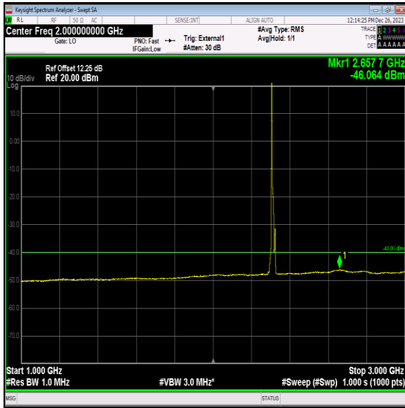
Band40_10MHz_QPSK_38750_1RB#0_1000~3000_1000~30 00
