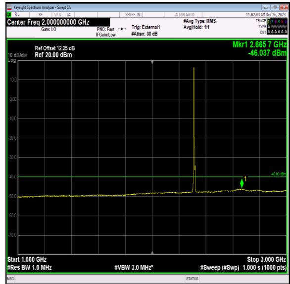
Band40_5MHz_64QAM_38775_1RB#0_1000~3000_1000~3000 00
