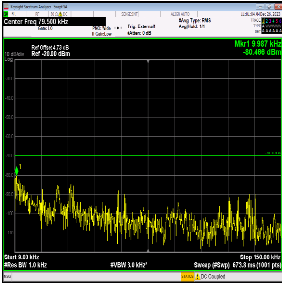
Band40_5MHz_64QAM_38775_1RB#0_0.009~0.15_0.009~0.15 15
