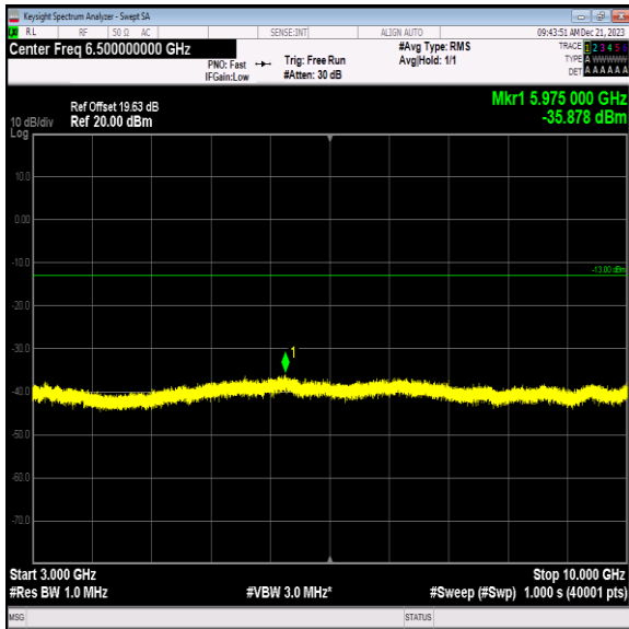
Band12_10MHz_64QAM_23095_1RB#0_3000~10000_3000~10000
