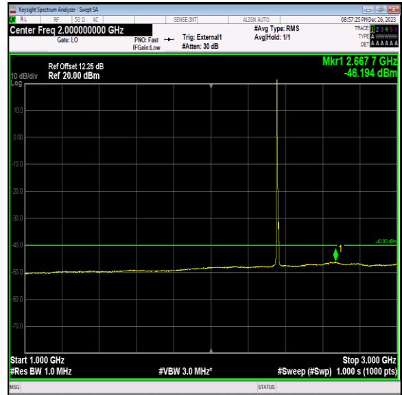
Band40_5MHz_QPSK_39225_1RB#0_1000~3000_1000~3000 0
