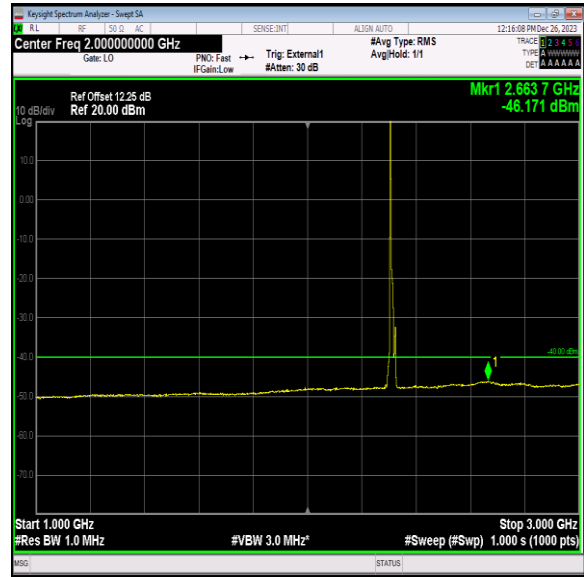
Band40_10MHz_16QAM_38750_1RB#0_1000~3000_1000~3000
