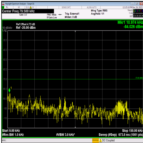
Band40_10MHz_16QAM_38750_1RB#0_0.009~0.15_0.009~ 0.15
