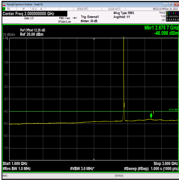
Band40_5MHz_QPSK_39200_1RB#0_1000~3000_1000~300 0
