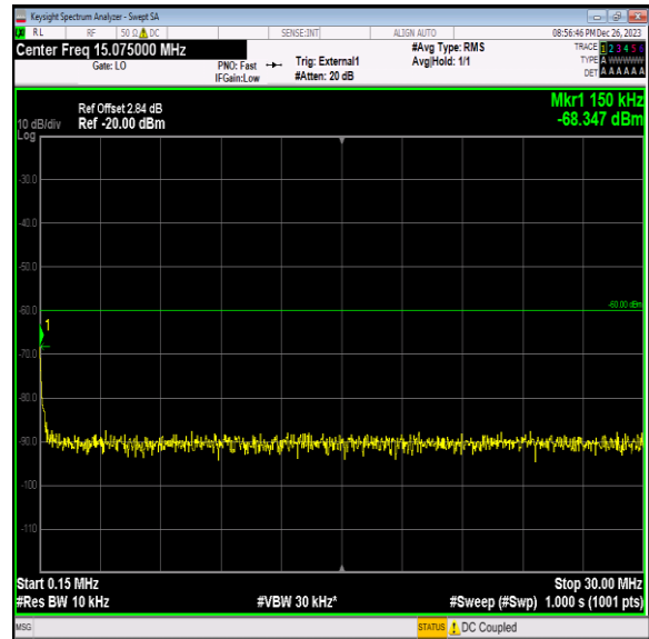
Band40_5MHz_QPSK_39225_1RB#0_0.15~30_0.15~30
