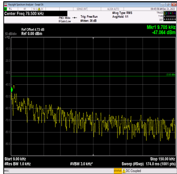
Band12_10MHz_64QAM_23130_1RB#0_0.009~0.15_0.009~0.15
