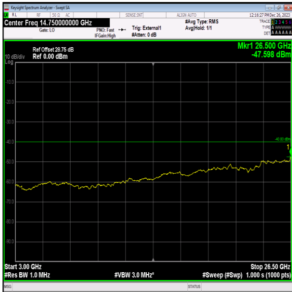
Band40_10MHz_16QAM_38750_1RB#0_3000~26500_3000~26500
