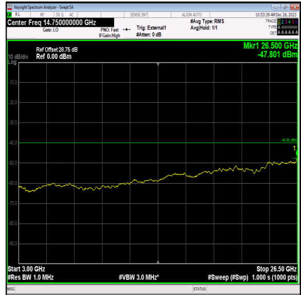
Band40_5MHz_QPSK_38750_1RB#0_3000~26500_3000~26500
