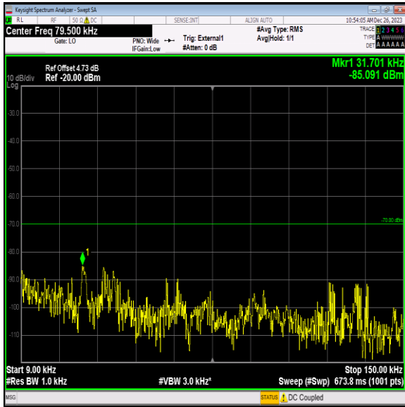
Band40_5MHz_16QAM_38750_1RB#0_0.009~0.15_0.009~0.15
