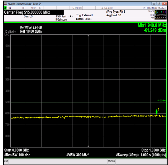
Band40_10MHz_QPSK_38750_1RB#0_30~1000_30~1000
