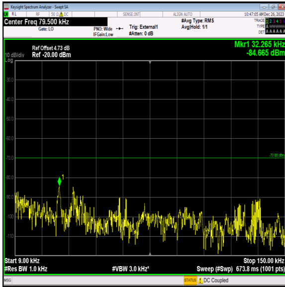
Band40_5MHz_QPSK_38725_1RB#0_0.009~0.15_0.009~0.1 5
