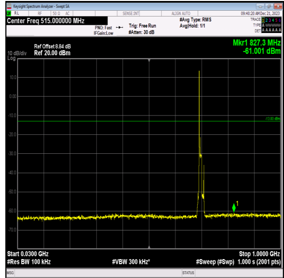
Band12_10MHz_64QAM_23060_1RB#0_30~1000_30~1000
