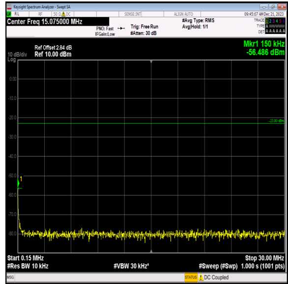
Band12_10MHz_16QAM_23130_1RB#0_0.15~30_0.15~30
