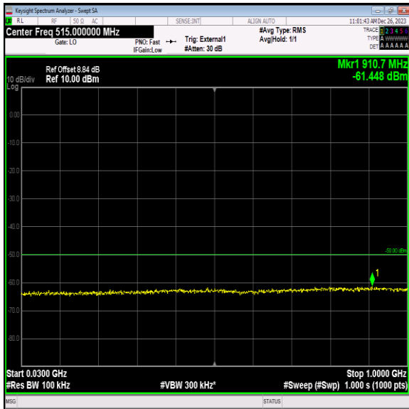
Band40_5MHz_64QAM_38775_1RB#0_30~1000_30~1000
