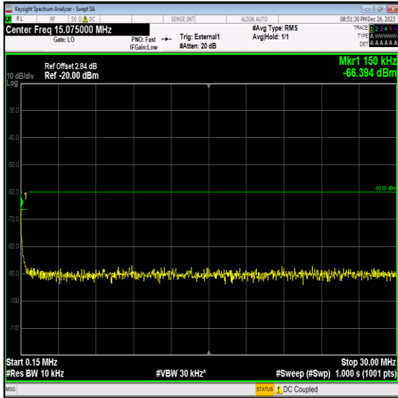
Band40_5MHz_QPSK_39200_1RB#0_0.15~30_0.15~30
