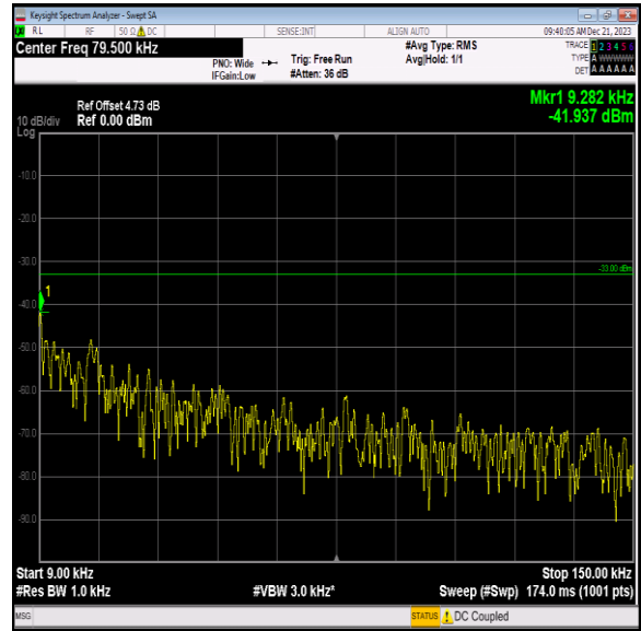
Band12_10MHz_64QAM_23060_1RB#0_0.009~0.15_0.009~0.15
