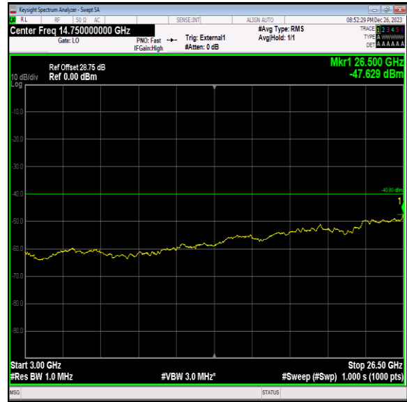
Band40_5MHz_QPSK_39200_1RB#0_3000~26500_3000~26 500
