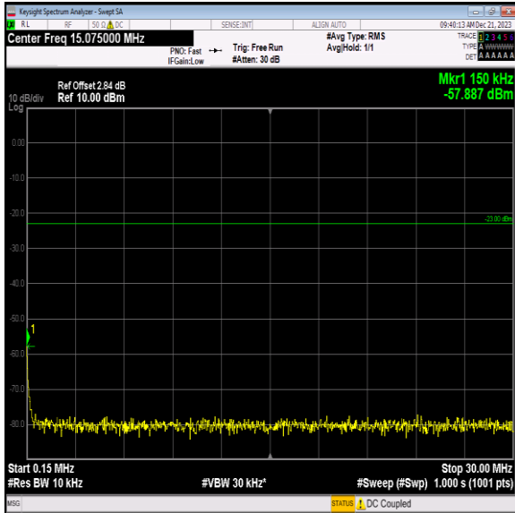
Band12_10MHz_64QAM_23060_1RB#0_0.15~30_0.15~30
