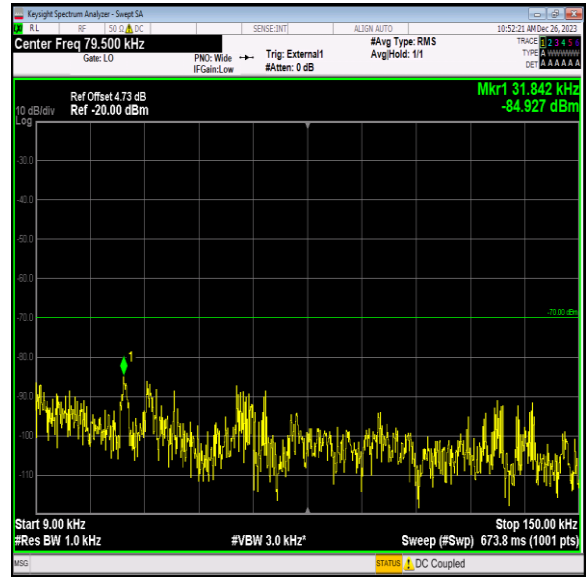
Band40_5MHz_QPSK_38750_1RB#0_0.009~0.15_0.009~0.1 5
