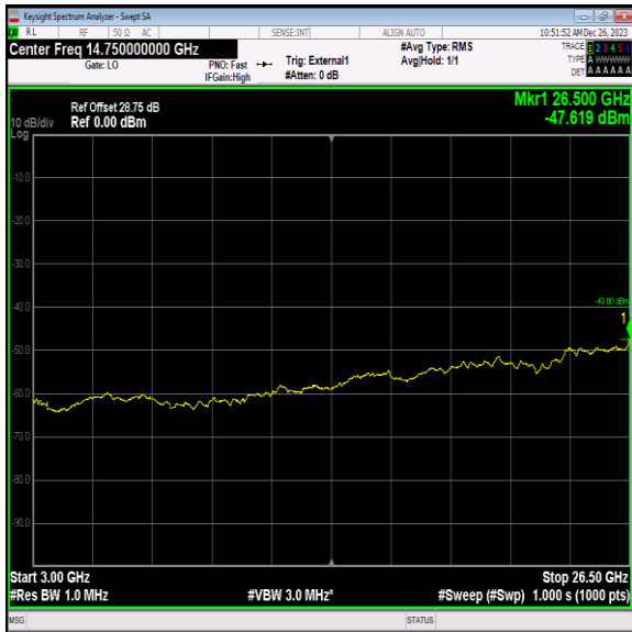
Band40_5MHz_64QAM_38725_1RB#0_3000~26500_3000~26500
