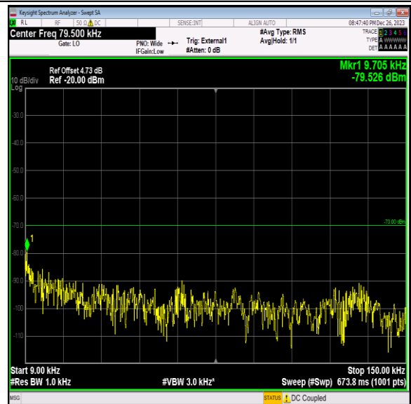
Band40_5MHz_16QAM_39175_1RB#0_0.009~0.15_0.009~0.15 15
