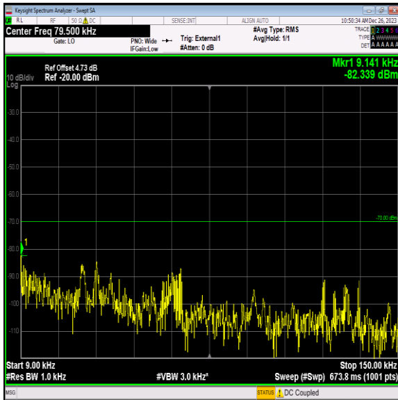
Band40_5MHz_64QAM_38725_1RB#0_0.009~0.15_0.009~0. 15
