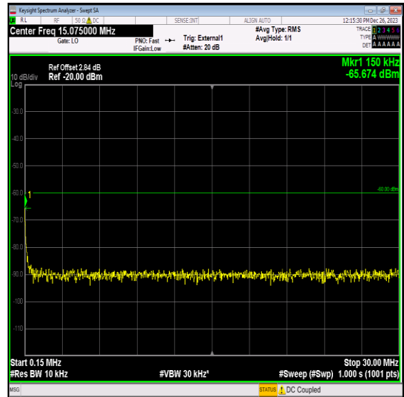
Band40_10MHz_16QAM_38750_1RB#0_0.15~30_0.15~30
