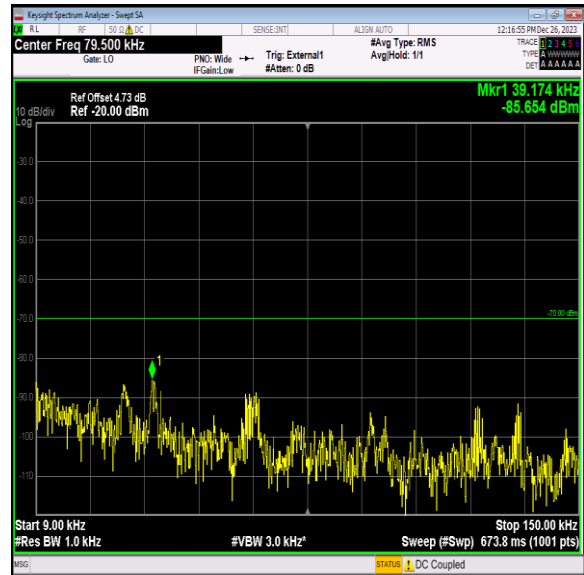
Band40_10MHz_64QAM_38750_1RB#0_0.009~0.15_0.009~0.15
