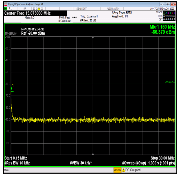
Band40_5MHz_QPSK_38725_1RB#0_0.15~30_0.15~30
