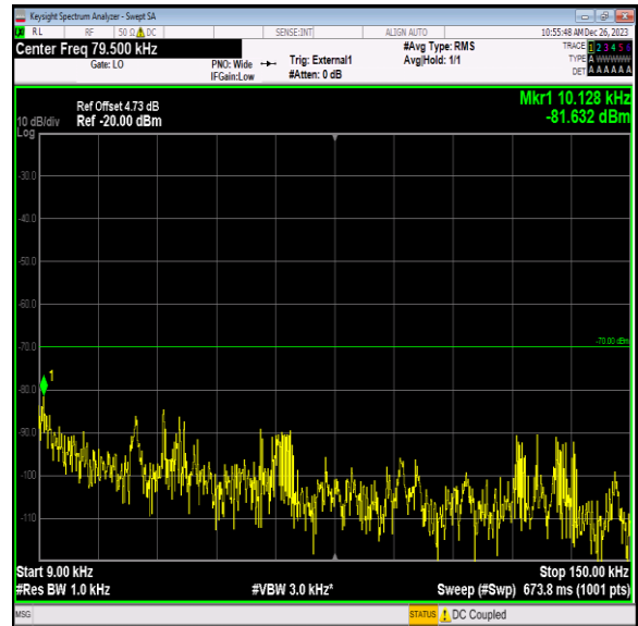
Band40_5MHz_64QAM_38750_1RB#0_0.009~0.15_0.009~0.15
