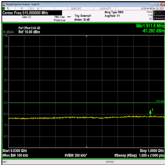
Band40_5MHz_16QAM_38750_1RB#0_30~1000_30~1000
