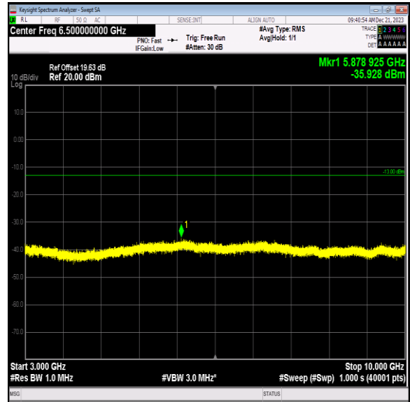
Band12_10MHz_64QAM_23060_1RB#0_3000~10000_3000~10000
