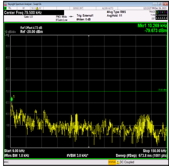
Band40_10MHz_QPSK_38750_1RB#0_0.009~0.15_0.009~0.15
