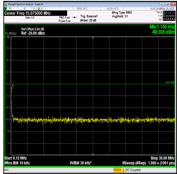
Band40_5MHz_64QAM_38775_1RB#0_0.15~30_0.15~30
