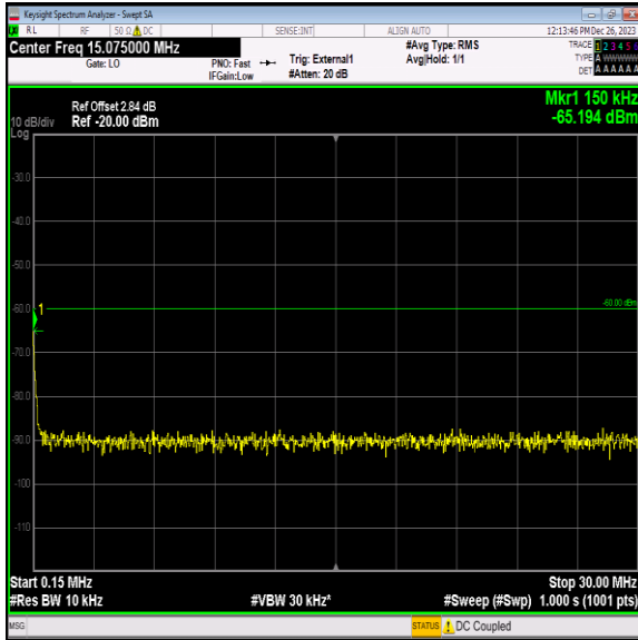
Band40_10MHz_QPSK_38750_1RB#0_0.15~30_0.15~30
