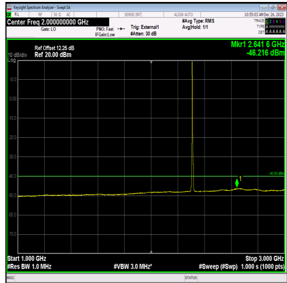
Band40_5MHz_16QAM_38750_1RB#0_1000~3000_1000~3000
