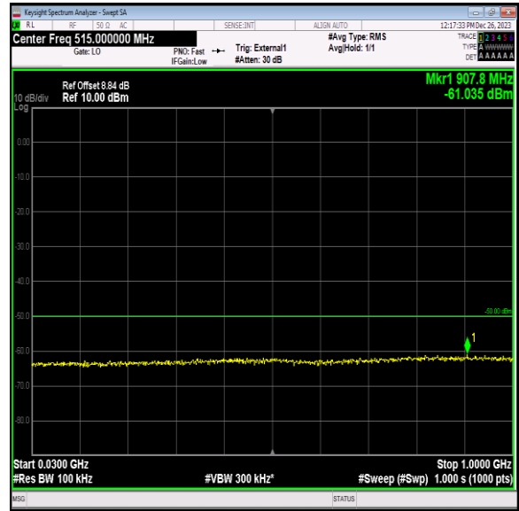
Band40_10MHz_64QAM_38750_1RB#0_30~1000_30~1000
