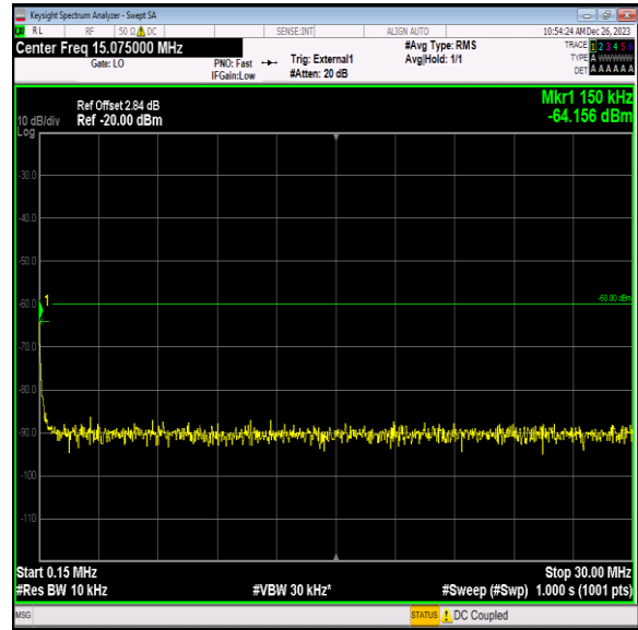
Band40_5MHz_16QAM_38750_1RB#0_0.15~30_0.15~30
