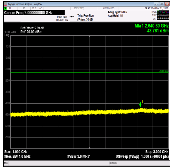
Band12_10MHz_64QAM_23095_1RB#0_1000~3000_1000~3000
