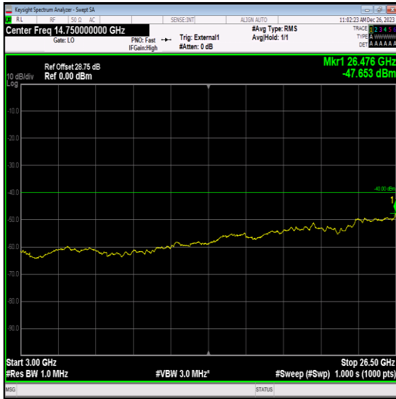
Band40_5MHz_64QAM_38775_1RB#0_3000~26500_3000~26500
