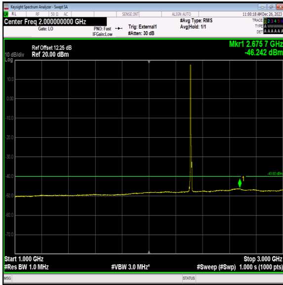
Band40_5MHz_16QAM_38775_1RB#0_1000~3000_1000~30 00
