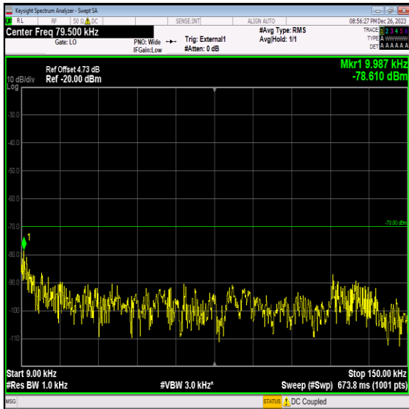
Band40_5MHz_QPSK_39225_1RB#0_0.009~0.15_0.009~0.1 5
