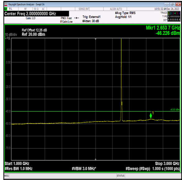
Band40_5MHz_64QAM_38725_1RB#0_1000~3000_1000~3000
