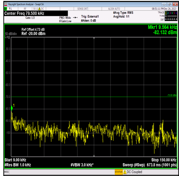
Band40_5MHz_QPSK_39200_1RB#0_0.009~0.15_0.009~0.1 5
