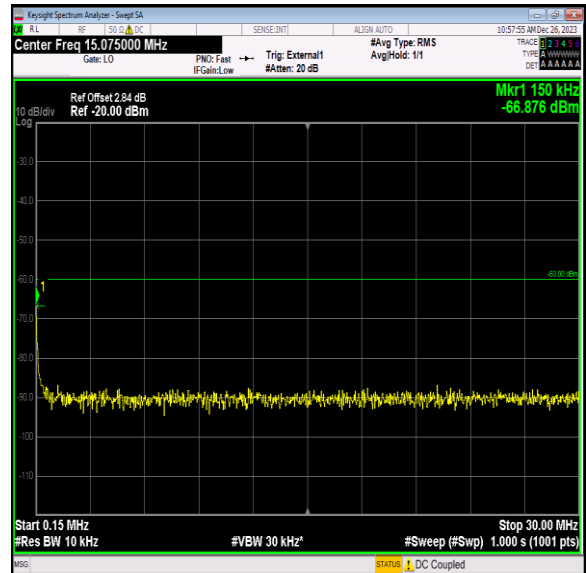
Band40_5MHz_QPSK_38775_1RB#0_0.15~30_0.15~30
