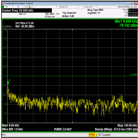
Band40_5MHz_QPSK_39175_1RB#0_0.009~0.15_0.009~0.1 5
