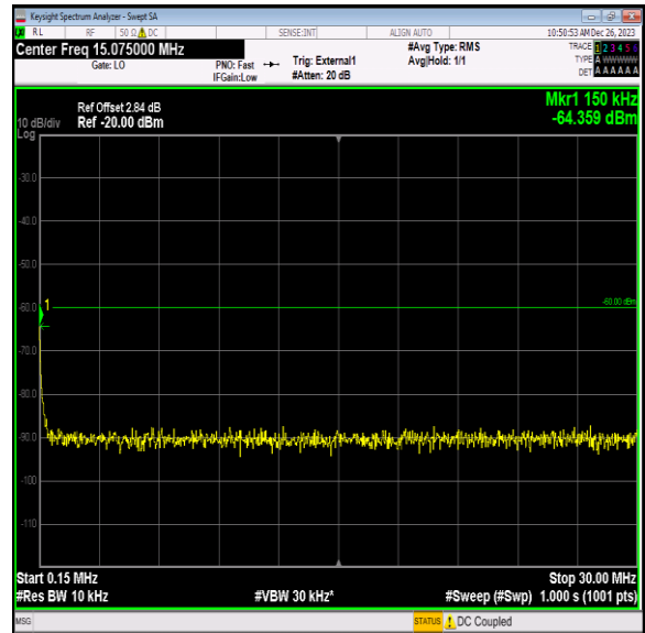
Band40_5MHz_64QAM_38725_1RB#0_0.15~30_0.15~30
