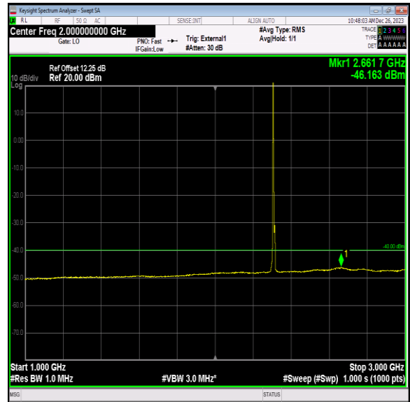
Band40_5MHz_QPSK_38725_1RB#0_1000~3000_1000~300 0
