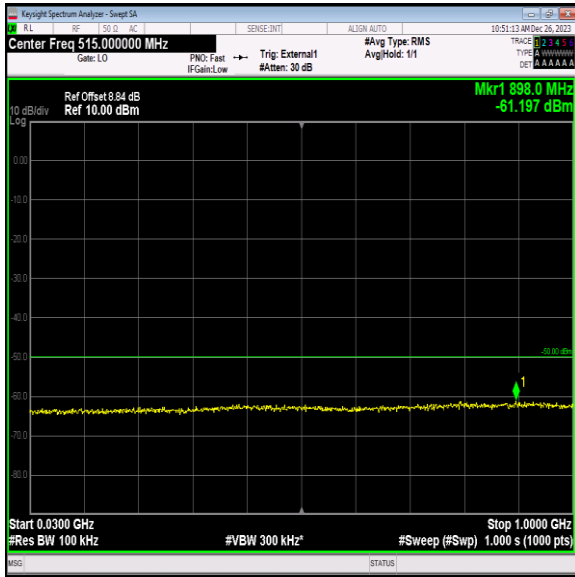
Band40_5MHz_64QAM_38725_1RB#0_30~1000_30~1000
