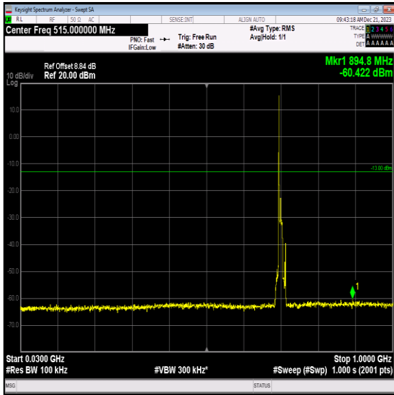
Band12_10MHz_64QAM_23095_1RB#0_30~1000_30~1000
