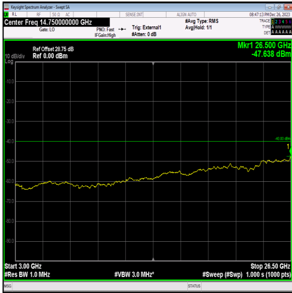
Band40_5MHz_QPSK_39175_1RB#0_3000~26500_3000~26 500
