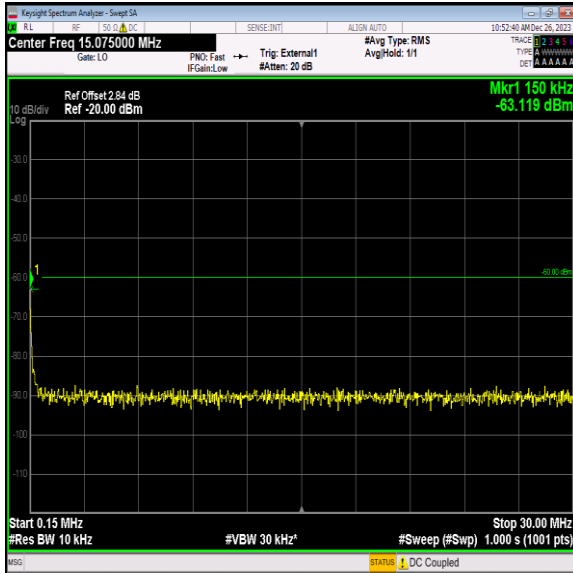
Band40_5MHz_QPSK_38750_1RB#0_0.15~30_0.15~30
