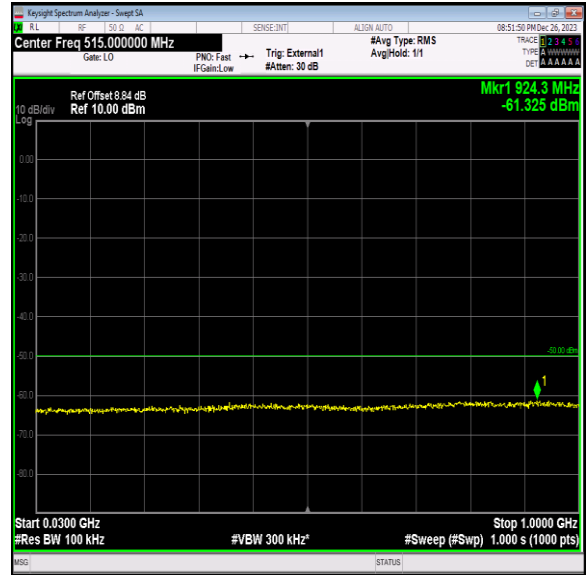
Band40_5MHz_QPSK_39200_1RB#0_30~1000_30~1000
