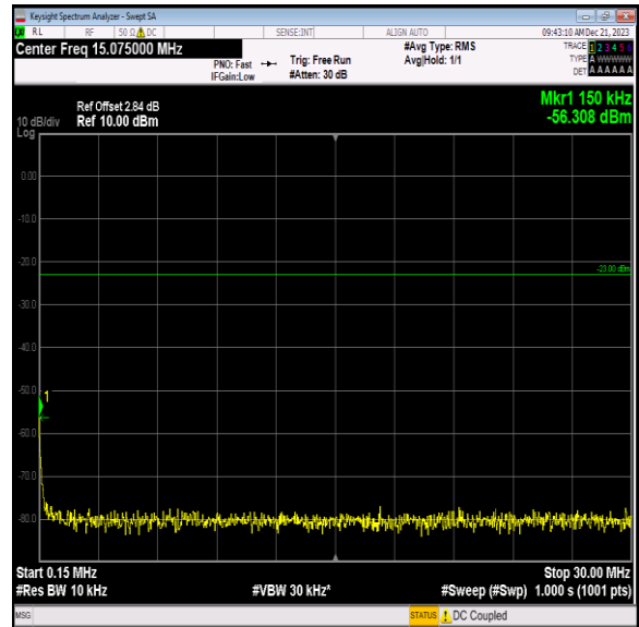
Band12_10MHz_64QAM_23095_1RB#0_0.15~30_0.15~30
