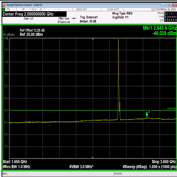
Band40_10MHz_64QAM_38750_1RB#0_1000~3000_1000~3000
