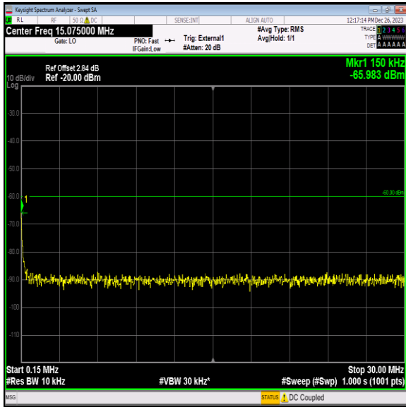
Band40_10MHz_64QAM_38750_1RB#0_0.15~30_0.15~30
