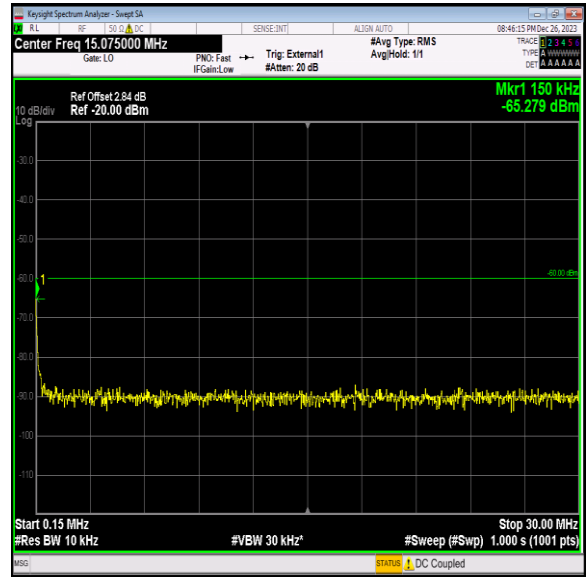
Band40_5MHz_QPSK_39175_1RB#0_0.15~30_0.15~30
