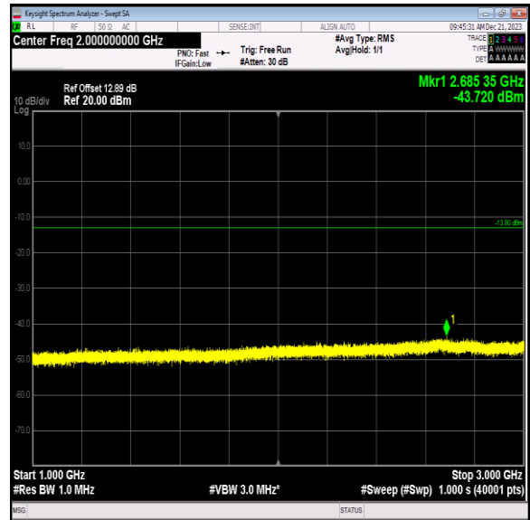
Band12_10MHz_16QAM_23130_1RB#0_1000~3000_1000~3000
