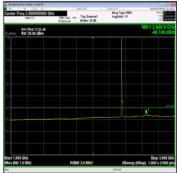
Band40_5MHz_QPSK_39175_1RB#0_1000~3000_1000~300 0
