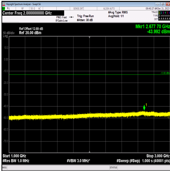
Band12_10MHz_64QAM_23060_1RB#0_1000~3000_1000~3000
