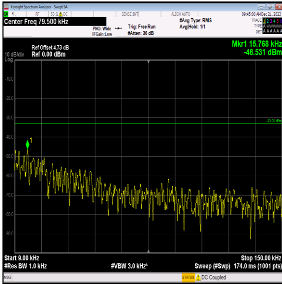
Band12_10MHz_16QAM_23130_1RB#0_0.009~0.15_0.009~0.15
