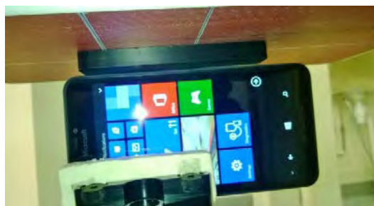
Photo of the device positioned for WR mode measurement – right edge facing phantom. The spacer was removed before the start of the measurements
