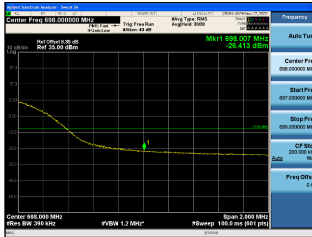
Band71-20MHz-16QAM-133222-100RB#0
