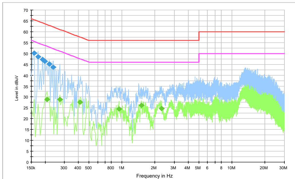
Fig.B.8.1 AC Powerline Conducted Emission- bluetooth
