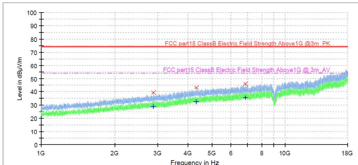
Figure 5: Spectral Diagrams, Radiated Emission, 1GHz-18GHz, Horizontal polarization
