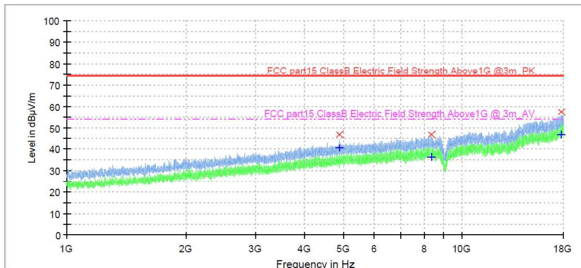
Figure 6: Spectral Diagrams, Radiated Emission, 1GHz-18GHz, Vertical polarization
