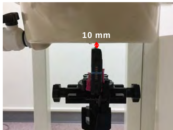
Fig.11 EUT Right side to flat phantom
