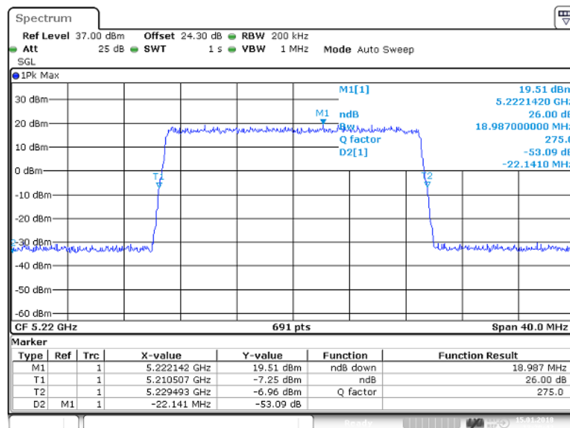
Figure 42 Occupied Bandwidth – 64QAM (5220.0 MHz) (20MHz Channel BW)
