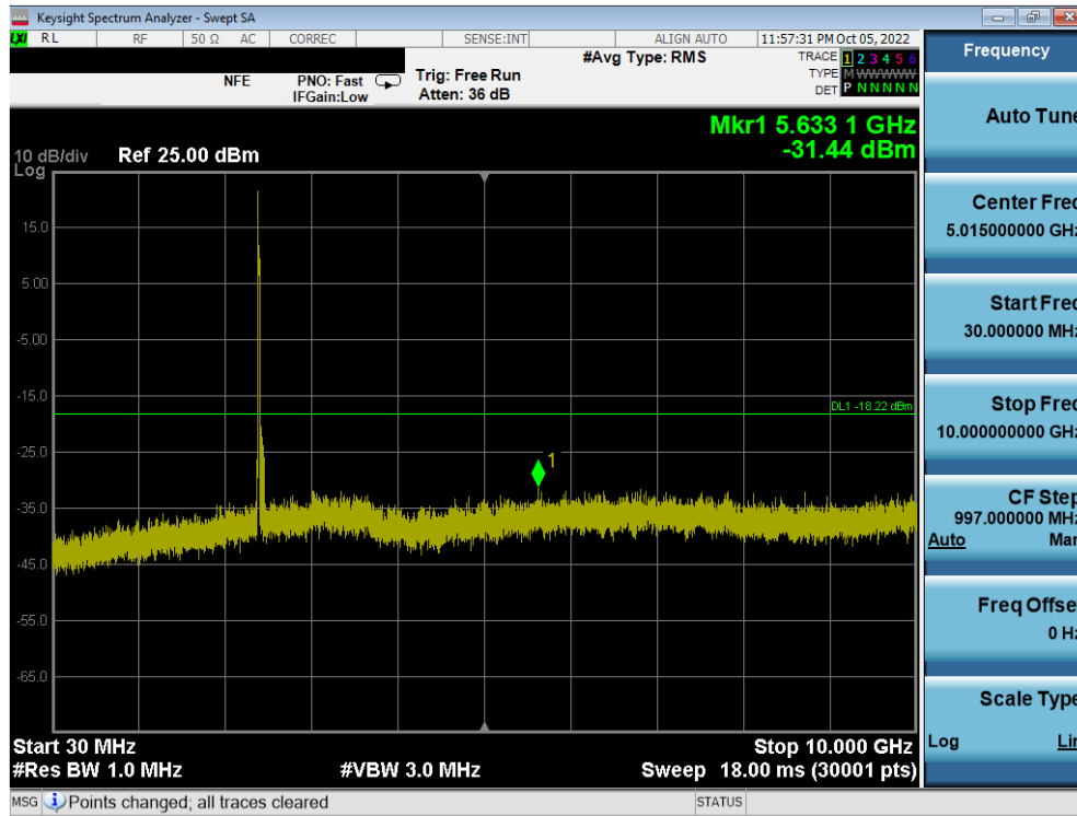
Plot 7-58. Conducted Spurious Plot SISO ANT2 (802.11ax OFDMA – 26 Tones – Ch. 1)
