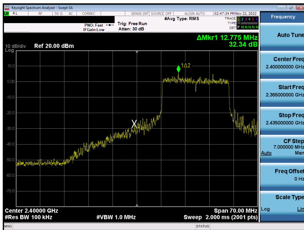
Plot 7-54. Band Edge Plot MIMO ANT2 (802.11ax OFDMA – 242 Tones – Ch. 2)
