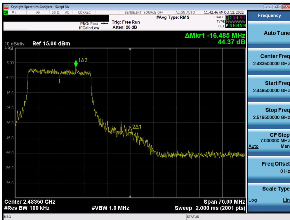
Plot 7-43. Band Edge Plot SISO ANT2 (802.11ax OFDMA – 242 Tones – Ch. 11)
