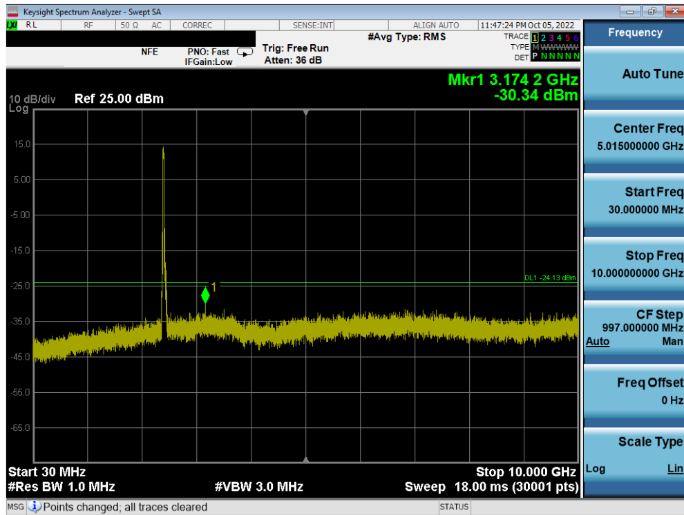
Plot 7-76. Conducted Spurious Plot MIMO ANT1 (802.11ax OFDMA – 242 Tones – Ch. 1)
