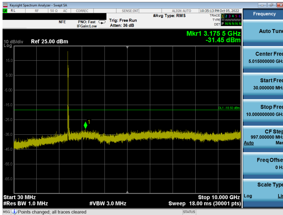
Plot 7-82. Conducted Spurious Plot MIMO ANT2 (802.11ax OFDMA – 26 Tones – Ch. 1)
