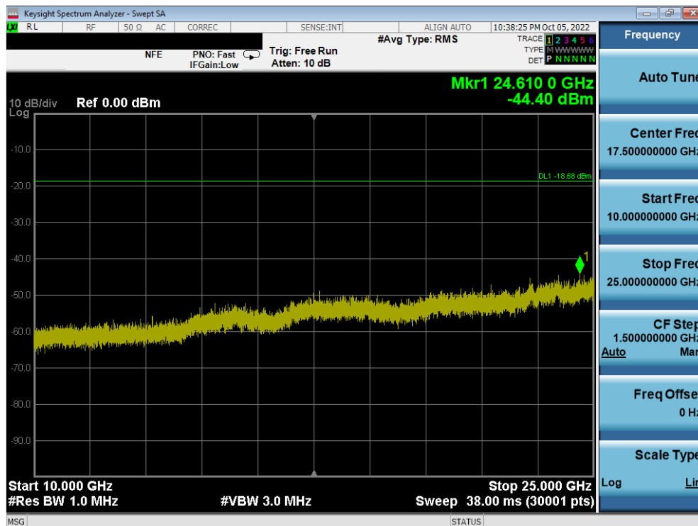
Plot 7-87. Conducted Spurious Plot MIMO ANT2 (802.11ax OFDMA – 26 Tones – Ch. 11)
