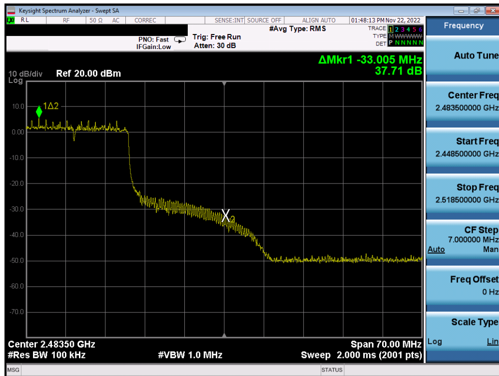
Plot 7-42. Band Edge Plot SISO ANT2 (802.11ax OFDMA – 242 Tones – Ch. 10)
