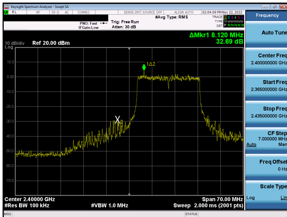
Plot 7-53. Band Edge Plot MIMO ANT2 (802.11ax OFDMA – 242 Tones – Ch. 1)
