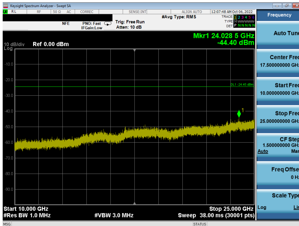
Plot 7-69. Conducted Spurious Plot SISO ANT2 (802.11ax OFDMA – 242 Tones – Ch. 11)
