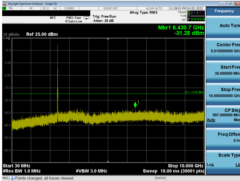
Plot 7-70. Conducted Spurious Plot MIMO ANT1 (802.11ax OFDMA – 26 Tones – Ch. 1)
