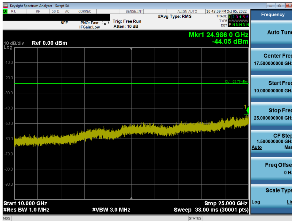
Plot 7-89. Conducted Spurious Plot MIMO ANT2 (802.11ax OFDMA – 242 Tones – Ch. 1)
