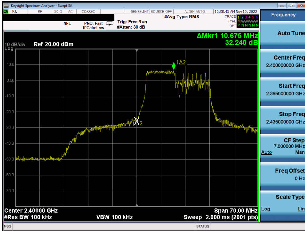
Plot 7-44. Band Edge Plot MIMO ANT1 (802.11ax OFDMA – 106 Tones – Ch. 1)
