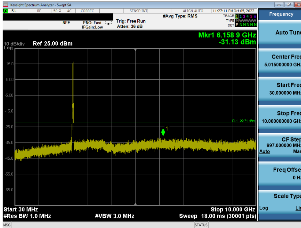
Plot 7-90. Conducted Spurious Plot MIMO ANT2 (802.11ax OFDMA – 242 Tones – Ch. 6)
