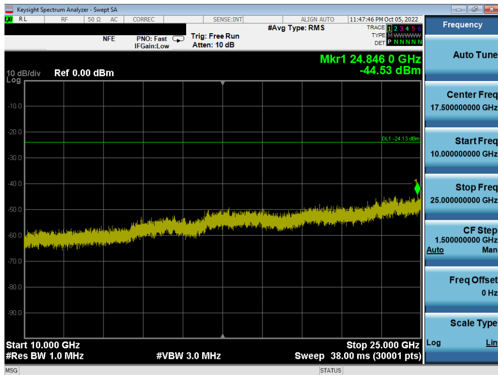
Plot 7-77. Conducted Spurious Plot MIMO ANT1 (802.11ax OFDMA – 242 Tones – Ch. 1)
