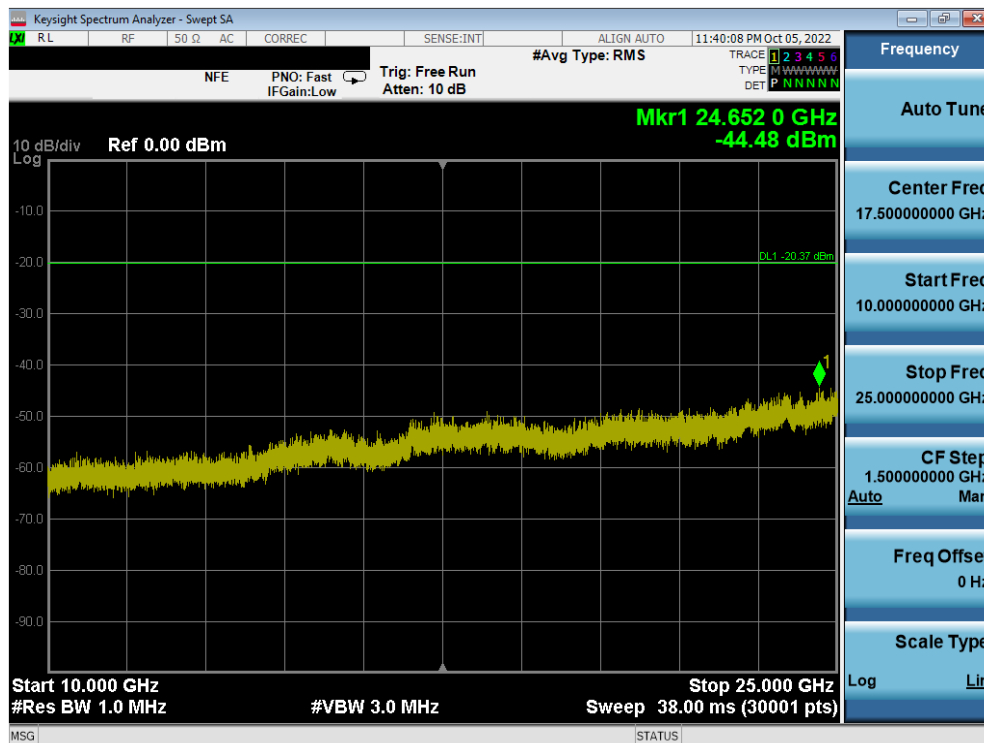
Plot 7-73. Conducted Spurious Plot MIMO ANT1 (802.11ax OFDMA – 26 Tones – Ch. 6)
