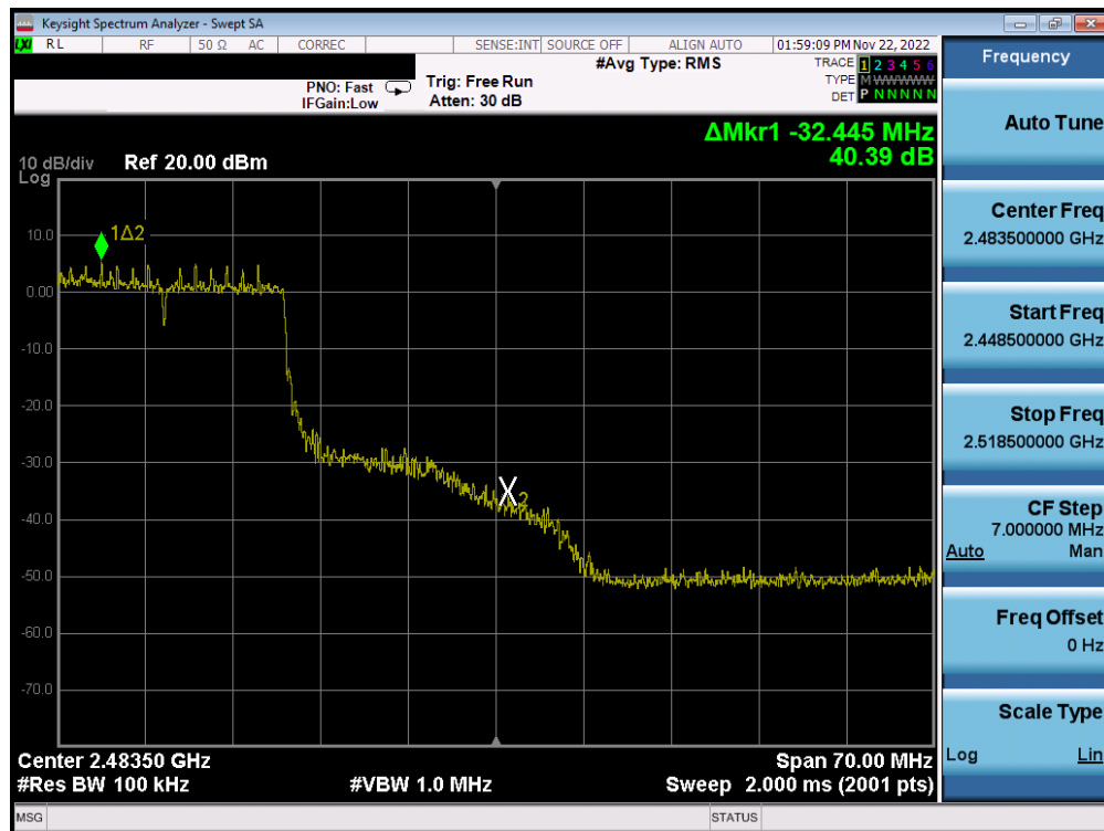
Plot 7-49. Band Edge Plot MIMO ANT1 (802.11ax OFDMA – 242 Tones – Ch. 10)
