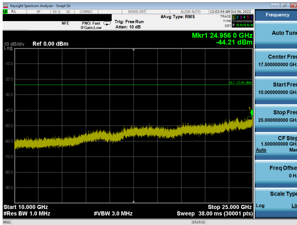
Plot 7-65. Conducted Spurious Plot SISO ANT2 (802.11ax OFDMA – 242 Tones – Ch. 1)
