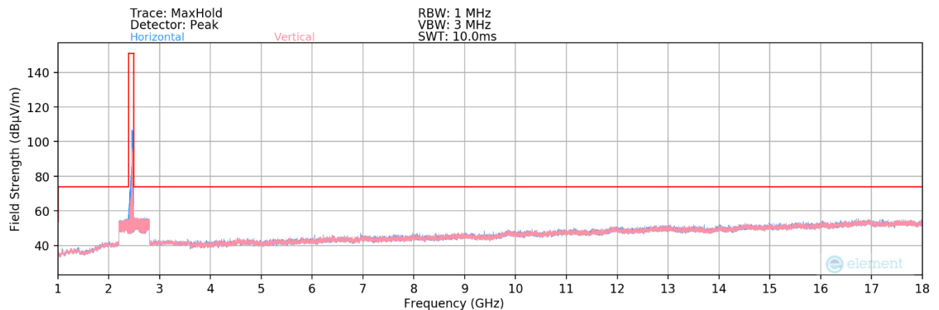
Plot 7-99. Radiated Spurious Plot above 1GHz SISO ANT2 (802.11ax OFDMA – 242 Tones – Ch. 11)
