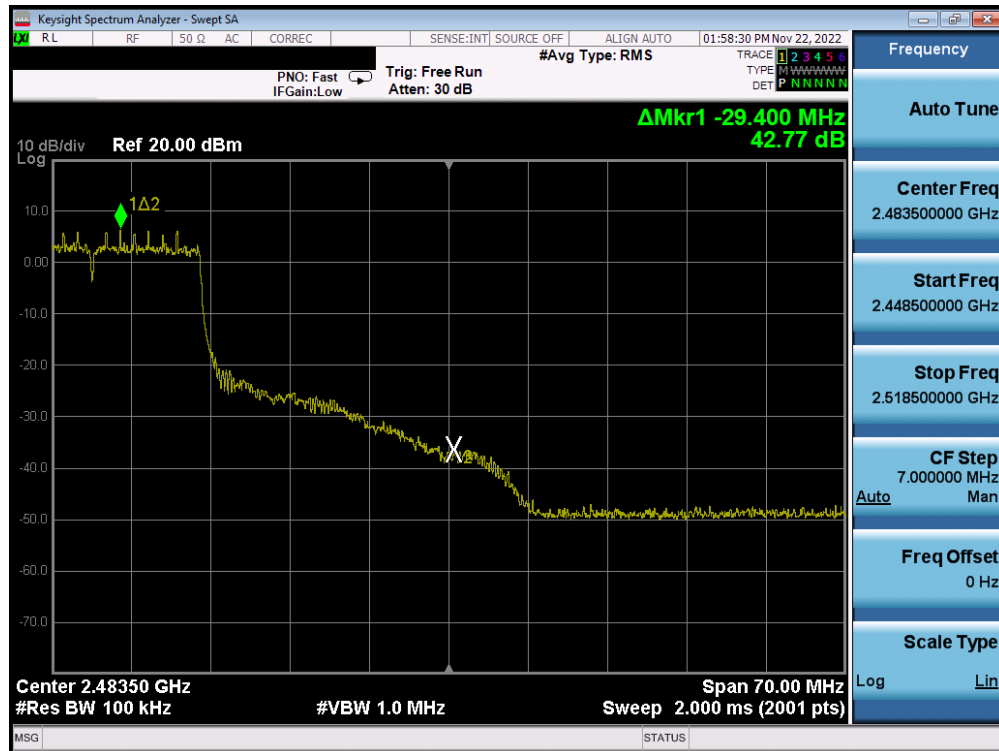
Plot 7-48. Band Edge Plot MIMO ANT1 (802.11ax OFDMA – 242 Tones – Ch. 9)
