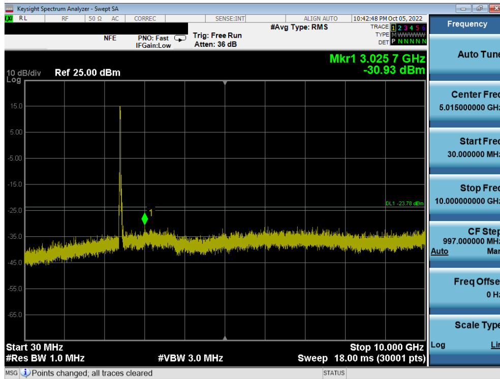
Plot 7-88. Conducted Spurious Plot MIMO ANT2 (802.11ax OFDMA – 242 Tones – Ch. 1)
