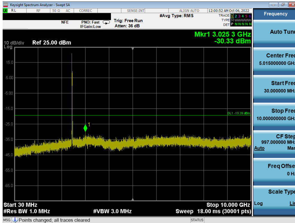
Plot 7-62. Conducted Spurious Plot SISO ANT2 (802.11ax OFDMA – 26 Tones – Ch. 11)
