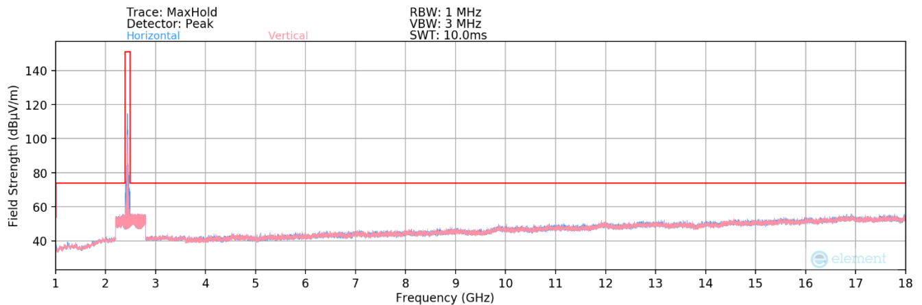
Plot 7-95. Radiated Spurious Plot above 1GHz SISO ANT2 (802.11ax OFDMA – 26 Tones – Ch. 6)
