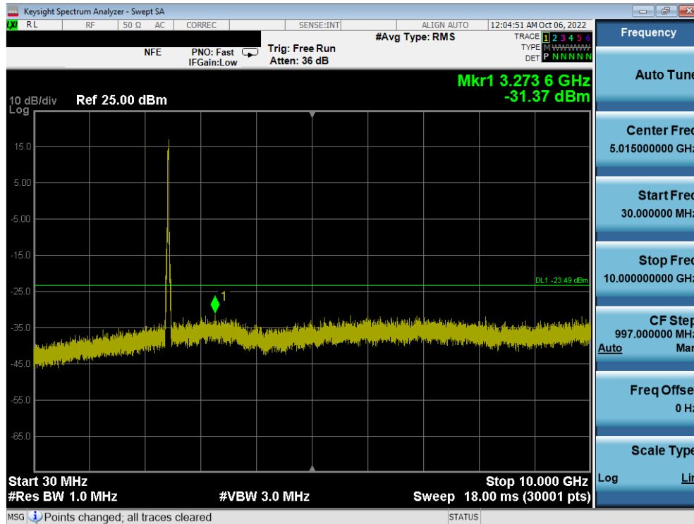
Plot 7-66. Conducted Spurious Plot SISO ANT2 (802.11ax OFDMA – 242 Tones – Ch. 6)
