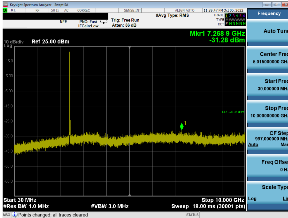
Plot 7-72. Conducted Spurious Plot MIMO ANT1 (802.11ax OFDMA – 26 Tones – Ch. 6)
