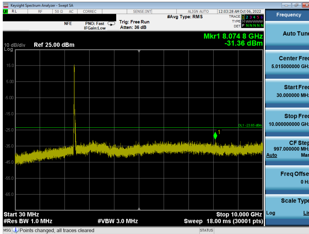
Plot 7-64. Conducted Spurious Plot SISO ANT2 (802.11ax OFDMA – 242 Tones – Ch. 1)
