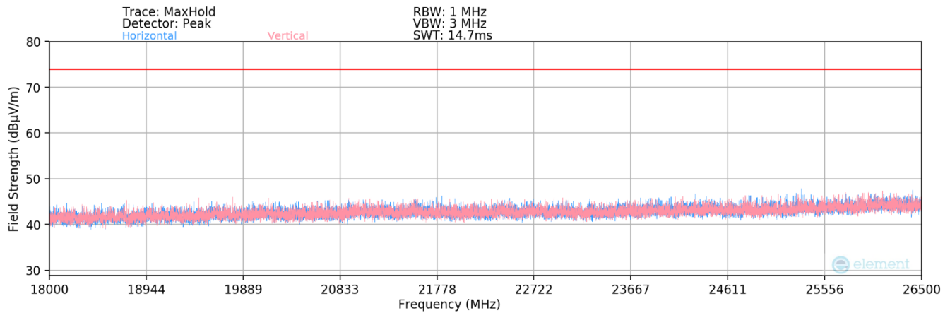
Plot 7-101. Radiated Spurious Plot above 18GHz SISO ANT2 (802.11ax OFDMA – 242 Tones)
