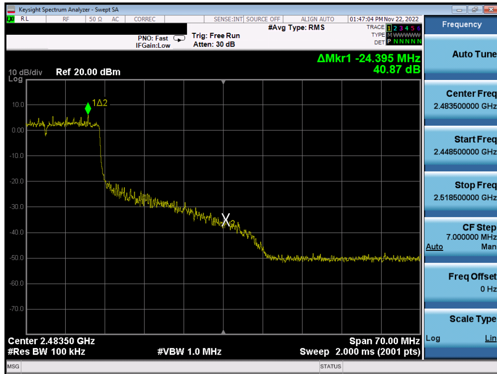
Plot 7-41. Band Edge Plot SISO ANT2 (802.11ax OFDMA – 242 Tones – Ch. 9)
