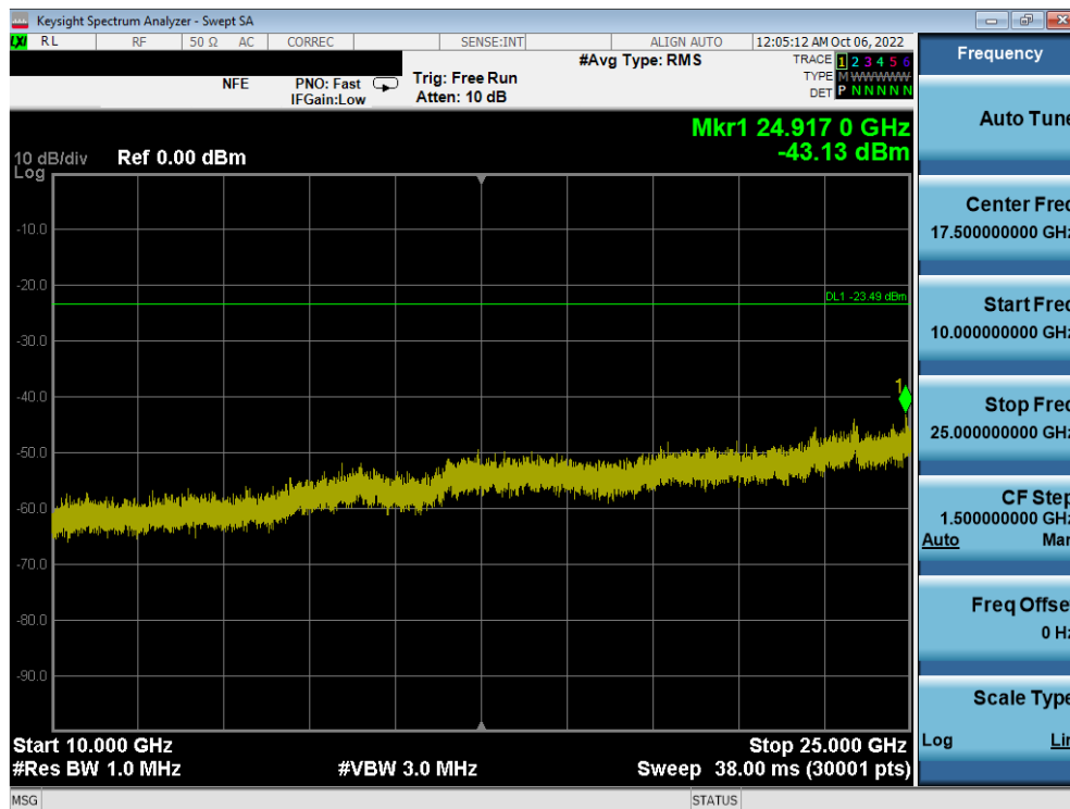
Plot 7-67. Conducted Spurious Plot SISO ANT2 (802.11ax OFDMA – 242 Tones – Ch. 6)
