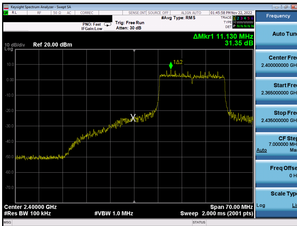
Plot 7-40. Band Edge Plot SISO ANT2 (802.11ax OFDMA – 242 Tones – Ch. 2)
