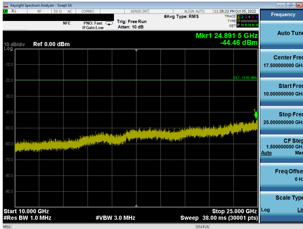
Plot 7-71. Conducted Spurious Plot MIMO ANT1 (802.11ax OFDMA – 26 Tones – Ch. 1)
