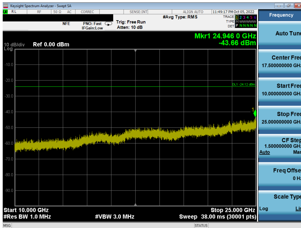
Plot 7-79. Conducted Spurious Plot MIMO ANT1 (802.11ax OFDMA – 242 Tones – Ch. 6)
