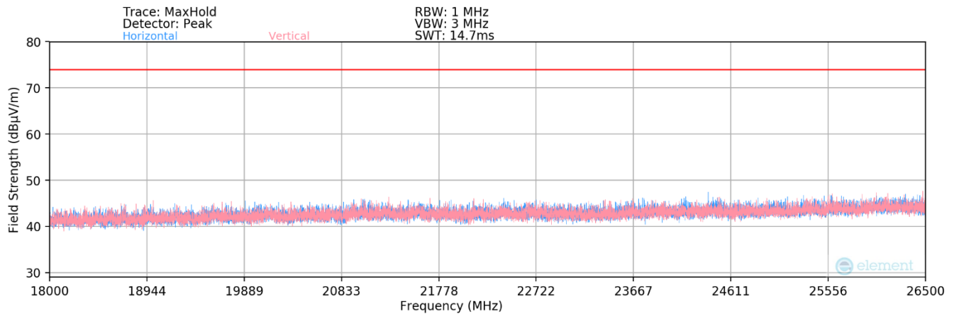
Plot 7-100. Radiated Spurious Plot above 18GHz SISO ANT2 (802.11ax OFDMA – 26 Tones)
