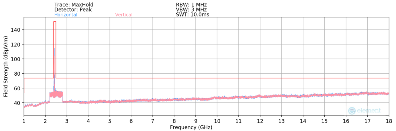
Plot 7-94. Radiated Spurious Plot above 1GHz SISO ANT2 (802.11ax OFDMA – 26 Tones – Ch. 1)
