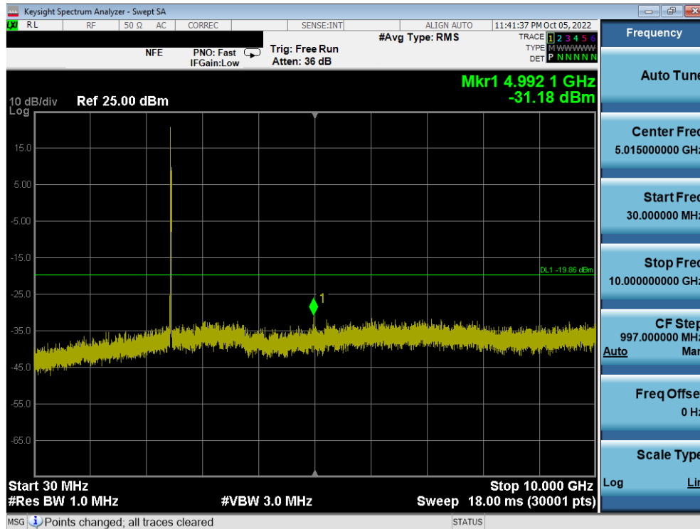
Plot 7-74. Conducted Spurious Plot MIMO ANT1 (802.11ax OFDMA – 26 Tones – Ch. 11)
