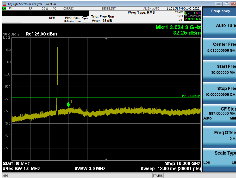
Plot 7-80. Conducted Spurious Plot MIMO ANT1 (802.11ax OFDMA – 242 Tones – Ch. 11)
