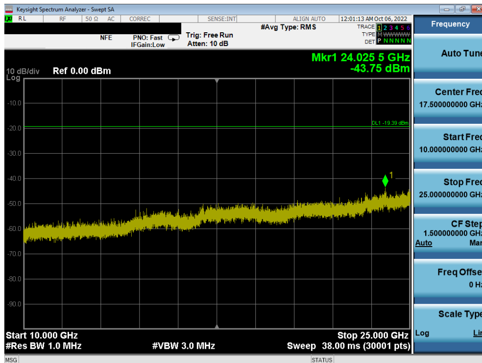
Plot 7-63. Conducted Spurious Plot SISO ANT2 (802.11ax OFDMA – 26 Tones – Ch. 11)
