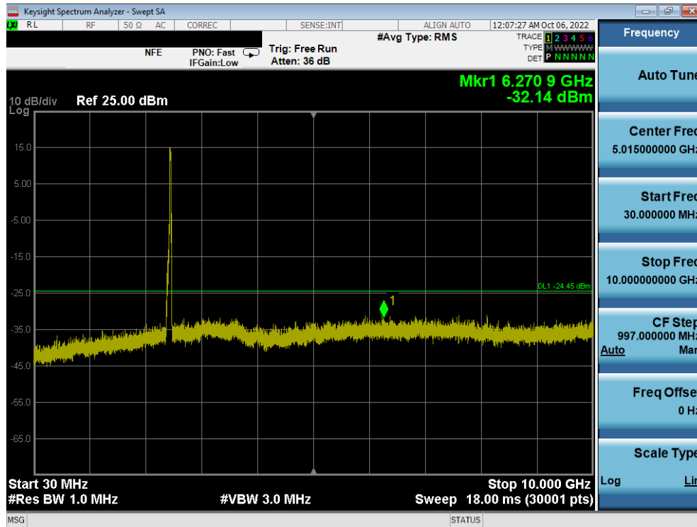
Plot 7-68. Conducted Spurious Plot SISO ANT2 (802.11ax OFDMA – 242 Tones – Ch. 11)
