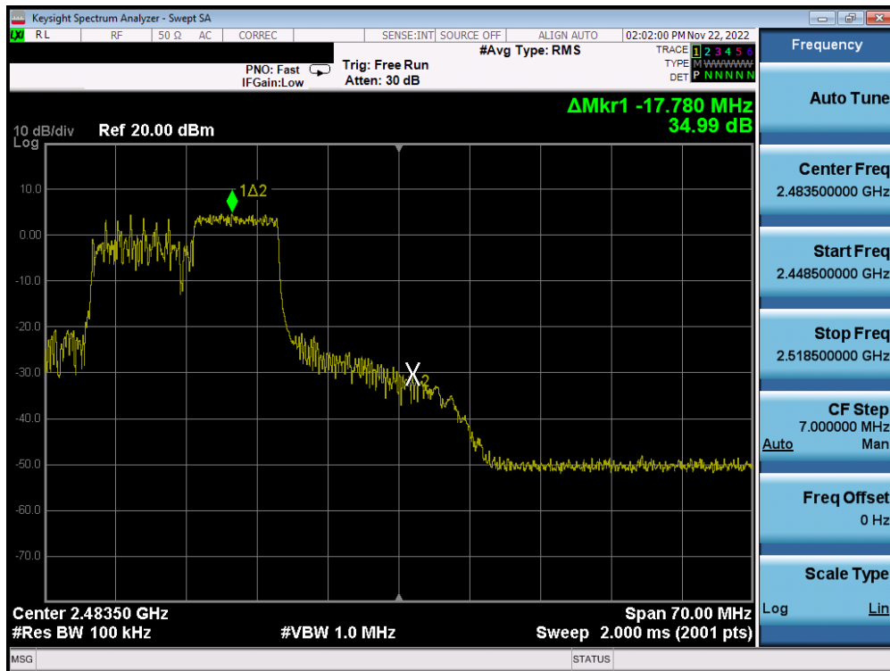
Plot 7-52. Band Edge Plot MIMO ANT2 (802.11ax OFDMA – 106 Tones – Ch. 11)
