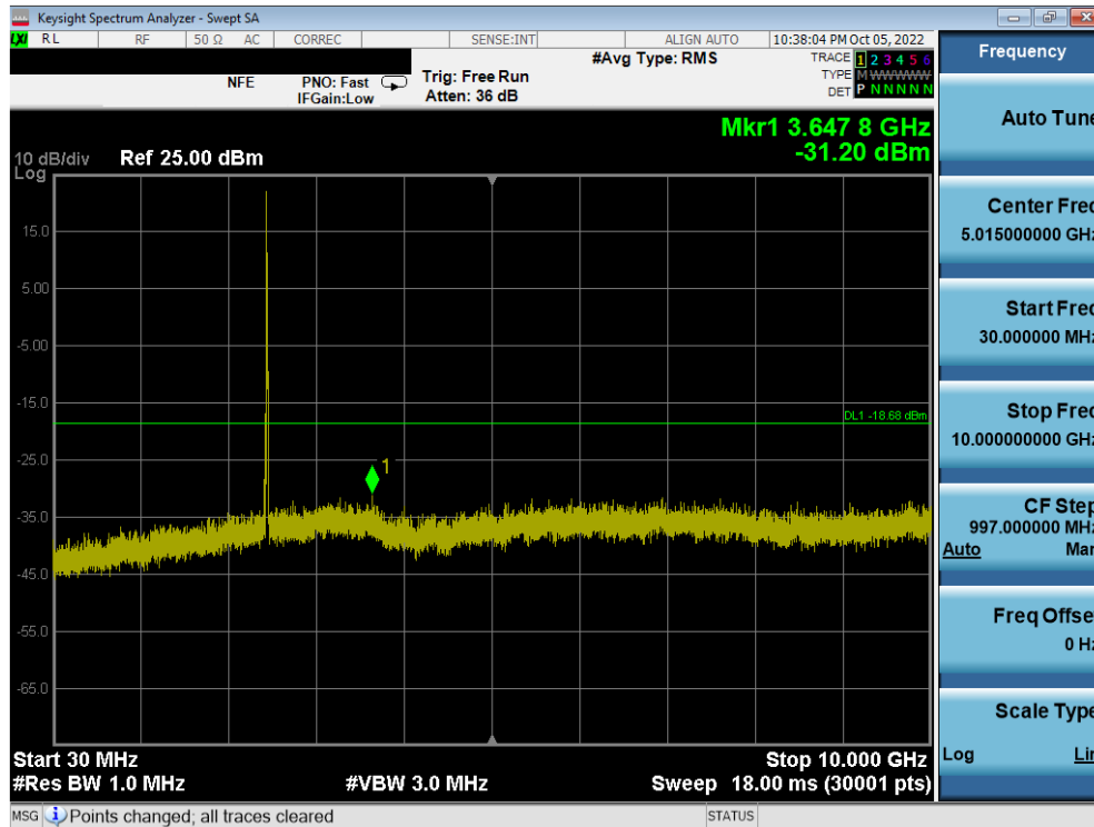
Plot 7-86. Conducted Spurious Plot MIMO ANT2 (802.11ax OFDMA – 26 Tones – Ch. 11)
