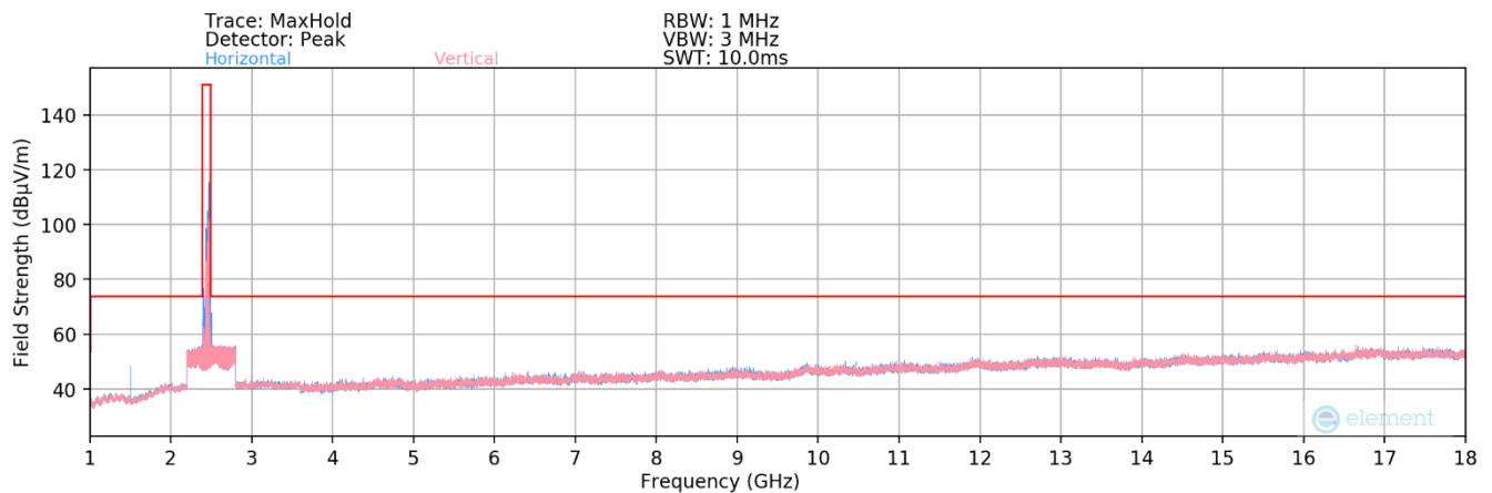
Plot 7-96. Radiated Spurious Plot above 1GHz SISO ANT2 (802.11ax OFDMA – 26 Tones – Ch. 11)
