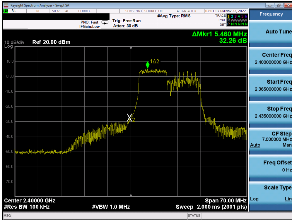
Plot 7-51. Band Edge Plot MIMO ANT2 (802.11ax OFDMA – 106 Tones – Ch. 1)
