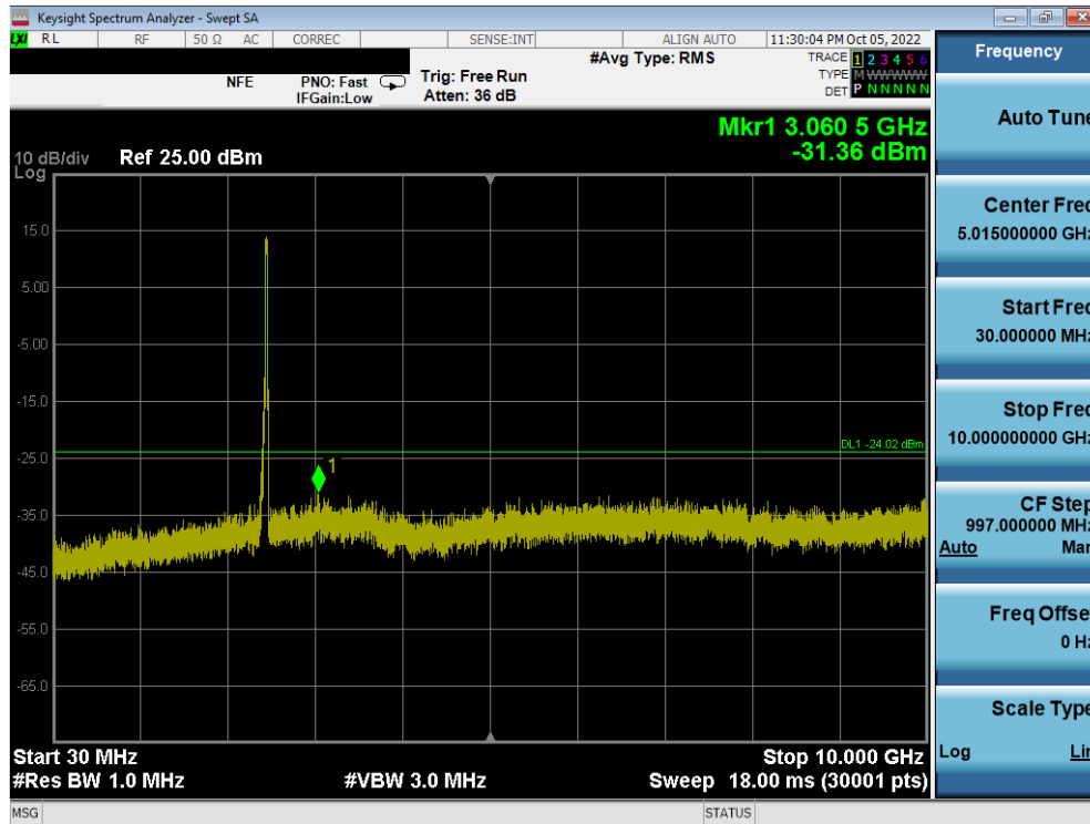
Plot 7-92. Conducted Spurious Plot MIMO ANT2 (802.11ax OFDMA – 242 Tones – Ch. 11)
