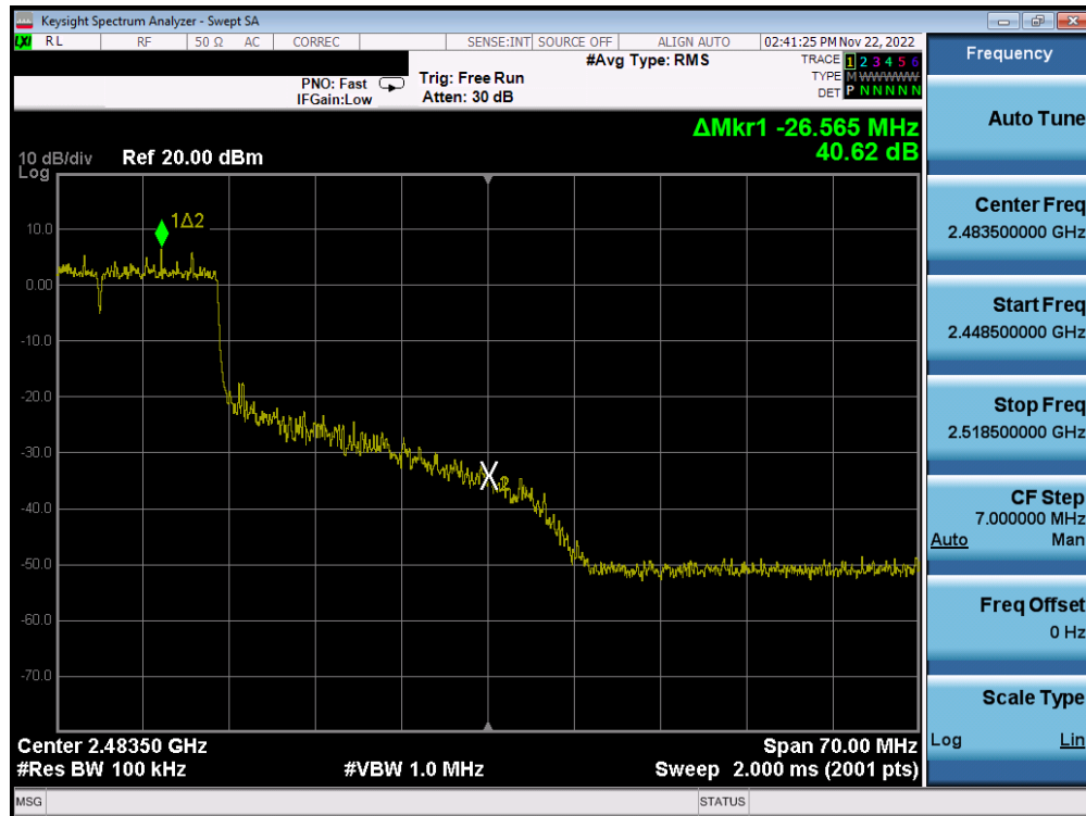
Plot 7-55. Band Edge Plot MIMO ANT2 (802.11ax OFDMA – 242 Tones – Ch. 9)
