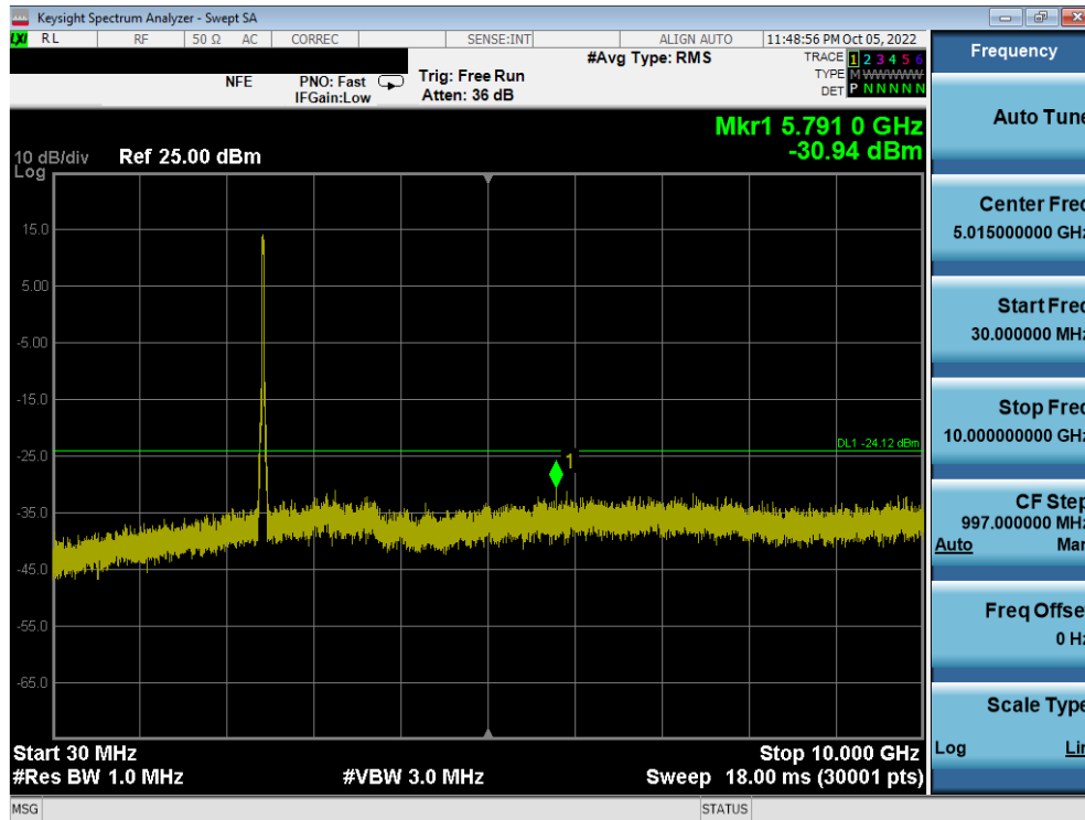
Plot 7-78. Conducted Spurious Plot MIMO ANT1 (802.11ax OFDMA – 242 Tones – Ch. 6)
