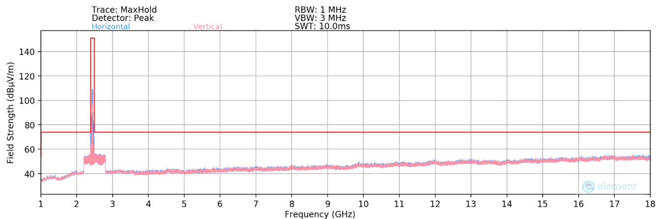
Plot 7-98. Radiated Spurious Plot above 1GHz SISO ANT2 (802.11ax OFDMA – 242 Tones – Ch. 6)
