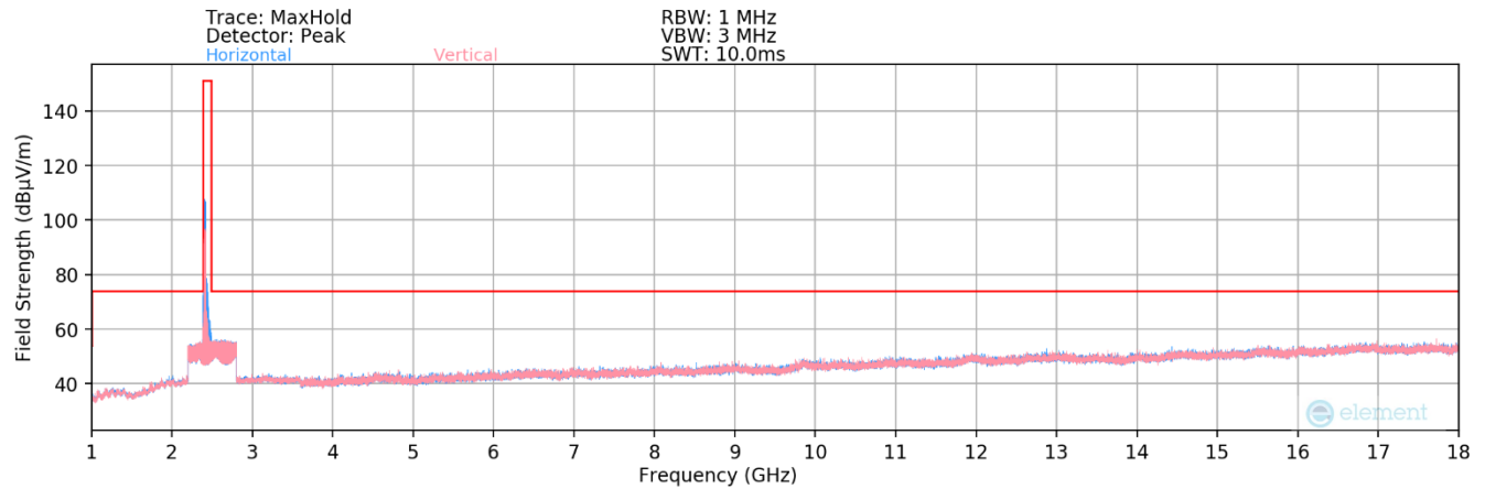
Plot 7-97. Radiated Spurious Plot above 1GHz SISO ANT2 (802.11ax OFDMA – 242 Tones – Ch. 1)
