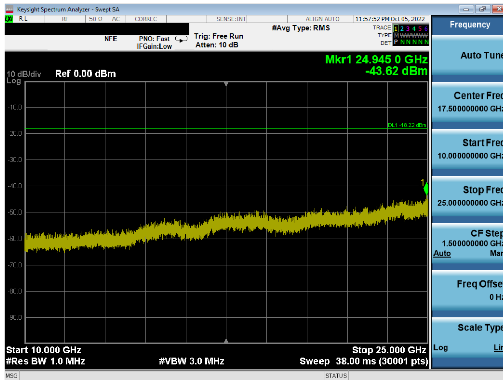
Plot 7-59. Conducted Spurious Plot SISO ANT2 (802.11ax OFDMA – 26 Tones – Ch. 1)
