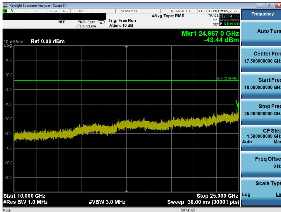
Plot 7-81. Conducted Spurious Plot MIMO ANT1 (802.11ax OFDMA – 242 Tones – Ch. 11)
