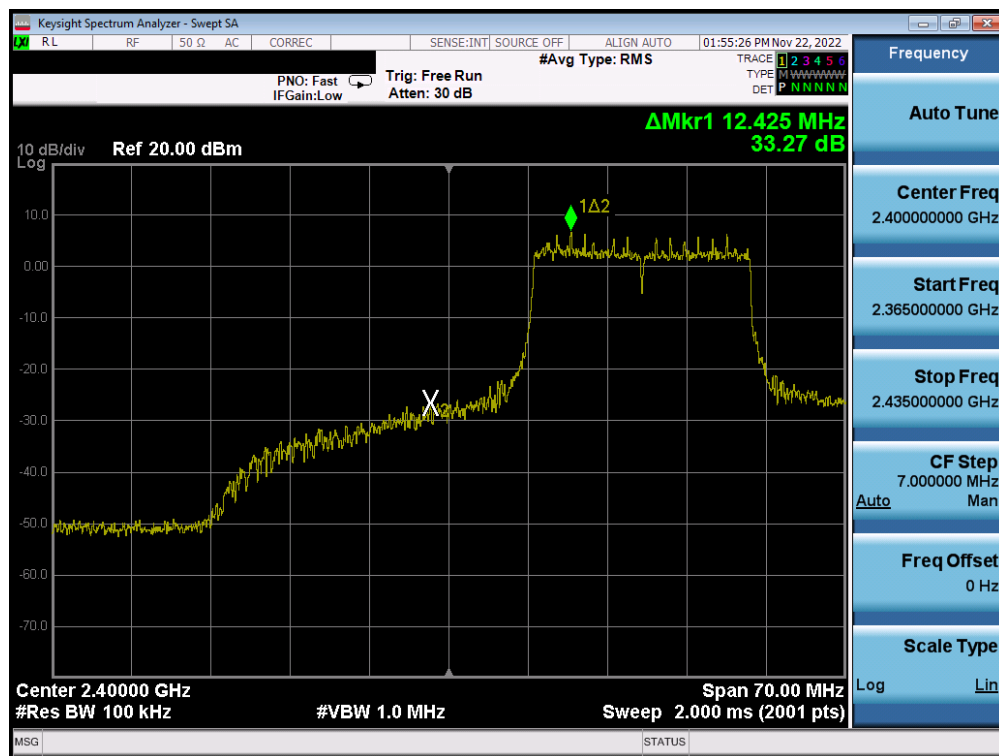
Plot 7-47. Band Edge Plot MIMO ANT1 (802.11ax OFDMA - 242 Tones - Ch. 2)
