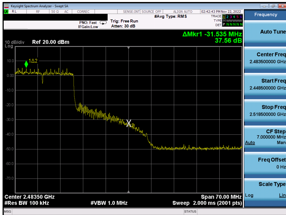
Plot 7-56. Band Edge Plot MIMO ANT2 (802.11ax OFDMA – 242 Tones – Ch. 10)
