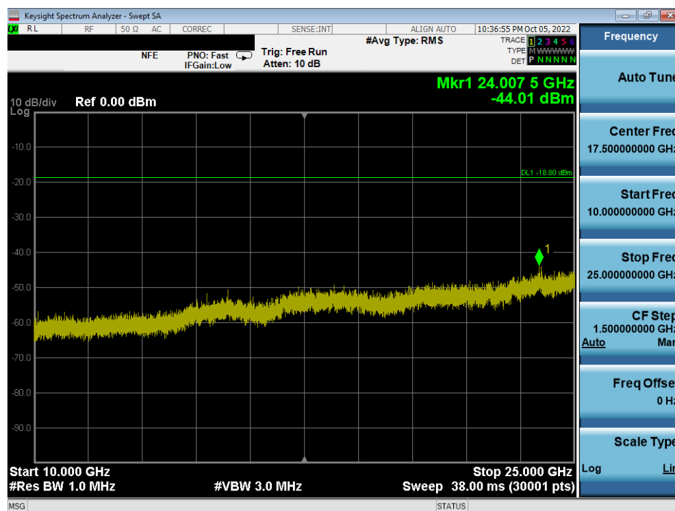
Plot 7-85. Conducted Spurious Plot MIMO ANT2 (802.11ax OFDMA – 26 Tones – Ch. 6)
