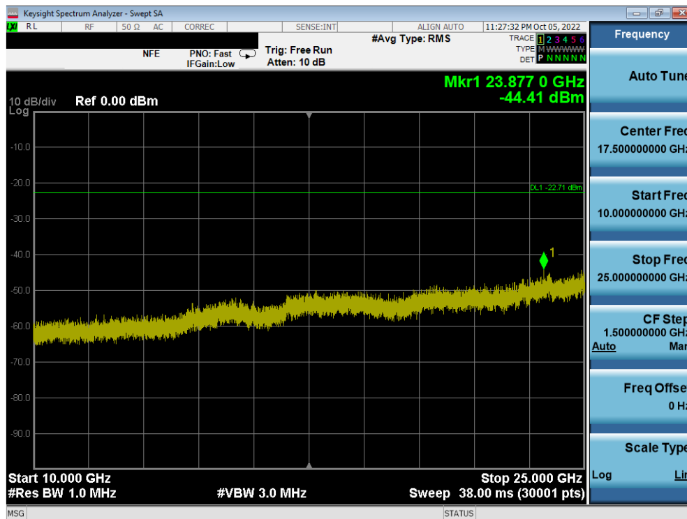
Plot 7-91. Conducted Spurious Plot MIMO ANT2 (802.11ax OFDMA – 242 Tones – Ch. 6)
