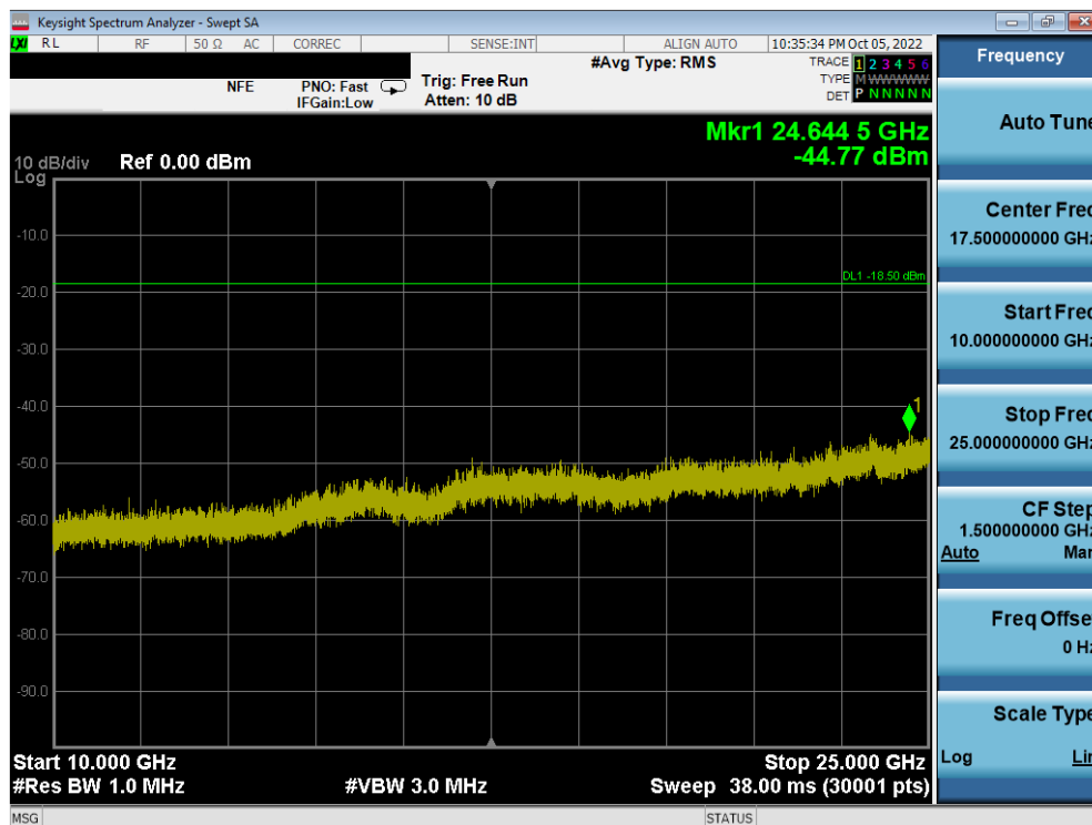
Plot 7-83. Conducted Spurious Plot MIMO ANT2 (802.11ax OFDMA – 26 Tones – Ch. 1)
