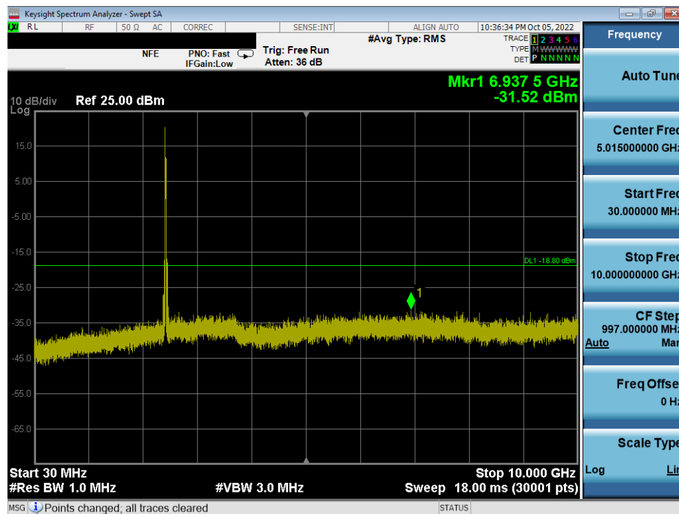
Plot 7-84. Conducted Spurious Plot MIMO ANT2 (802.11ax OFDMA – 26 Tones – Ch. 6)
