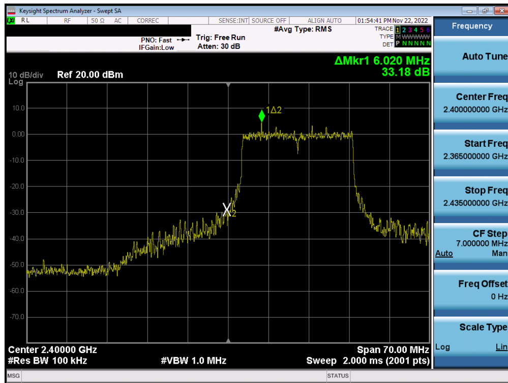
Plot 7-46. Band Edge Plot MIMO ANT1 (802.11ax OFDMA - 242 Tones - Ch. 1)
