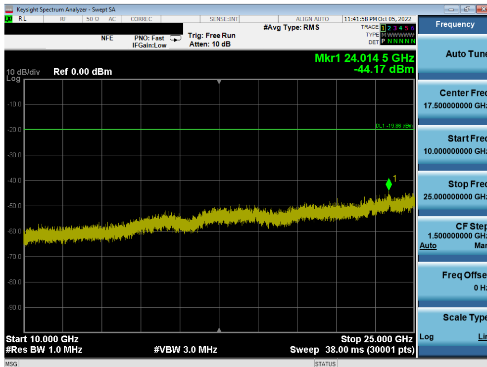
Plot 7-75. Conducted Spurious Plot MIMO ANT1 (802.11ax OFDMA – 26 Tones – Ch. 11)
