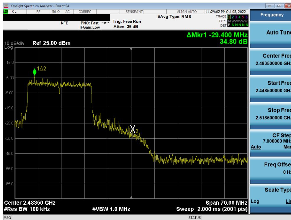
Plot 7-57. Band Edge Plot MIMO ANT2 (802.11ax OFDMA – 242 Tones – Ch. 11)
