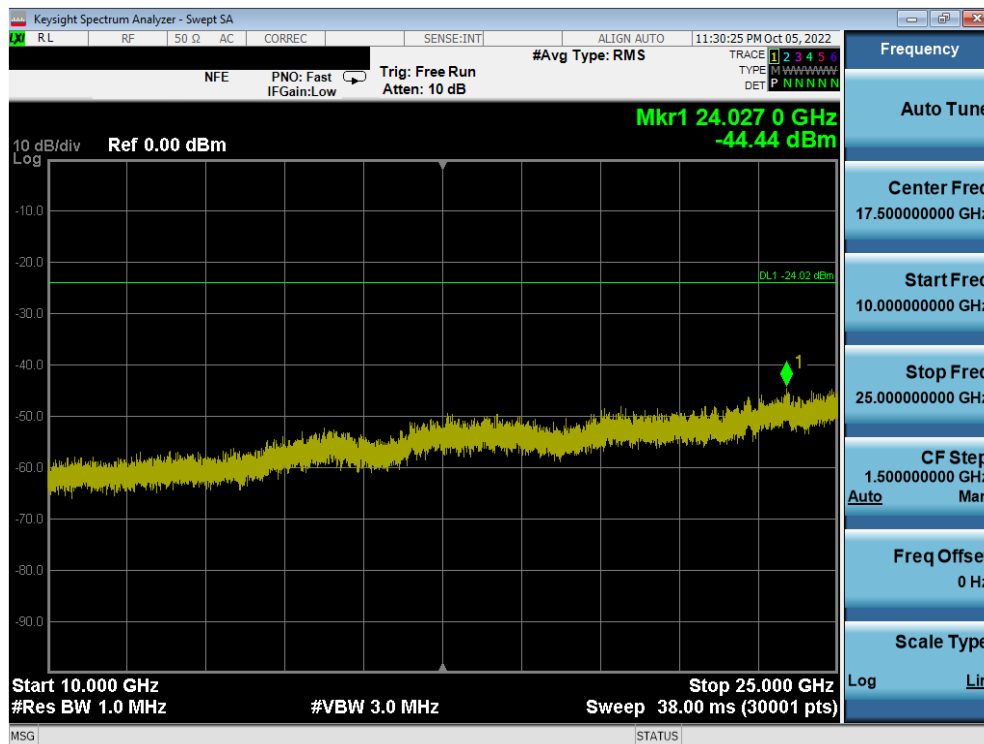
Plot 7-93. Conducted Spurious Plot MIMO ANT2 (802.11ax OFDMA – 242 Tones – Ch. 11)
