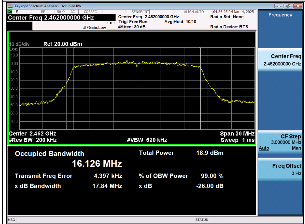
Test_Graph_802.11g_Chain A_2462_6Mbps_OBW
