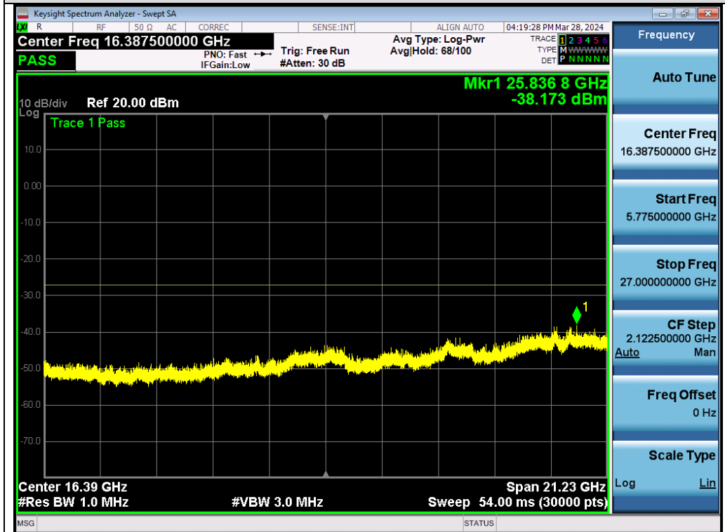
Test_Graph_802.11a_Chain B_5500_6Mbps_Frequency Band 4
