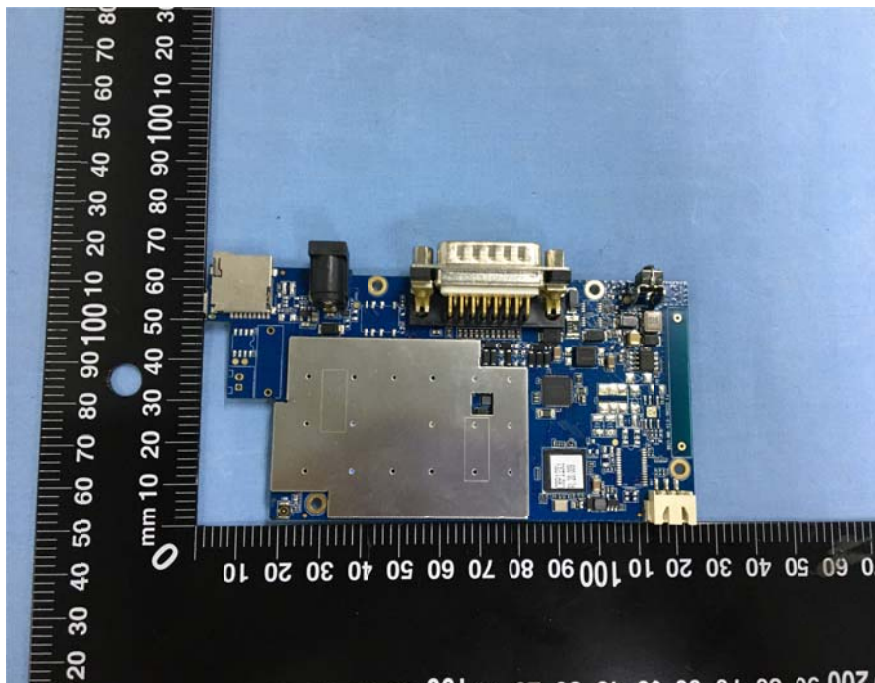
Solder Board-Component View (2)
