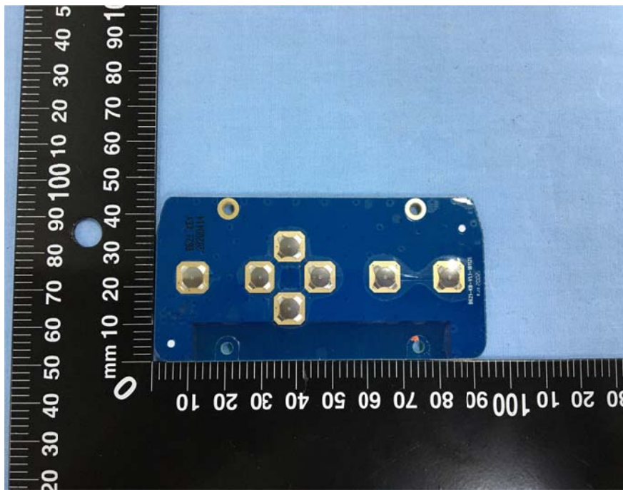
Solder Board-Component View (7)
