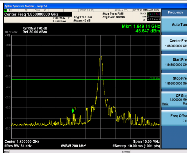
Band25-15MHz-16QAM-26115-1-0-Low--45.65-PASS
