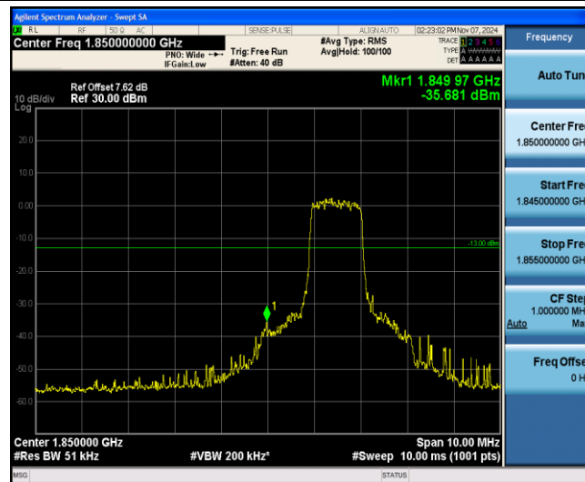
Band25-15MHz-16QAM-26115-6-0-Low--35.68-PASS
