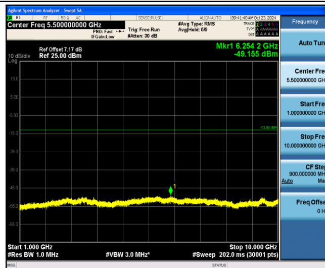
Band12-1.4MHz-QPSK-23173-1-0-Low-1000-10000--49.16-PASS
