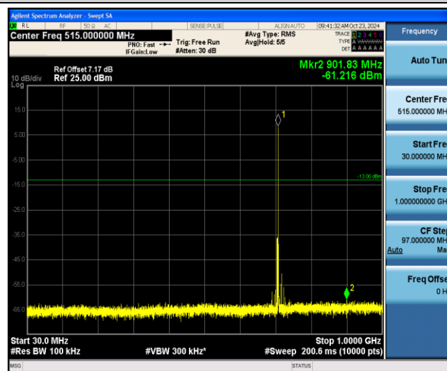
Band12-1.4MHz-QPSK-23173-1-0-Low-30-1000--61.22-PASS
