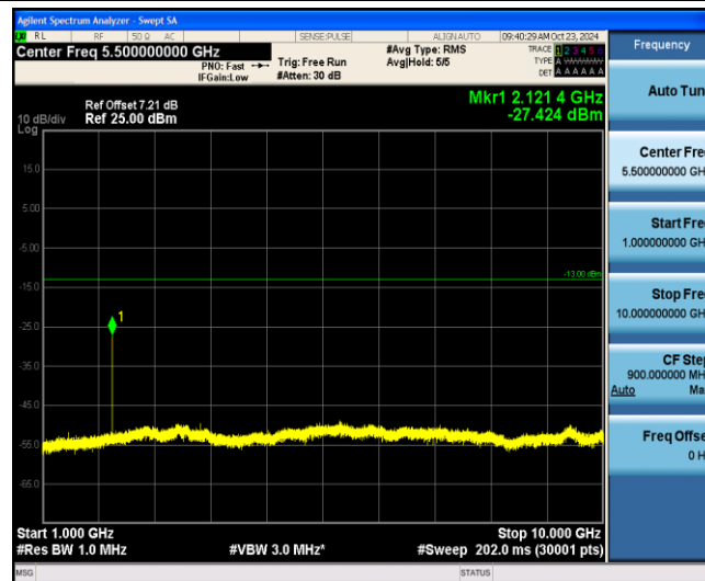
Band12-1.4MHz-QPSK-23095-1-0-Low-1000-10000--27.42-PASS
