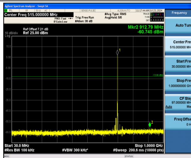
Band12-5MHz-16QAM-23095-1-0-Low-30-1000--60.75-PASS
