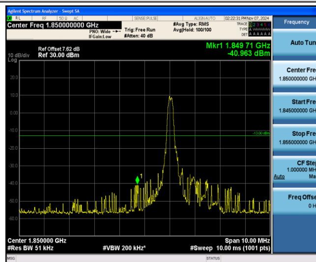
Band25-15MHz-QPSK-26115-1-0-Low--40.96-PASS
