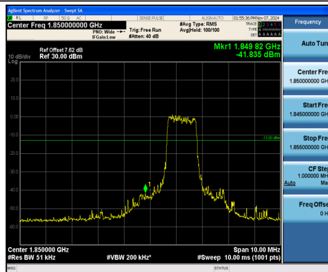
Band25-10MHz-16QAM-26090-6-0-Low--41.83-PASS
