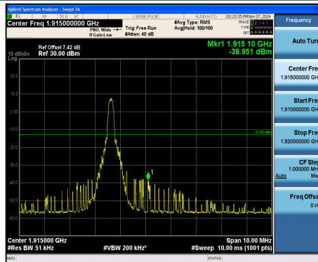
Band25-15MHz-QPSK-26615-1-5-High--38.95-PASS
