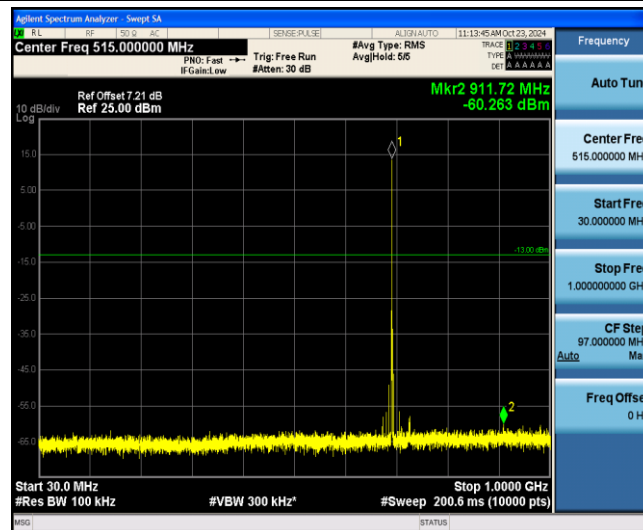
Band12-5MHz-16QAM-23035-1-0-Low-30-1000--60.26-PASS
