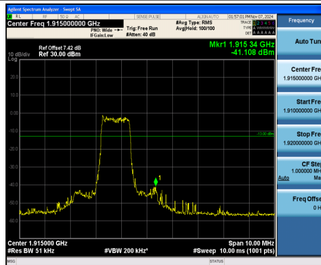
Band25-10MHz-16QAM-26640-6-0-High--41.11-PASS
