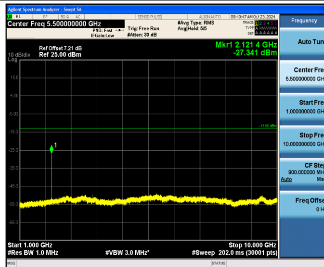
Band12-1.4MHz-16QAM-23095-1-0-Low-1000-10000--27.34-PASS
