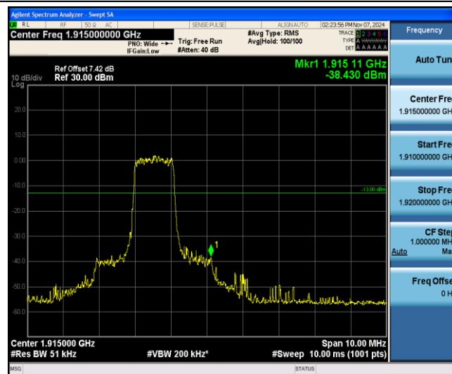
Band25-15MHz-QPSK-26615-6-0-High--38.43-PASS
