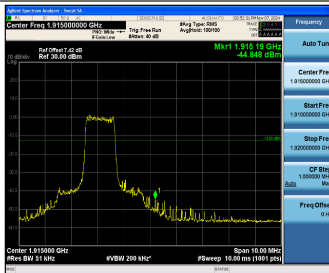
Band25-20MHz-16QAM-26590-6-0-High--44.85-PASS
