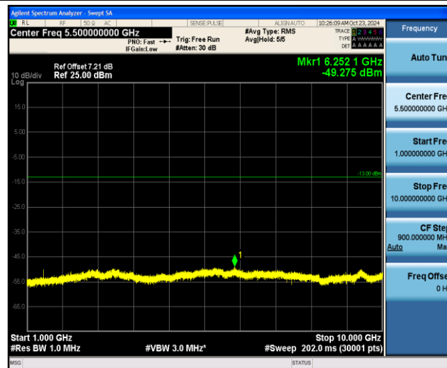
Band12-3MHz-16QAM-23095-1-0-Low-1000-10000--49.28-PASS
