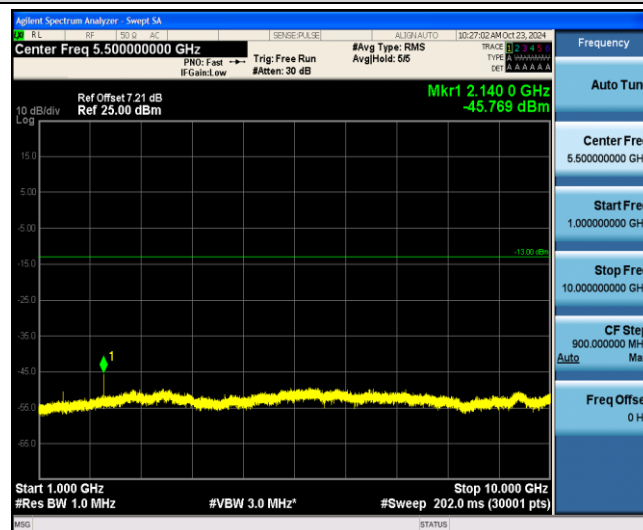
Band12-3MHz-QPSK-23165-1-0-Low-1000-10000--45.77-PASS
