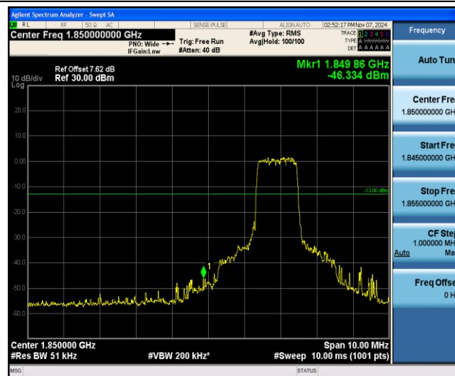
Band25-20MHz-QPSK-26140-6-0-Low--46.33-PASS
