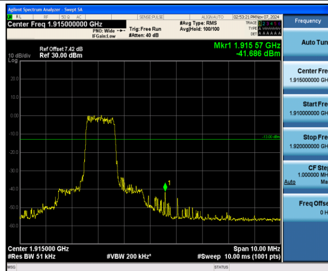
Band25-20MHz-QPSK-26590-6-0-High--41.69-PASS
