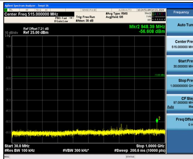
Band12-3MHz-16QAM-23025-1-0-Low-30-1000--56.61-PASS
