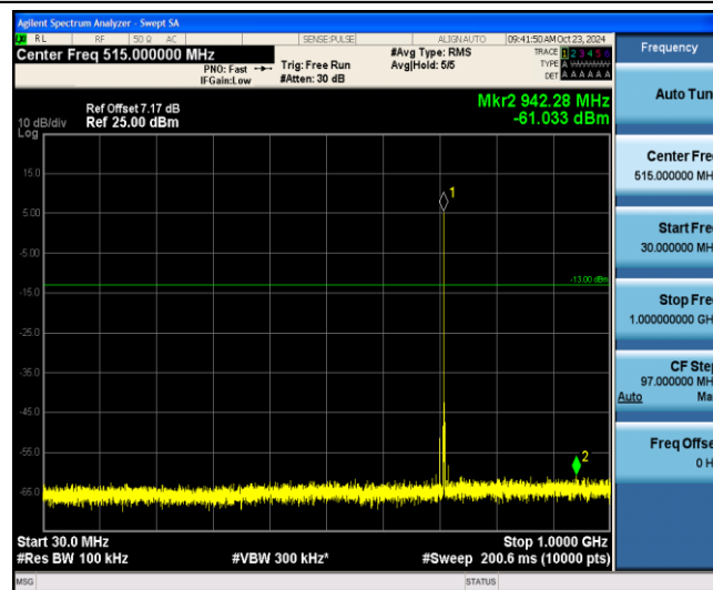
Band12-1.4MHz-16QAM-23173-1-0-Low-30-1000--61.03-PASS
