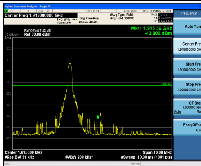
Band25-15MHz-16QAM-26615-1-5-High--43.80-PASS
