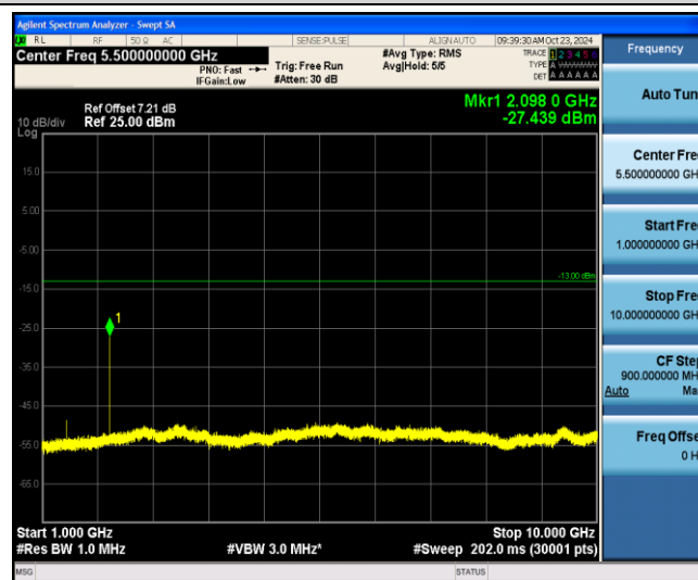
Band12-1.4MHz-16QAM-23017-1-0-Low-1000-10000--27.44-PASS
