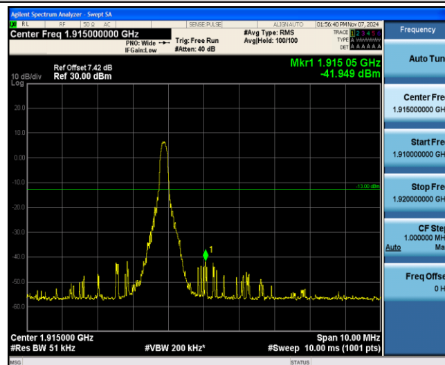
Band25-10MHz-16QAM-26640-1-5-High--41.95-PASS
