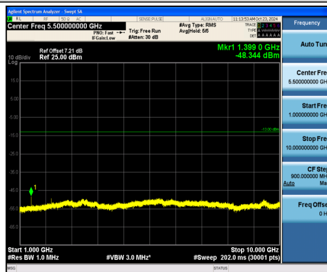
Band12-5MHz-16QAM-23035-1-0-Low-1000-10000--48.34-PASS
