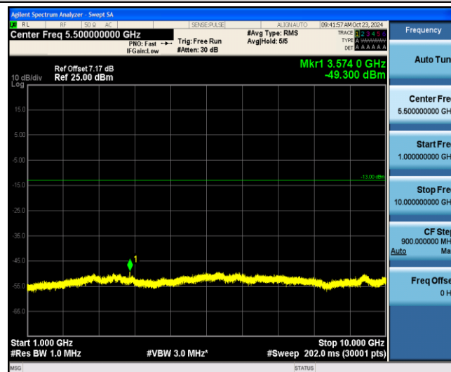
Band12-1.4MHz-16QAM-23173-1-0-Low-1000-10000--49.3-PASS
