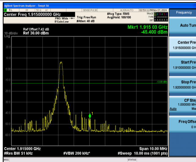
Band25-20MHz-16QAM-26590-1-5-High--45.40-PASS
