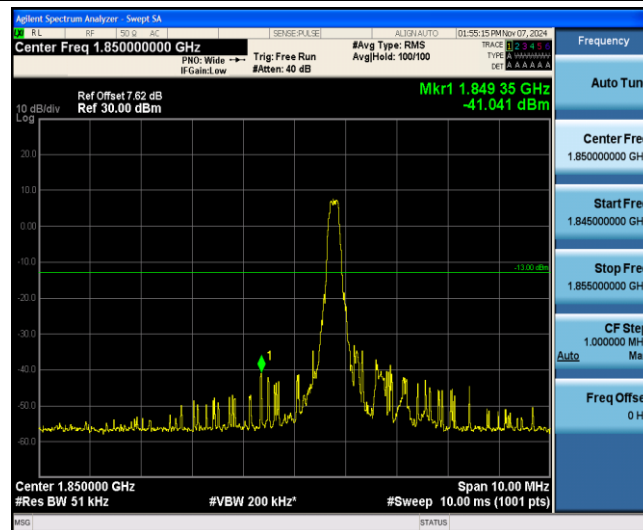
Band25-10MHz-16QAM-26090-1-0-Low--41.04-PASS
