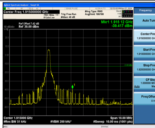
Band25-20MHz-QPSK-26590-1-5-High--39.42-PASS
