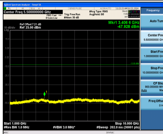
Band12-5MHz-QPSK-23155-1-0-Low-1000-10000--47.93-PASS
