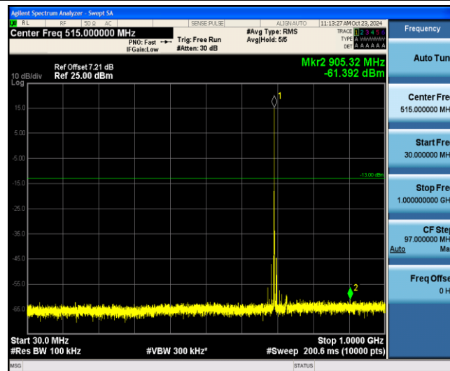
Band12-5MHz-QPSK-23035-1-0-Low-30-1000--61.39-PASS
