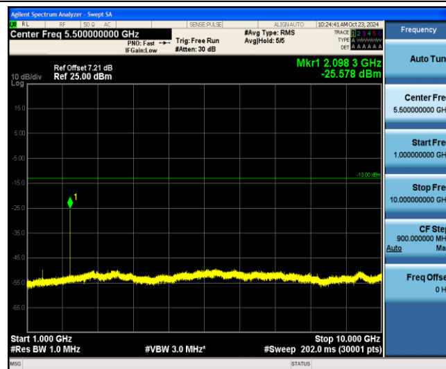
Band12-3MHz-QPSK-23025-1-0-Low-1000-10000--25.58-PASS
