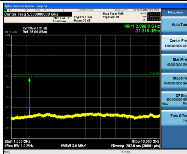
Band12-3MHz-16QAM-23025-1-0-Low-1000-10000--21.32-PASS
