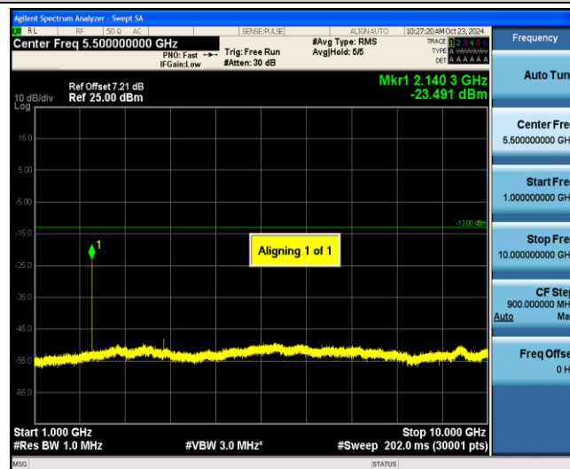
Band12-3MHz-16QAM-23165-1-0-Low-1000-10000--23.49-PASS
