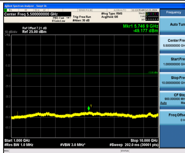
Band12-5MHz-QPSK-23035-1-0-Low-1000-10000--49.18-PASS
