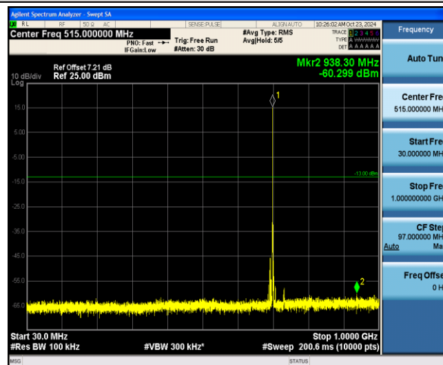
Band12-3MHz-16QAM-23095-1-0-Low-30-1000--60.3-PASS
