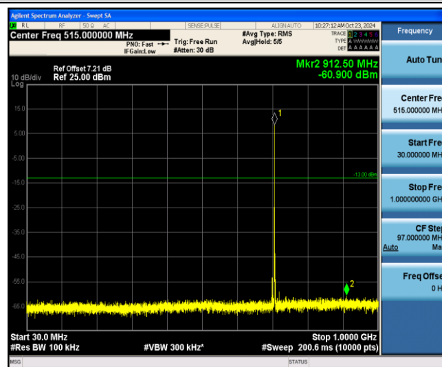
Band12-3MHz-16QAM-23165-1-0-Low-30-1000--60.9-PASS
