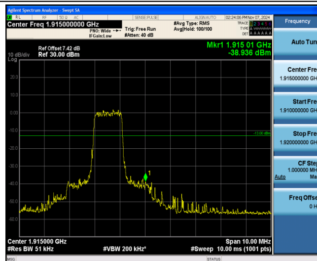
Band25-15MHz-16QAM-26615-6-0-High--38.94-PASS
