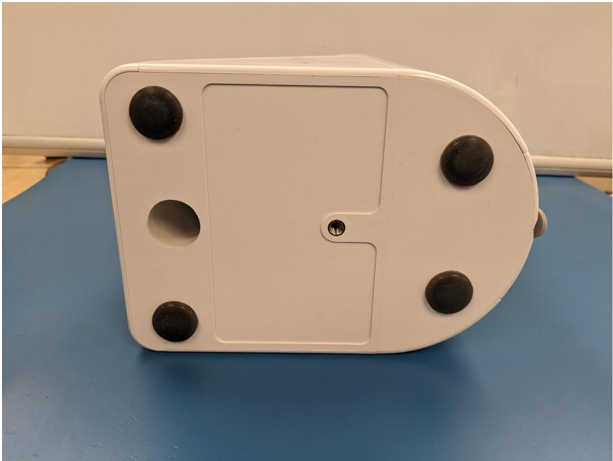
Figure 4: Underside, showing feet, exhaust port, label location, and tripod mounting point
