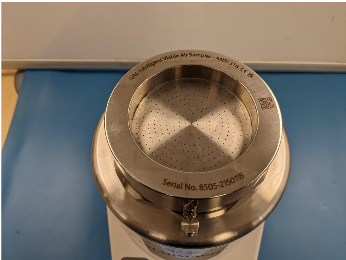
Figure 8: Top view, with sieve head fitted
