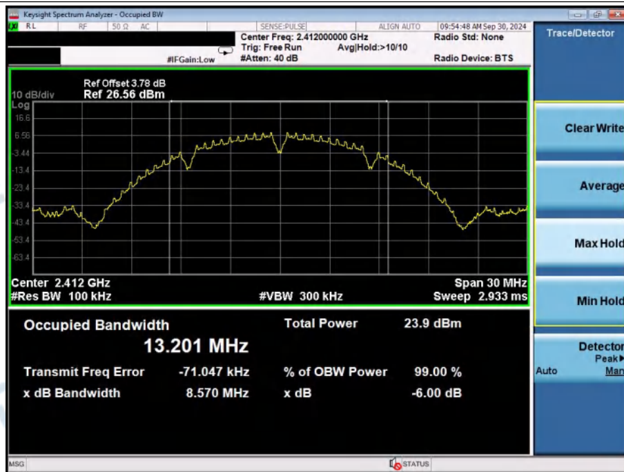
-6dB_Bandwidth_NVNT_ANT1_802_11b_2412
