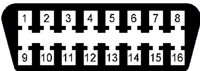
Connector on Vehicle side
