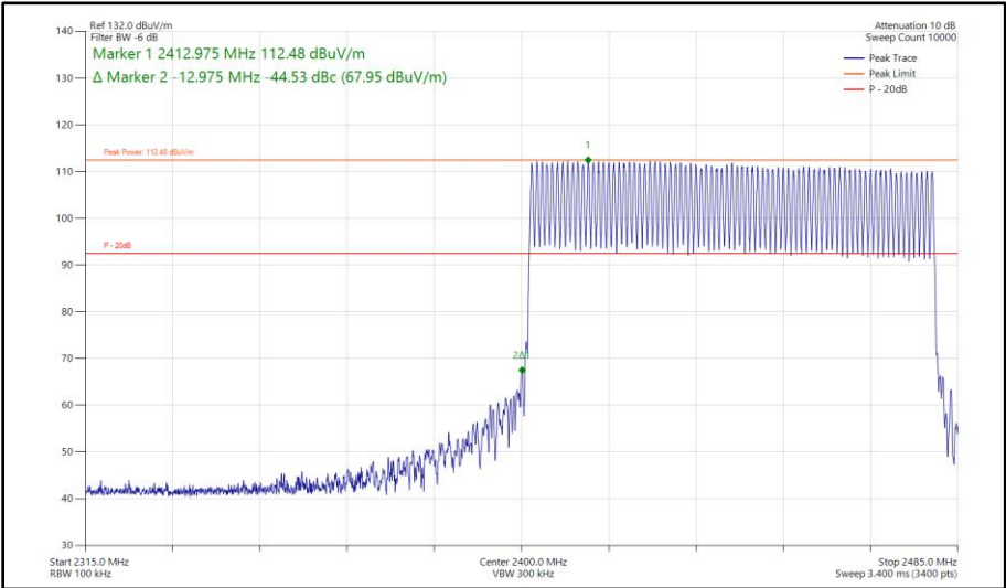
Figure 236 - Bluetooth 3-DH5, MIMO, Core 0 - Core 1 - Hopping Band Edge Frequency 2400 MHz
