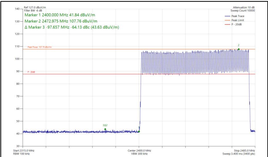
Figure 228 - Bluetooth DH5, SISO, Core 2 - Hopping Band Edge Frequency 2400 MHz
