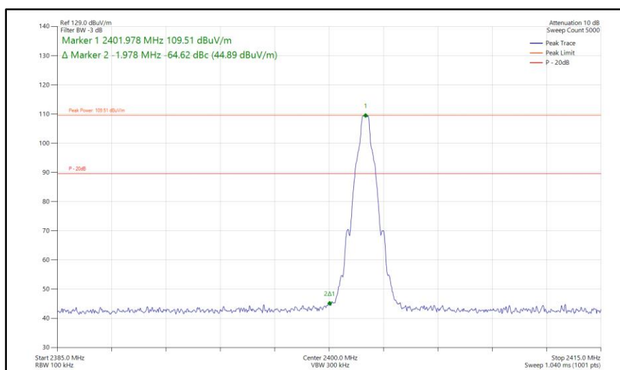
Figure 213 - Bluetooth DH5, SISO, Core 0 - 2402 MHz Band Edge Frequency 2400 MHz
