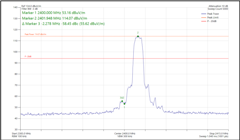
Figure 239 - Bluetooth 3-DH5, SISO, Core 0 - 2402 MHz Band Edge Frequency 2400 MHz
