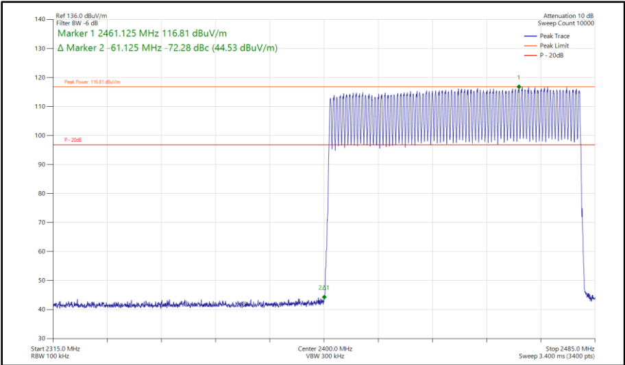
Figure 240 - Bluetooth DH5, SISO, Core 0 - Hopping Band Edge Frequency 2400 MHz
