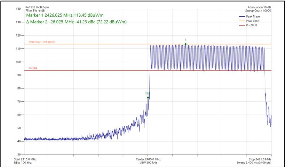
Figure 235 - Bluetooth 2-DH5, MIMO, Core 0 - Core 1 - Hopping Band Edge Frequency 2400 MHz
