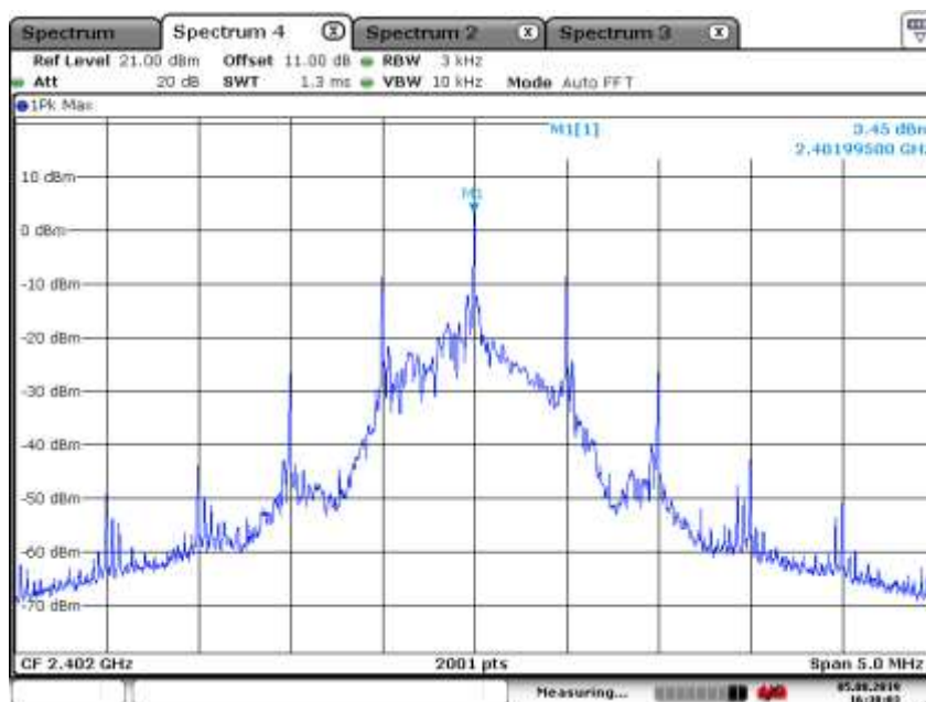
Mode 1 CH00(2402MHz)
