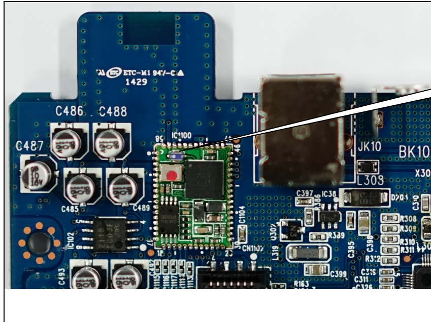
Chip Antenna
