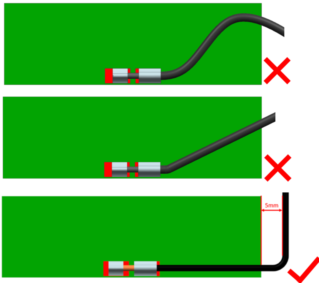
FIGURE 5.2 CABLE BENDING
