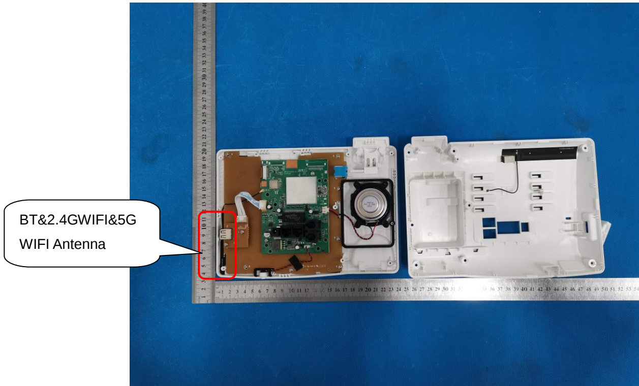
OPEN VIEW OF EUT(FIGURE 3)
