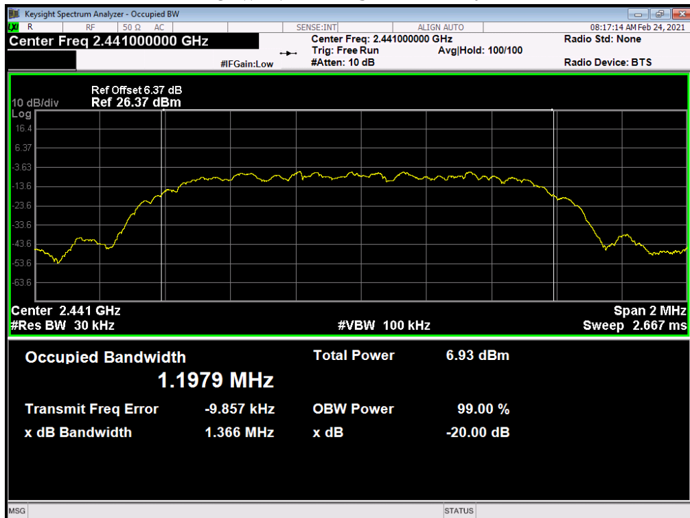
OBW NVNT 2-DH3 2441MHz Ant1
