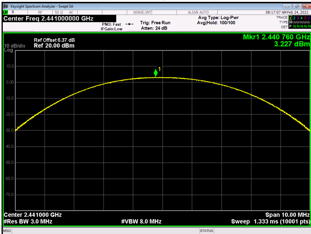
Power NVNT 2-DH3 2441MHz Ant1
