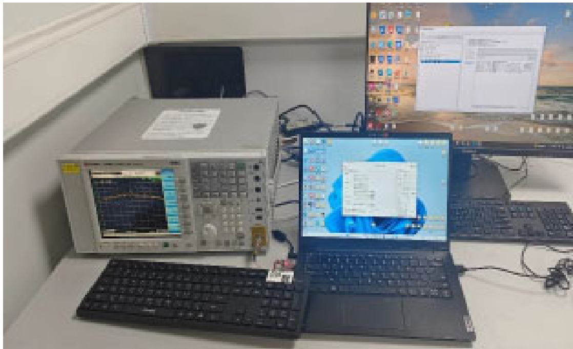
Conducted Test
