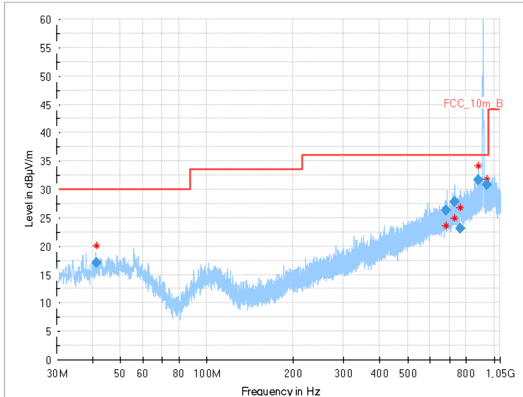
Plot 3: 30 MHz – 1 GHz, horizontal &amp; vertical polarisation (high channel)
