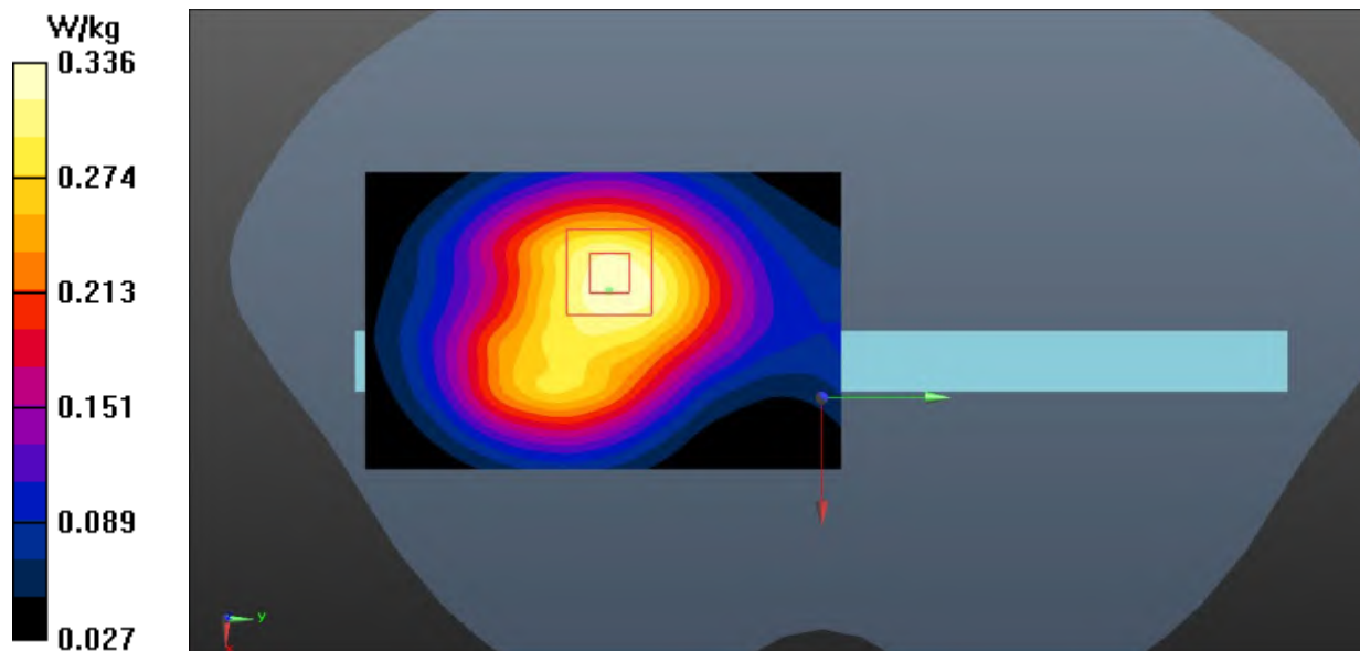
Fig.15 LTE Band 13 Body
