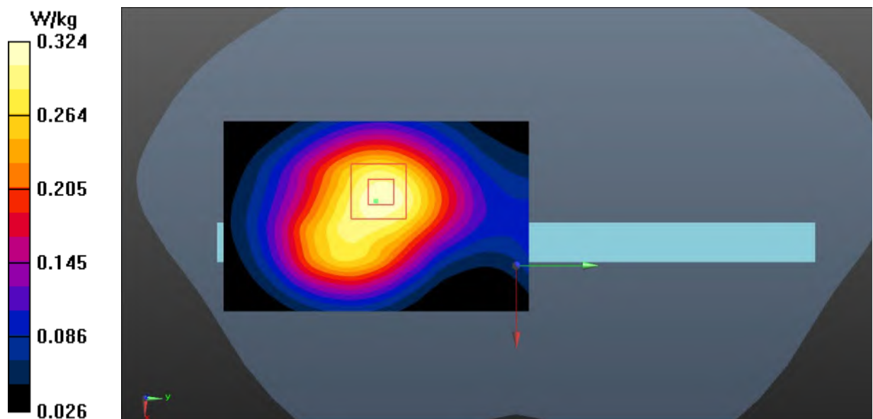
Fig.17 LTE Band 14 Body
