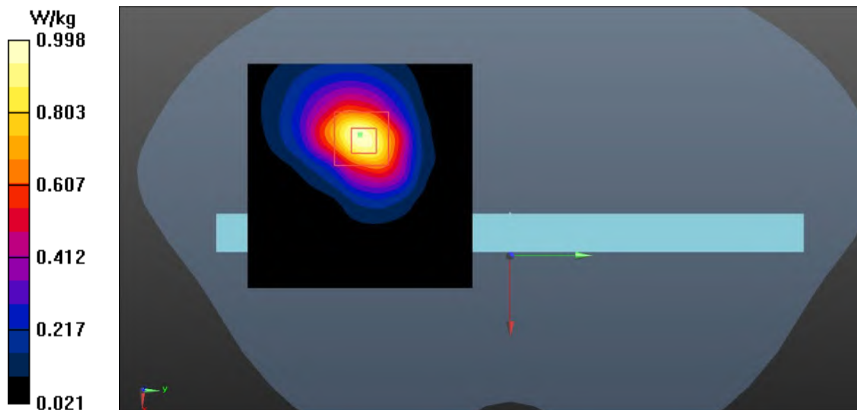
Fig.5 WCDMA Band 2 Body
