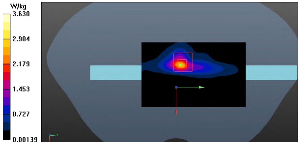
Fig.35 WLAN 5GHz Extremity
