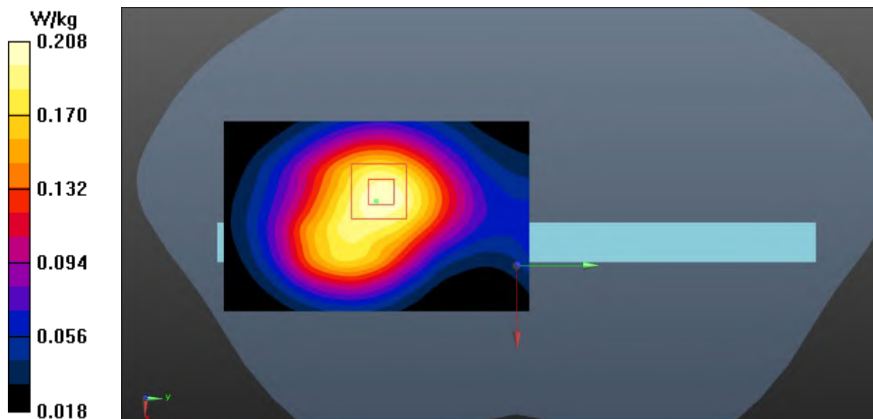
Fig.29 LTE Band 71 Body
