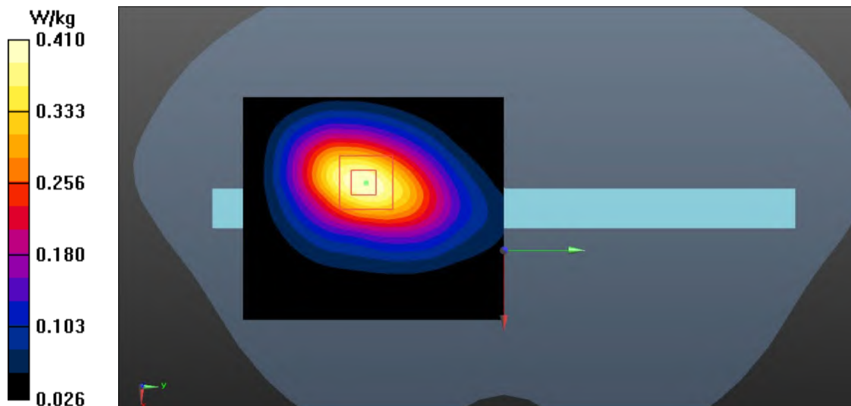
Fig.9 WCDMA Band 5 Body
