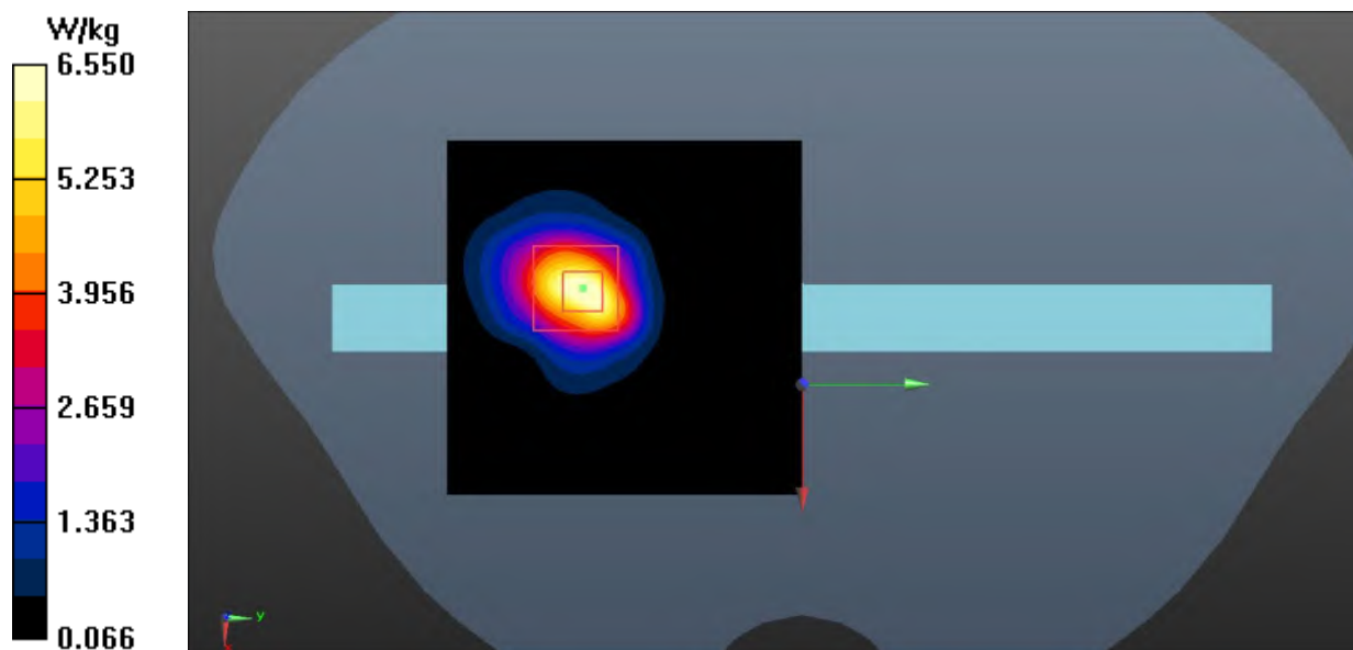
Fig.20 LTE Band 25 Extremity
