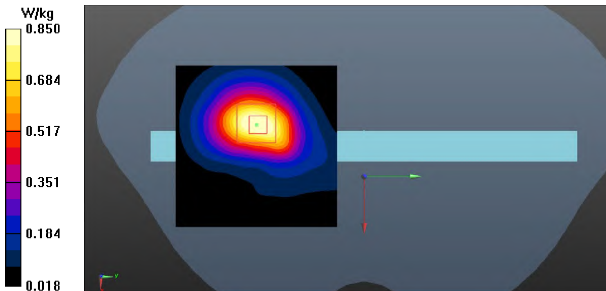
Fig.23 LTE Band 30 Body
