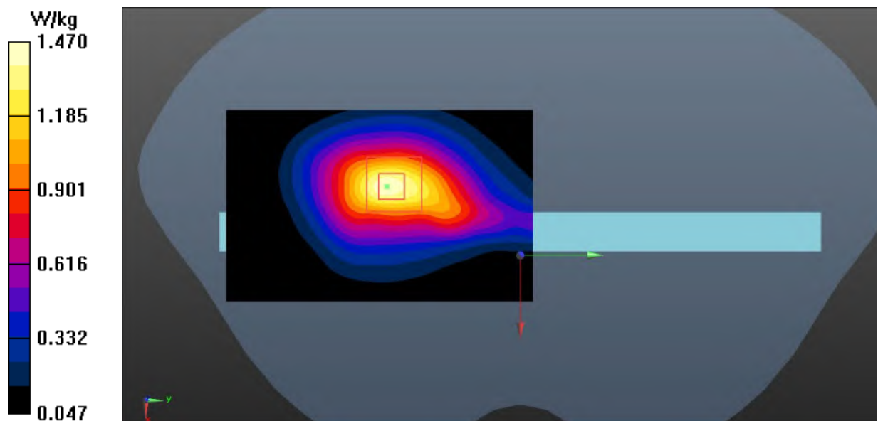
Fig.16 LTE Band 13 Extremity
