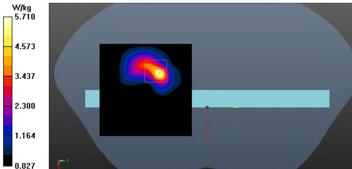
Fig.26 LTE Band 41 Extremity
