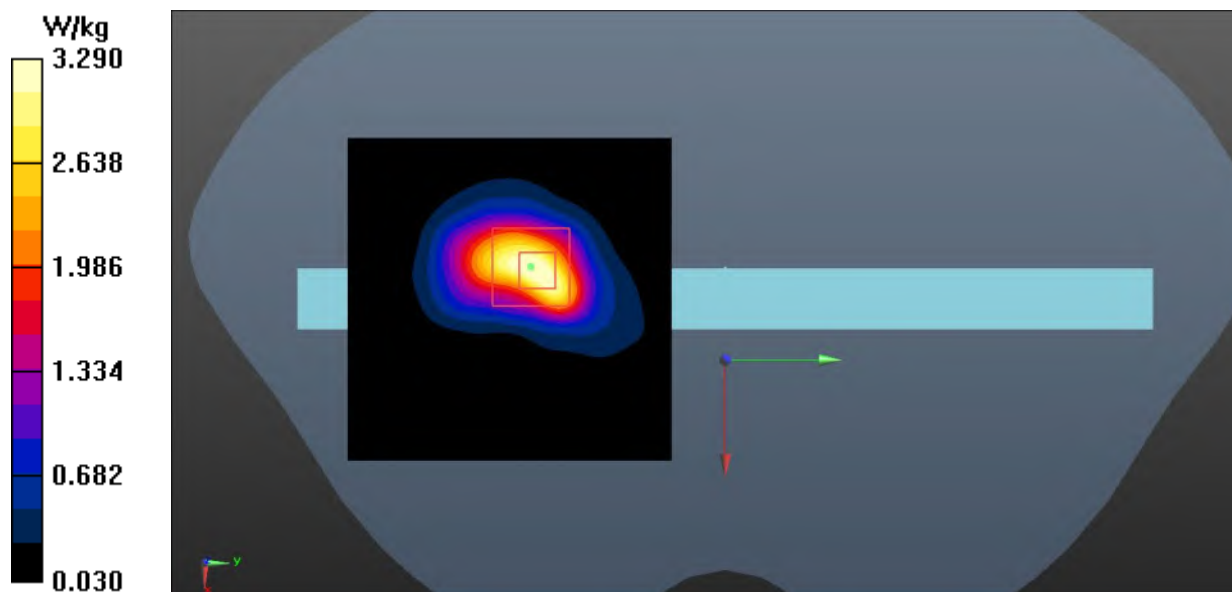
Fig.24 LTE Band 30 Extremity
