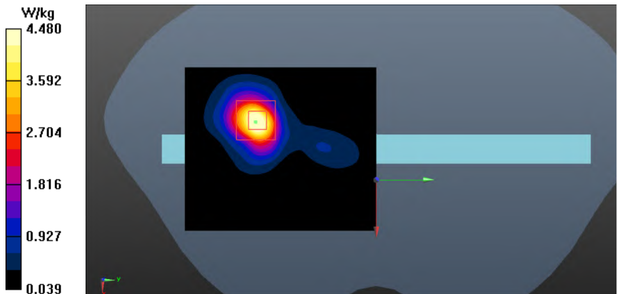
Fig.8 WCDMA Band 4 Extremity
