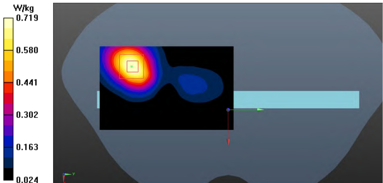
Fig.7 WCDMA Band 4 Body
