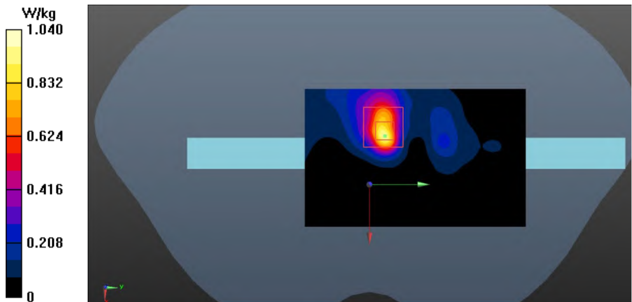
Fig.34 WLAN 5GHz Body
