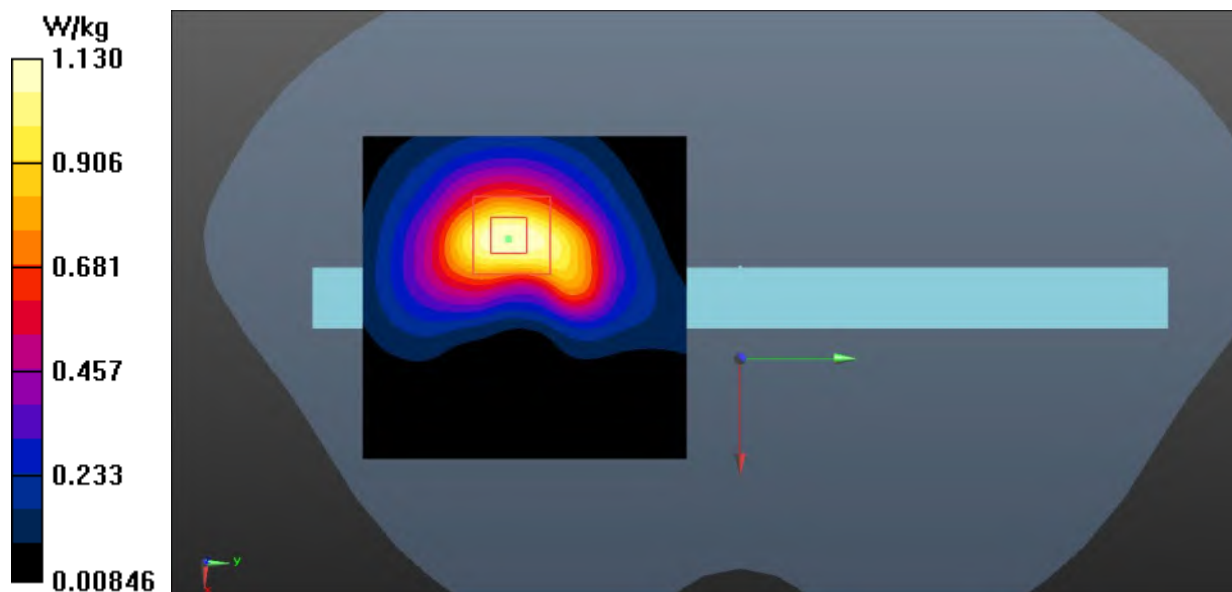
Fig.11 LTE Band 7 Body
