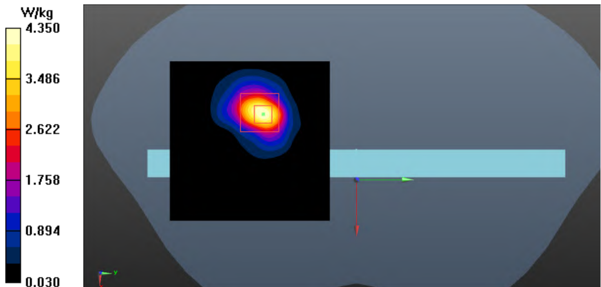
Fig.6 WCDMA Band 2 Extremity
