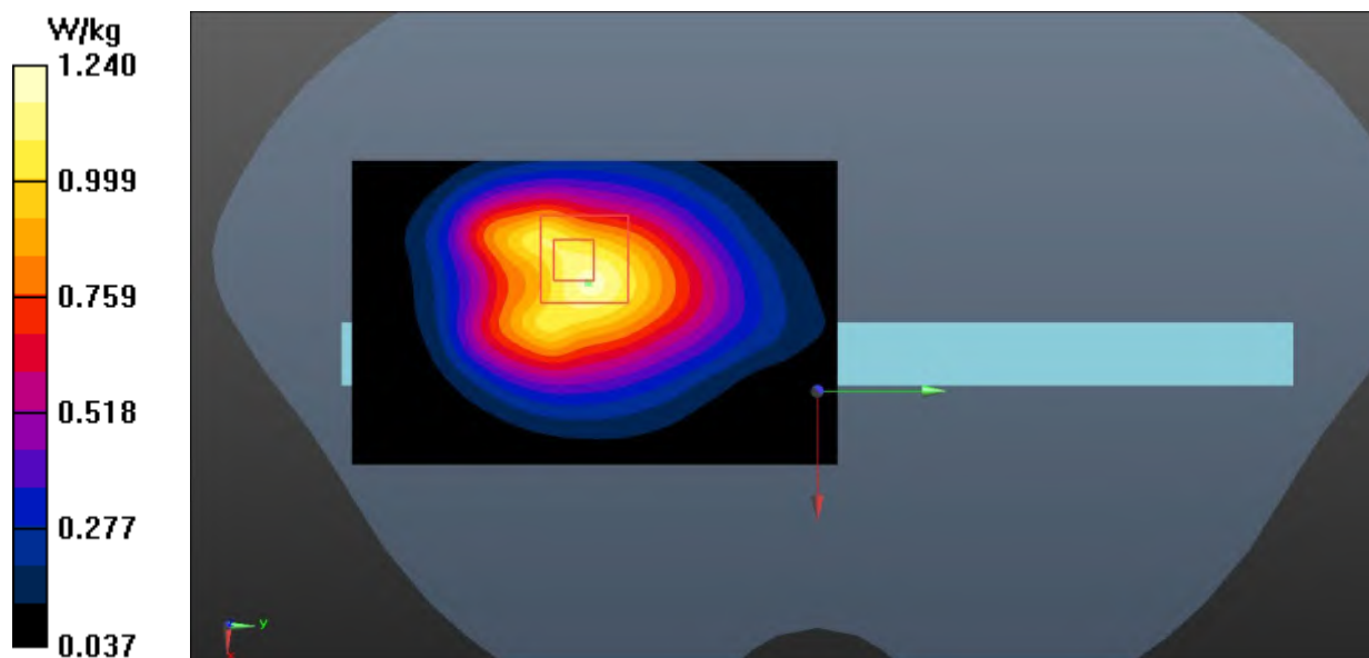
Fig.14 LTE Band 12 Extremity
