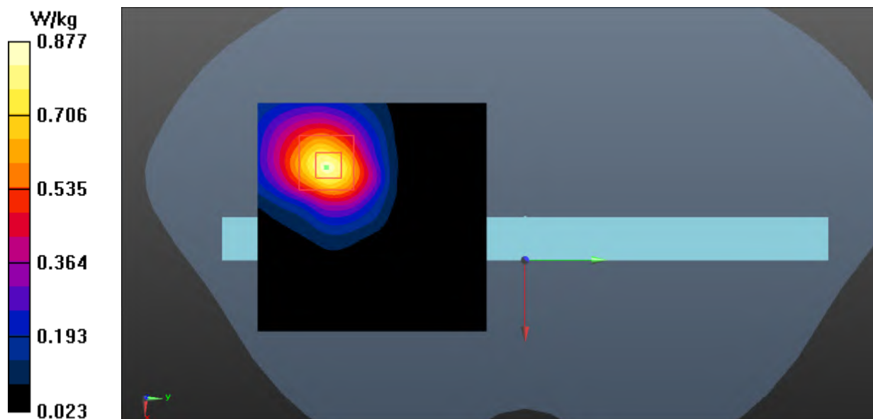
Fig.19 LTE Band 25 Body
