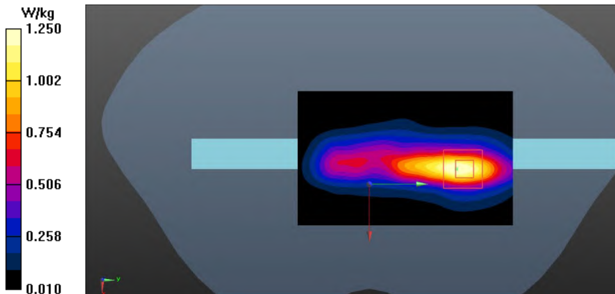
Fig.33 WLAN 2.4GHz Extremity
