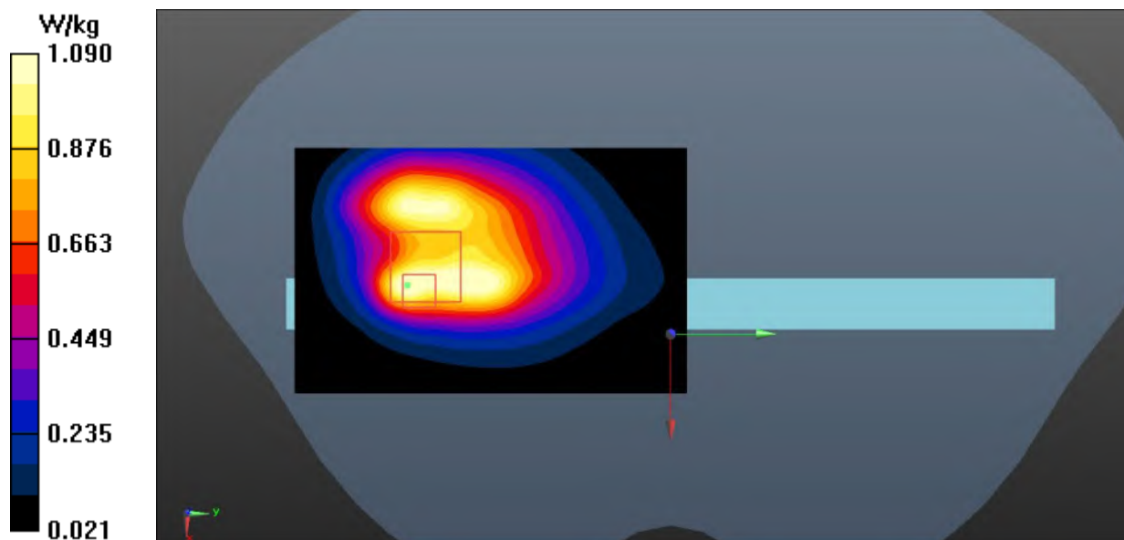
Fig.30 LTE Band 71 Extremity
