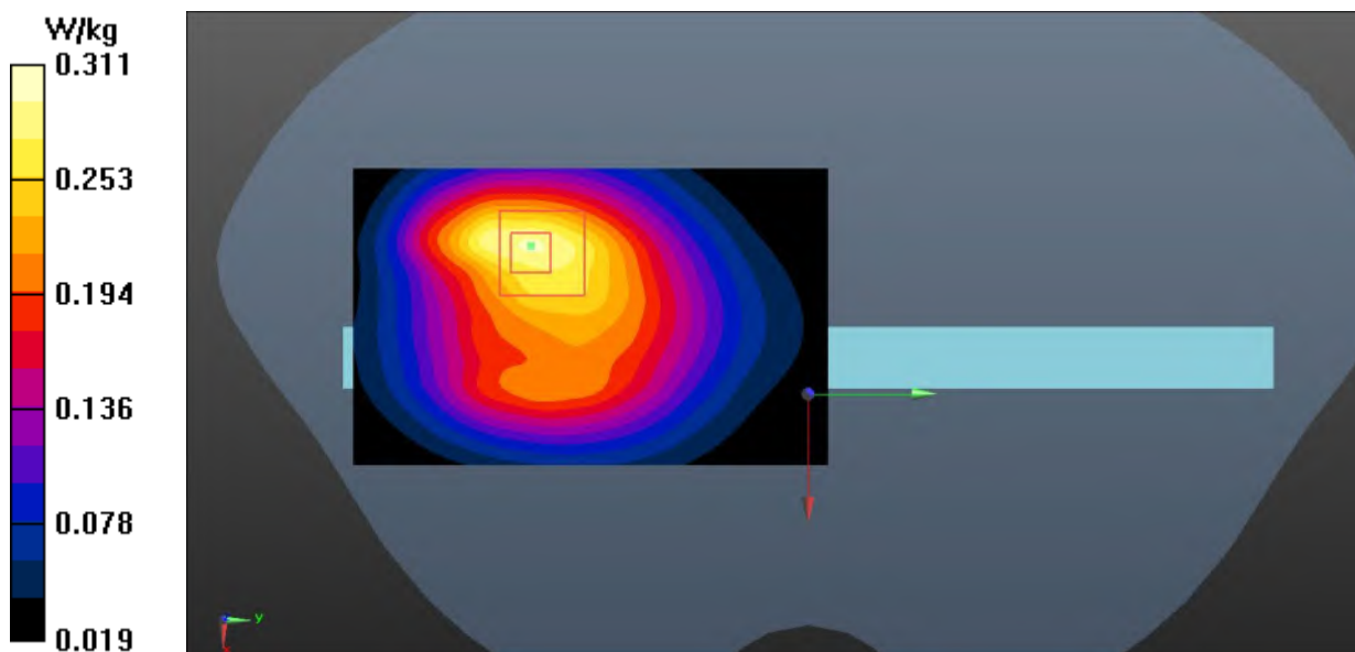
Fig.13 LTE Band 12 Body
