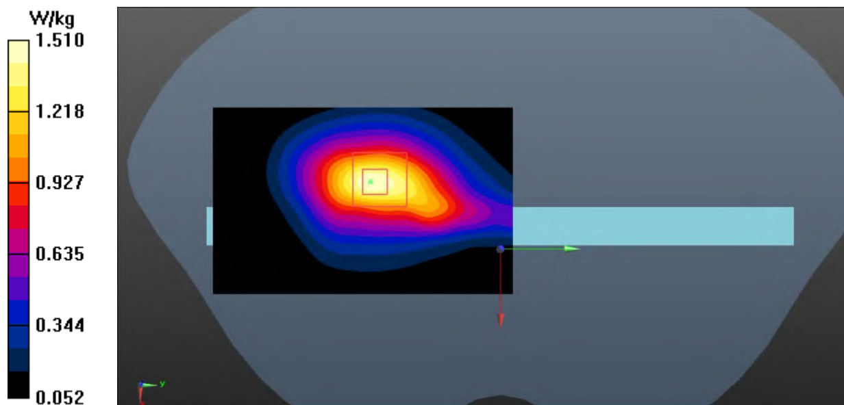
Fig.18 LTE Band 14 Extremity
