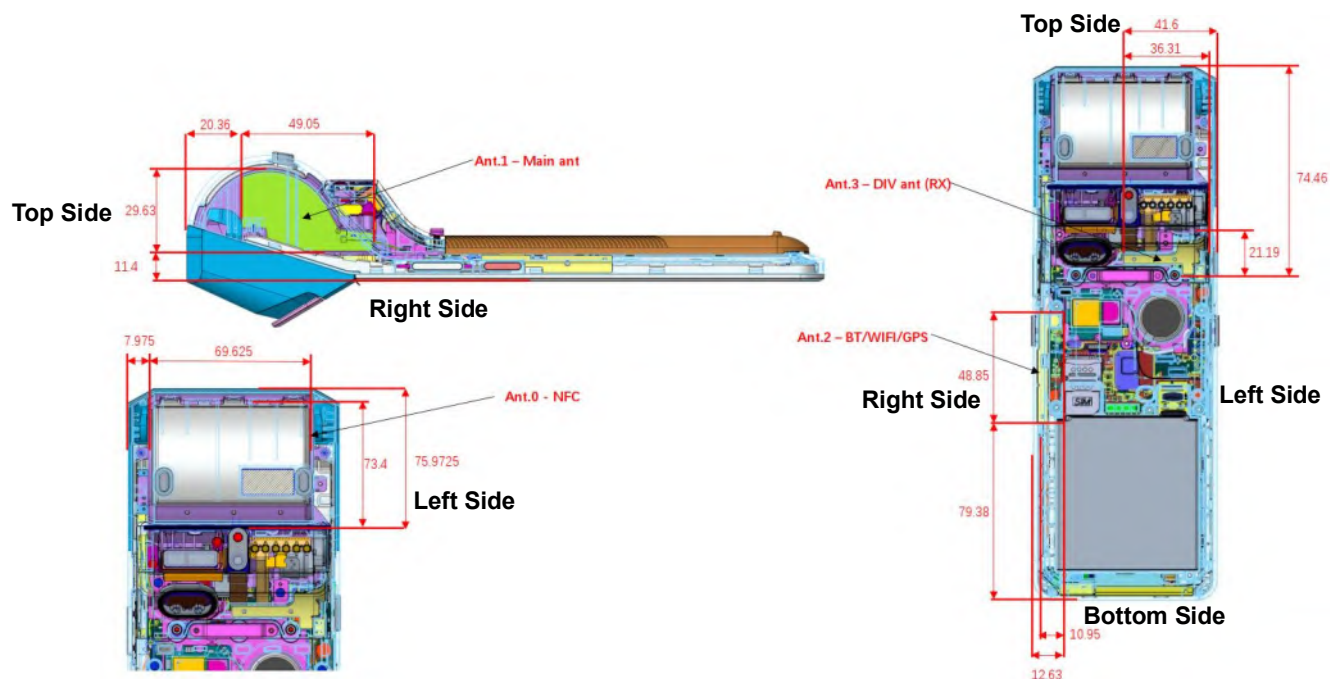
Picture 11.1 Antenna Locations (Back View)
