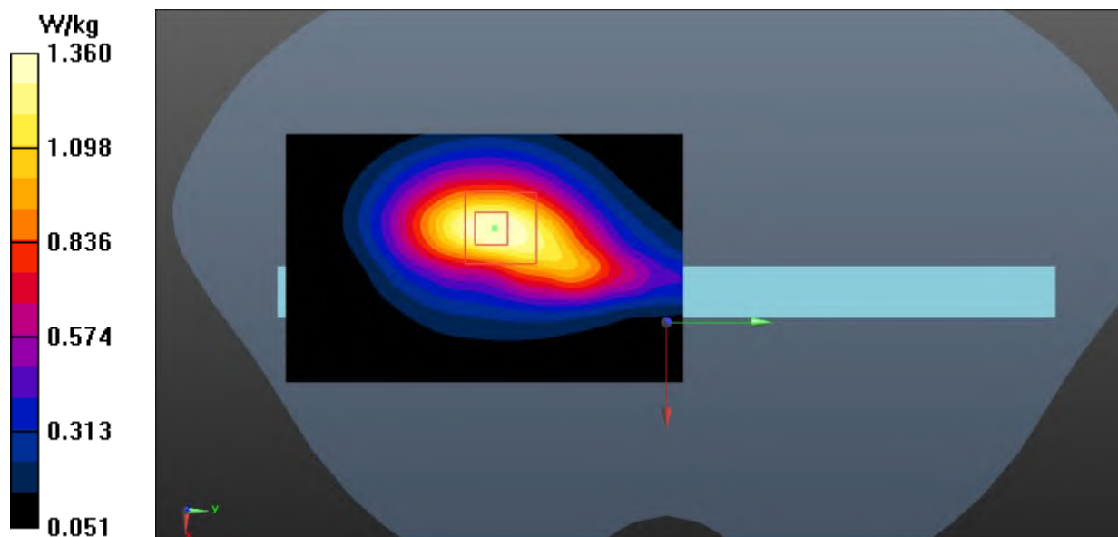
Fig.22 LTE Band 26 Extremity
