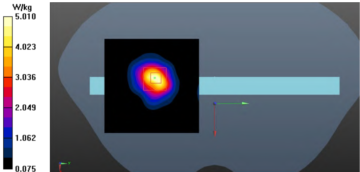
Fig.28 LTE Band 66 Extremity
