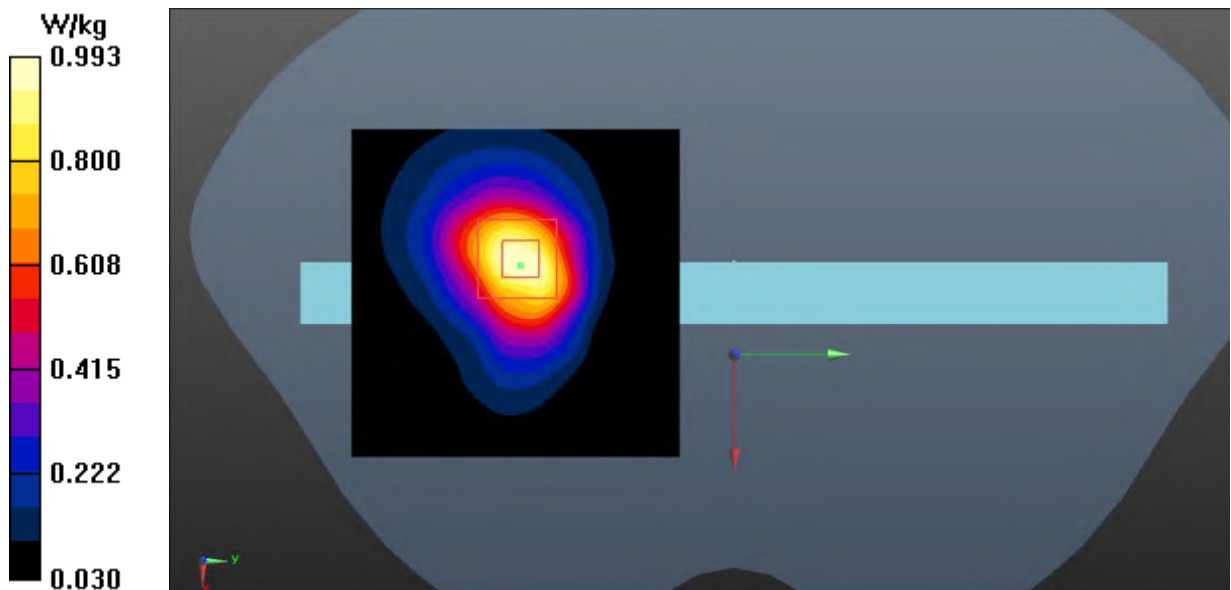
Fig.27 LTE Band 66 Body
