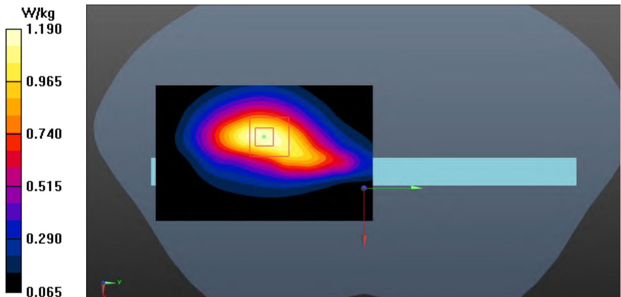
Fig.10 WCDMA Band 5 Extremity
